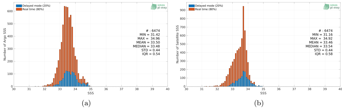
Figure 2: Histograms of SSS from Argo (a) and SMOS SSS L3 v8 - 18 Days (CATDS-CECOS-LOCEAN) (b) considering all match-up pairs per bins of 0.1 over the South China Sea Pi-MEP region and for the full satellite product period.
