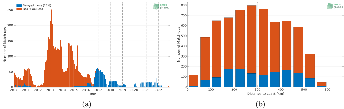
Figure 1: Number of match-ups between Argo and SMOS SSS L3 v8 - 18 Days (CATDS-CECOS-LOCEAN) SSS as a function of time (a) and as function of the distance to coast (b) over the South China Sea Pi-MEP region and for the full satellite product period.
