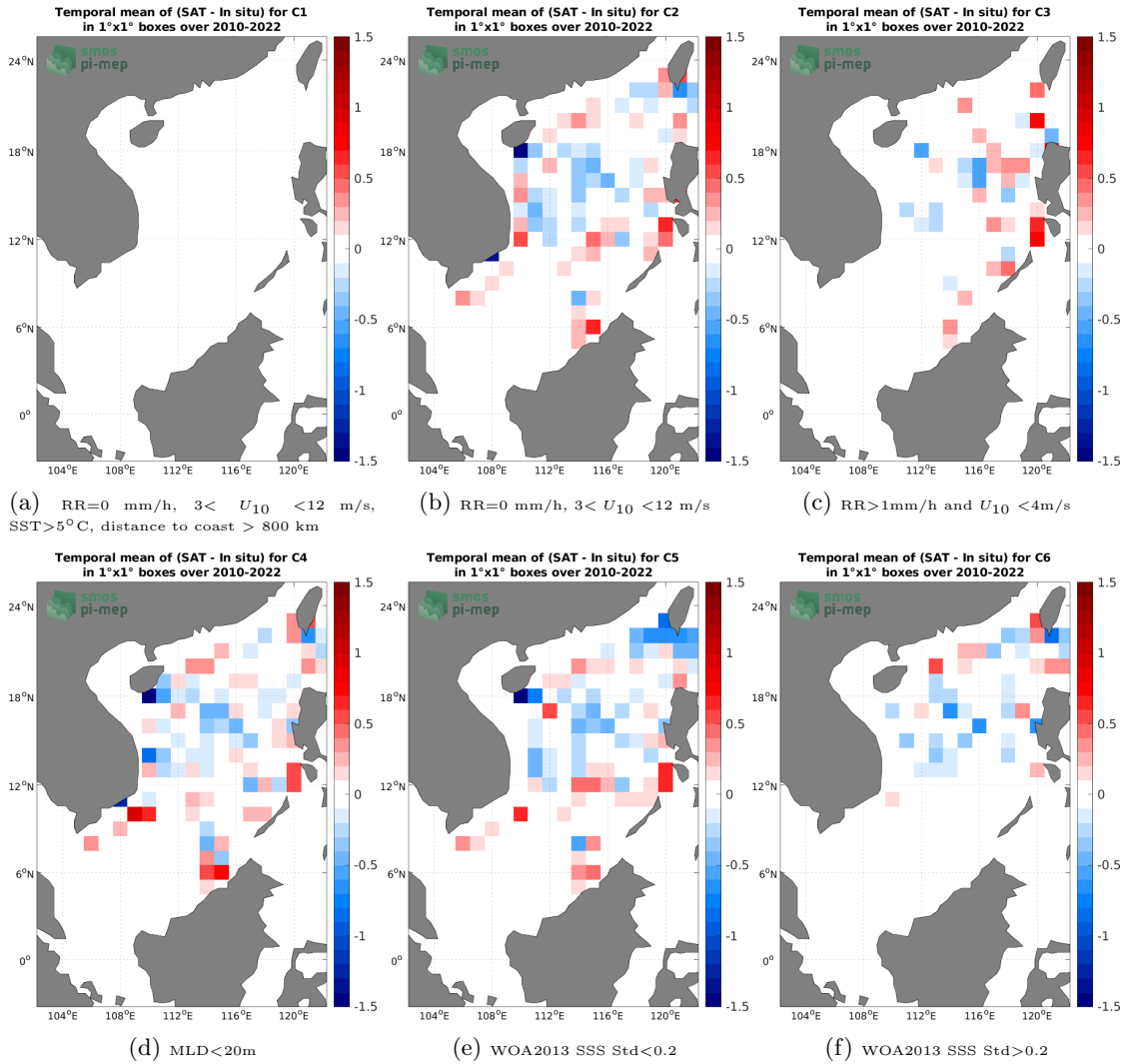
Figure 12: Temporal mean gridded over spatial boxes of size 1^\circ \times 1^\circ of \Delta SSS (SMOS SSS L3 v8 - 18 Days (CATDS-CECOS-LOCEAN) - Argo) for 6 different subdatasets corresponding to: RR=0 mm/h, 3 < U_{10} < 12 m/s, SST > 5^\circ\text{C} , distance to coast > 800 km (a), RR=0 mm/h, 3 < U_{10} < 12 m/s (b), RR > 1 mm/h and U_{10} < 4 m/s (c), MLD < 20 m (d), WOA2013 SSS Std < 0.2 (e), WOA2013 SSS Std > 0.2 (f).
