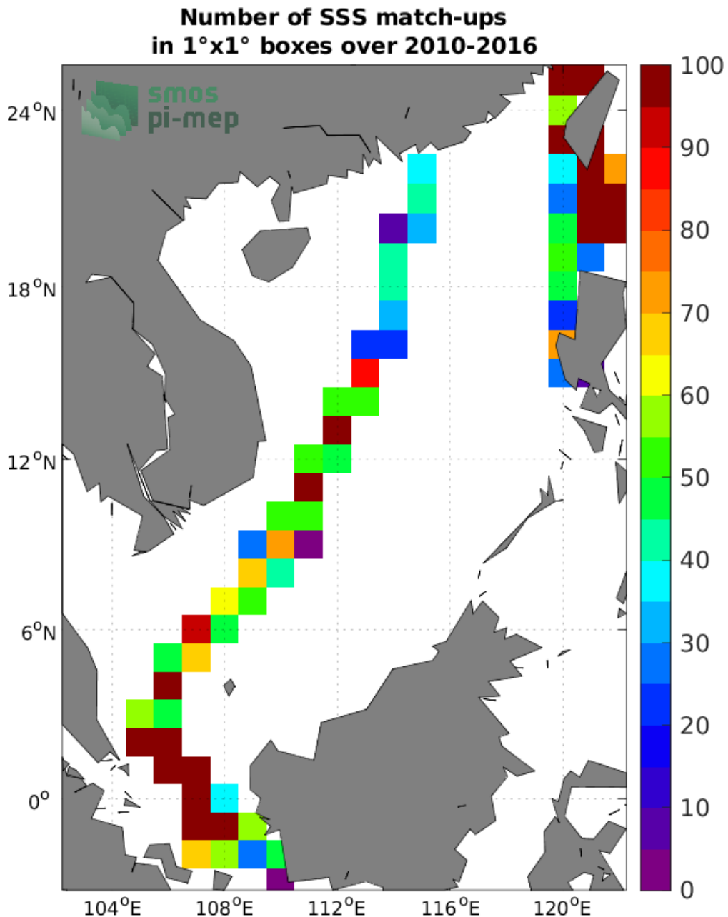
Figure 4: Number of SSS match-ups between TSG (LEGOS-DM) SSS and the SMOS SSS L3 v7 - 9 Days (CATDS-CECOS-LOCEAN) SSS product for the South China Sea Pi-MEP region over 1°×1° boxes and for the full satellite product period.
