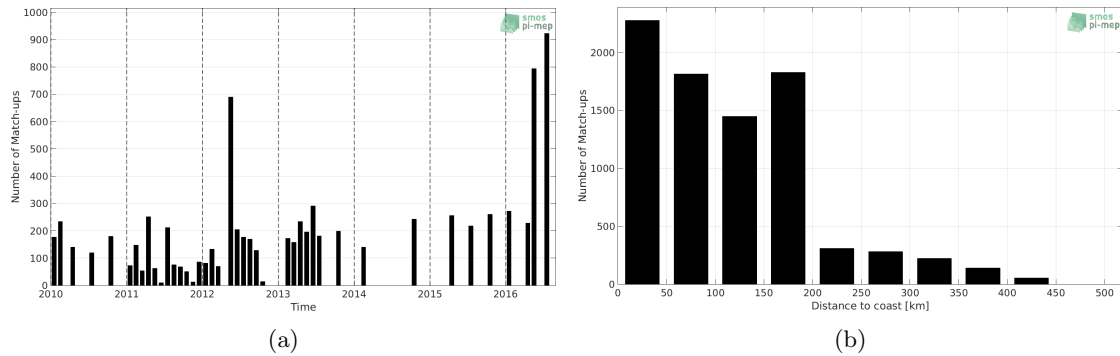
Figure 1: Number of match-ups between TSG (LEGOS-DM) and SMOS SSS L3 v7 - 9 Days (CATDS-CECOS-LOCEAN) SSS as a function of time (a) and as function of the distance to coast (b) over the South China Sea Pi-MEP region and for the full satellite product period.
