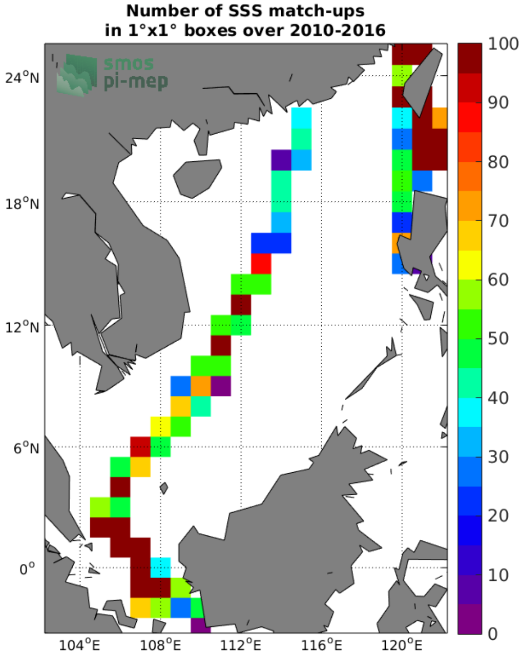
Figure 4: Number of SSS match-ups between TSG (LEGOS-DM) SSS and the SMOS SSS L3 v7 - 9 Days (CATDS-CECOS-LOCEAN) SSS product for the South China Sea Pi-MEP region over 1°x1° boxes and for the full satellite product period.
