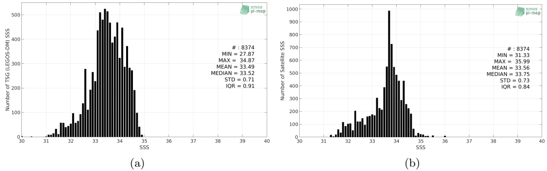
Figure 2: Histograms of SSS from TSG (LEGOS-DM) (a) and SMOS SSS L3 v7 - 9 Days (CATDS-CECOS-LOCEAN) (b) considering all match-up pairs per bins of 0.1 over the South China Sea Pi-MEP region and for the full satellite product period.
