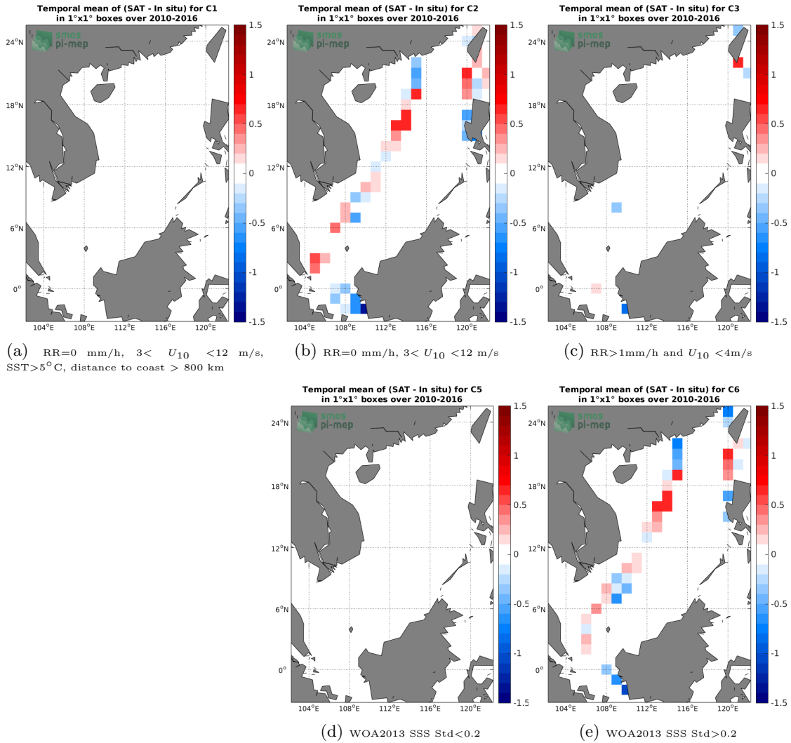
Figure 12: Temporal mean gridded over spatial boxes of size 1^\circ \times 1^\circ of \Delta\text{SSS} (SMOS SSS L3 v7 - 9 Days (CATDS-CECOS-LOCEAN) - TSG (LEGOS-DM)) for 5 different subdatasets corresponding to: RR=0 mm/h, 3 < U_{10} < 12 m/s, SST > 5^\circ\text{C} , distance to coast > 800 km (a), RR=0 mm/h, 3 < U_{10} < 12 m/s (b), RR > 1 mm/h and U_{10} < 4 m/s (c), WOA2013 SSS Std < 0.2 (d), WOA2013 SSS Std > 0.2 (e).
