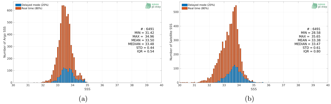
Figure 2: Histograms of SSS from Argo (a) and SMOS SSS L3 v7 - 9 Days (CATDS-CECOS-LOCEAN) (b) considering all match-up pairs per bins of 0.1 over the South China Sea Pi-MEP region and for the full satellite product period.
