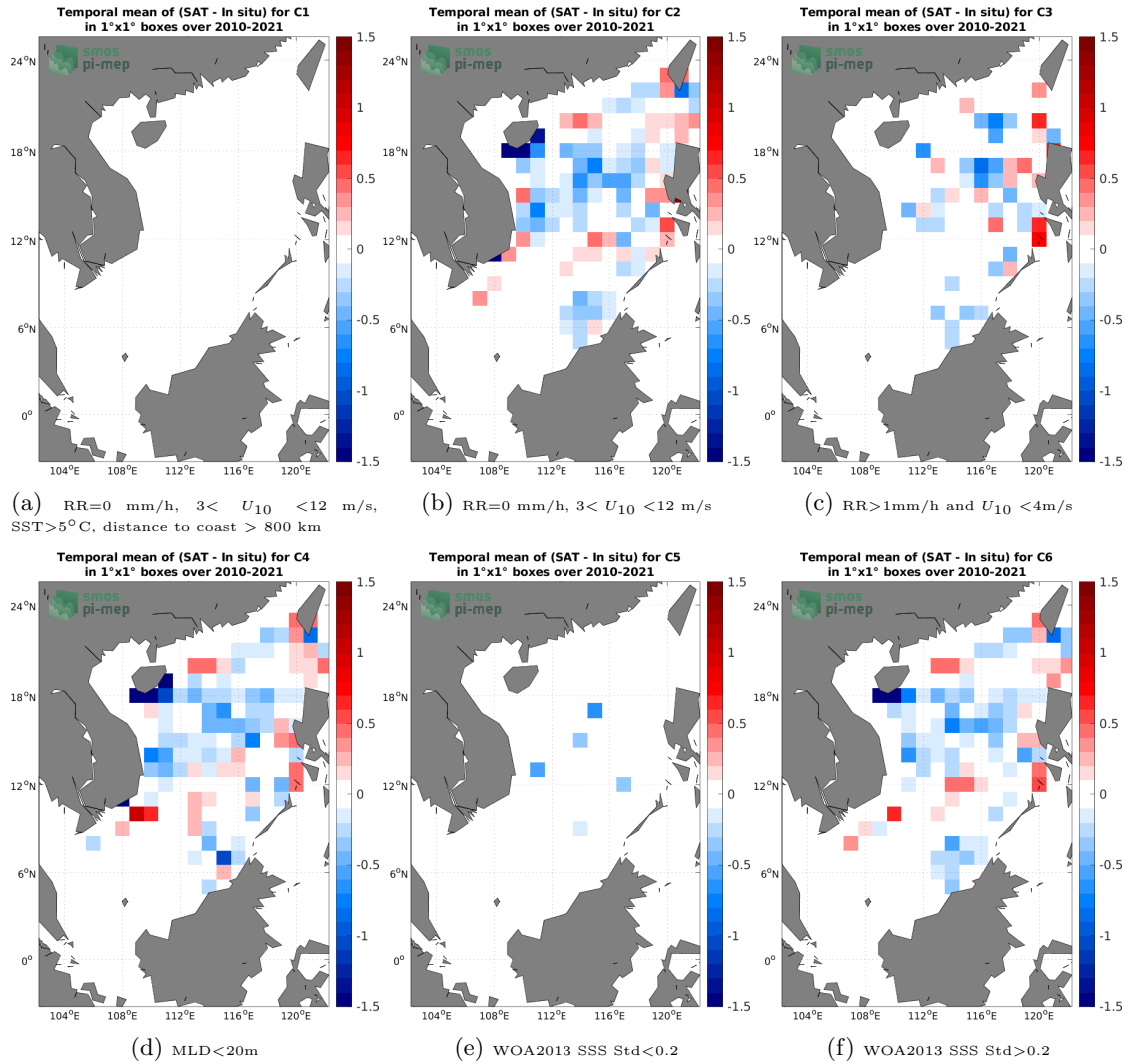
Figure 12: Temporal mean gridded over spatial boxes of size 1^\circ \times 1^\circ of \Delta SSS (SMOS SSS L3 v7 - 9 Days (CATDS-CECOS-LOCEAN) - Argo) for 6 different subdatasets corresponding to:RR=0 mm/h, 3 < U_{10} < 12 m/s, SST>5°C, distance to coast > 800 km (a), RR=0 mm/h, 3 < U_{10} < 12 m/s (b), RR>1mm/h and U_{10} < 4 m/s (c),MLD<20m (d),WOA2013 SSS Std<0.2 (e),WOA2013 SSS Std>0.2 (f).
