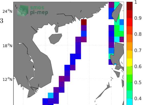
Temporal STD of (Sat - TSG (LEGOS-DM)) in 1°x1° boxes over 2010-2016
