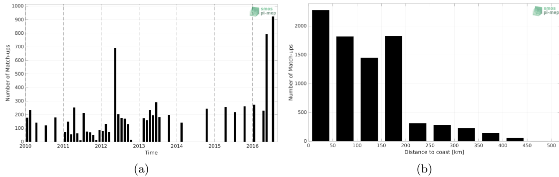
Figure 1: Number of match-ups between TSG (LEGOS-DM) and SMOS SSS L3 v7 - 18 Days (CATDS-CECOS-LOCEAN) SSS as a function of time (a) and as function of the distance to coast (b) over the South China Sea Pi-MEP region and for the full satellite product period.
