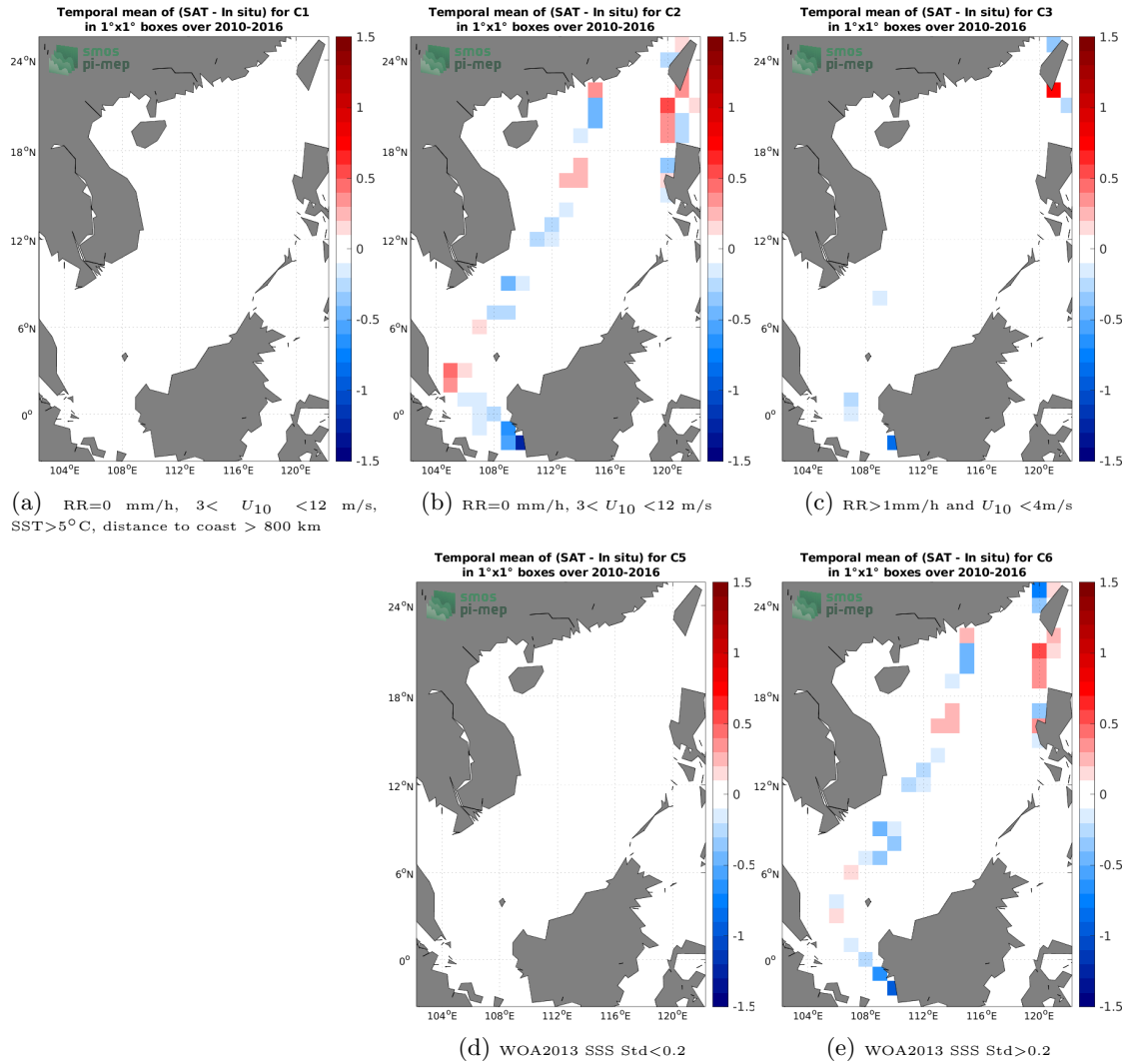
Figure 12: Temporal mean gridded over spatial boxes of size 1^\circ \times 1^\circ of \Delta\text{SSS} (SMOS SSS L3 v7 - 18 Days (CATDS-CECOS-LOCEAN) - TSG (LEGOS-DM)) for 5 different subdatasets corresponding to: RR=0 mm/h, 3 < U_{10} < 12 m/s, SST > 5^\circ\text{C} , distance to coast > 800 km (a), RR=0 mm/h, 3 < U_{10} < 12 m/s (b), RR > 1 mm/h and U_{10} < 4 m/s (c), WOA2013 SSS Std < 0.2 (d), WOA2013 SSS Std > 0.2 (e).
