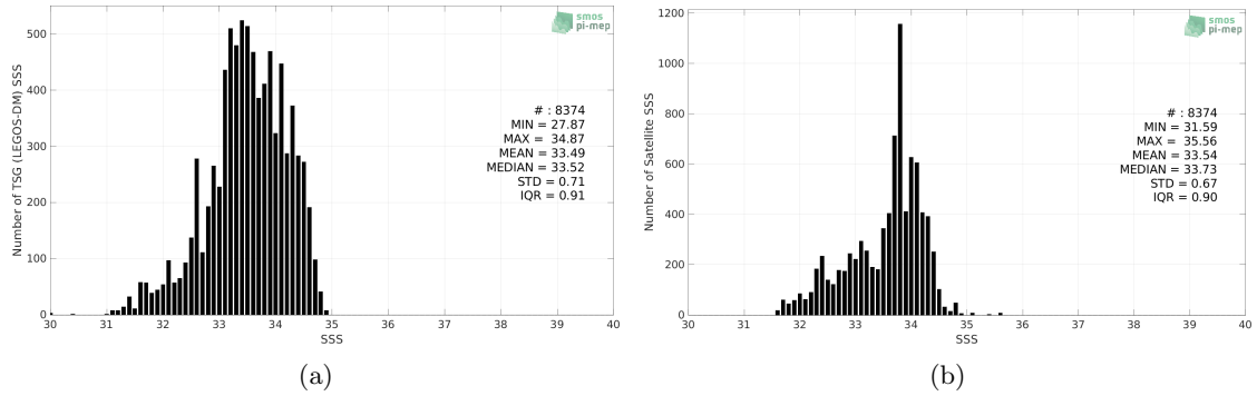
Figure 2: Histograms of SSS from TSG (LEGOS-DM) (a) and SMOS SSS L3 v7 - 18 Days (CATDS-CECOS-LOCEAN) (b) considering all match-up pairs per bins of 0.1 over the South China Sea Pi-MEP region and for the full satellite product period.
