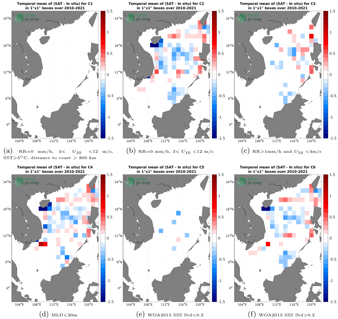
Figure 12: Temporal mean gridded over spatial boxes of size 1^\circ \times 1^\circ of \Delta\text{SSS} (SMOS SSS L3 v7 - 18 Days (CATDS-CECOS-LOCEAN) - Argo) for 6 different subdatasets corresponding to: RR=0 mm/h, 3 < U_{10} < 12 m/s, SST > 5^\circ\text{C} , distance to coast > 800 km (a), RR=0 mm/h, 3 < U_{10} < 12 m/s (b), RR > 1 mm/h and U_{10} < 4 m/s (c), MLD < 20 m (d), WOA2013 SSS Std < 0.2 (e), WOA2013 SSS Std > 0.2 (f).
