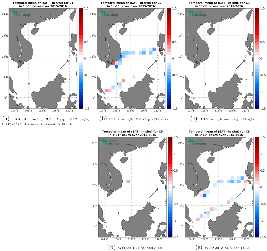
Figure 12: Temporal mean gridded over spatial boxes of size 1^\circ \times 1^\circ of \Delta SSS (SMOS SSS L3 v5 - 18 Days (CATDS-CECOS-LOCEAN) - TSG (SAMOS)) for 5 different subdatasets corresponding to:RR=0 mm/h, 3 < U_{10} < 12 m/s, SST>5°C, distance to coast > 800 km (a), RR=0 mm/h, 3 < U_{10} < 12 m/s (b), RR>1mm/h and U_{10} < 4 m/s (c), WOA2013 SSS Std<0.2 (d), WOA2013 SSS Std>0.2 (e).
