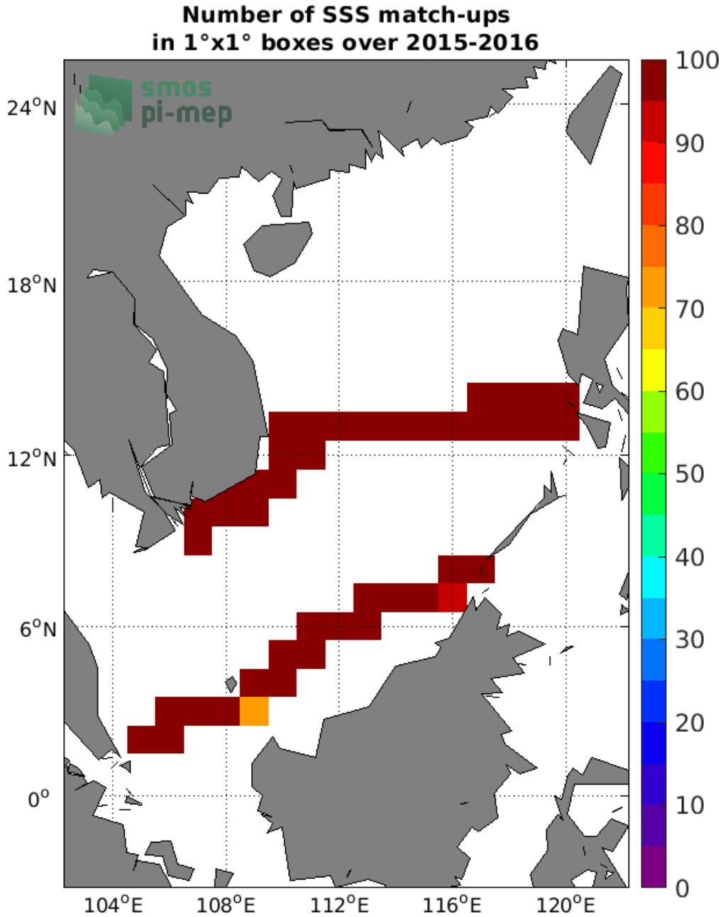
Figure 4: Number of SSS match-ups between TSG (SAMOS) SSS and the SMOS SSS L3 v5 - 18 Days (CATDS-CECOS-LOCEAN) SSS product for the South China Sea Pi-MEP region over 1°x1° boxes and for the full satellite product period.
