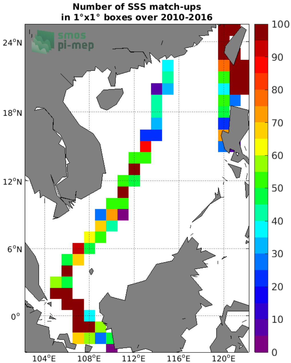
Figure 4: Number of SSS match-ups between TSG (LEGOS-DM) SSS and the SMOS SSS L3 v5 - 18 Days (CATDS-CECOS-LOCEAN) SSS product for the South China Sea Pi-MEP region over 1°x1° boxes and for the full satellite product period.
