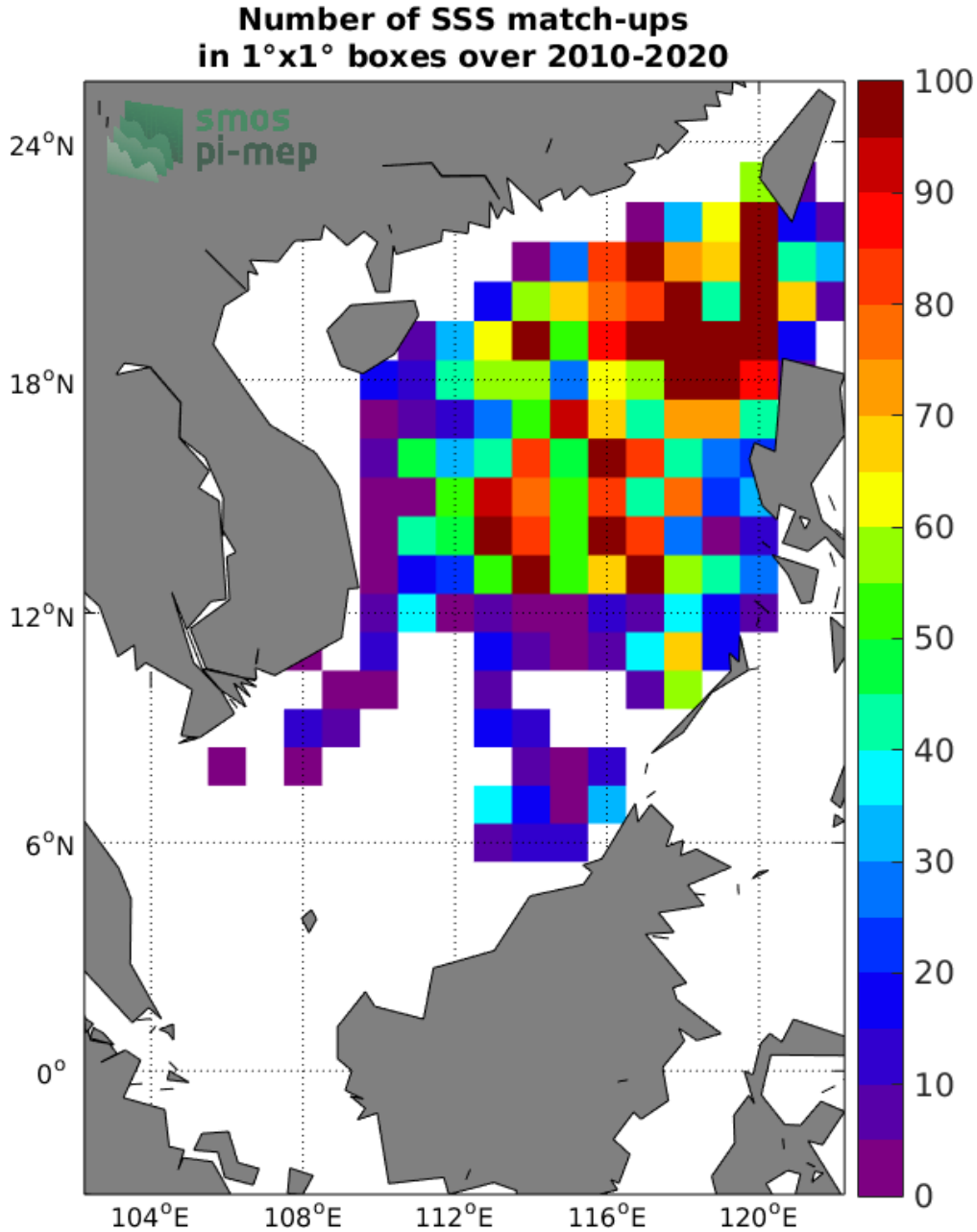
Figure 4: Number of SSS match-ups between Argo SSS and the SMOS SSS L3 v5 - 18 Days (CATDS-CECOS-LOCEAN) SSS product for the South China Sea Pi-MEP region over 1^\circ \times 1^\circ boxes and for the full satellite product period.
