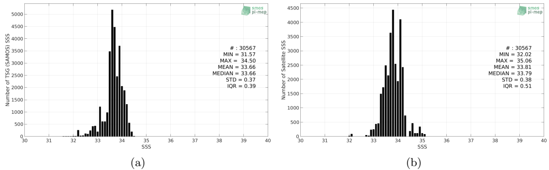
Figure 2: Histograms of SSS from TSG (SAMOS) (a) and SMOS SSS L3 v4 - 9 Days (CATDS-CECOS-LOCEAN) (b) considering all match-up pairs per bins of 0.1 over the South China Sea Pi-MEP region and for the full satellite product period.
