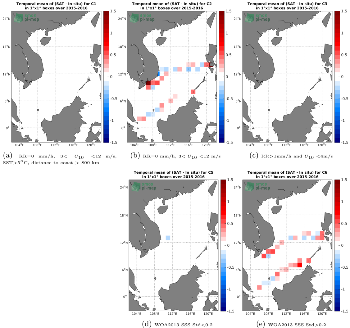
Figure 12: Temporal mean gridded over spatial boxes of size 1°x1° of \Delta SSS (SMOS SSS L3 v4 - 9 Days (CATDS-CECOS-LOCEAN) - TSG (SAMOS)) for 5 different subdatasets corresponding to:RR=0 mm/h, 3 < U_{10} < 12 m/s, SST>5°C, distance to coast > 800 km (a), RR=0 mm/h, 3 < U_{10} < 12 m/s (b), RR>1mm/h and U_{10} < 4 m/s (c), WOA2013 SSS Std<0.2 (d), WOA2013 SSS Std>0.2 (e).
