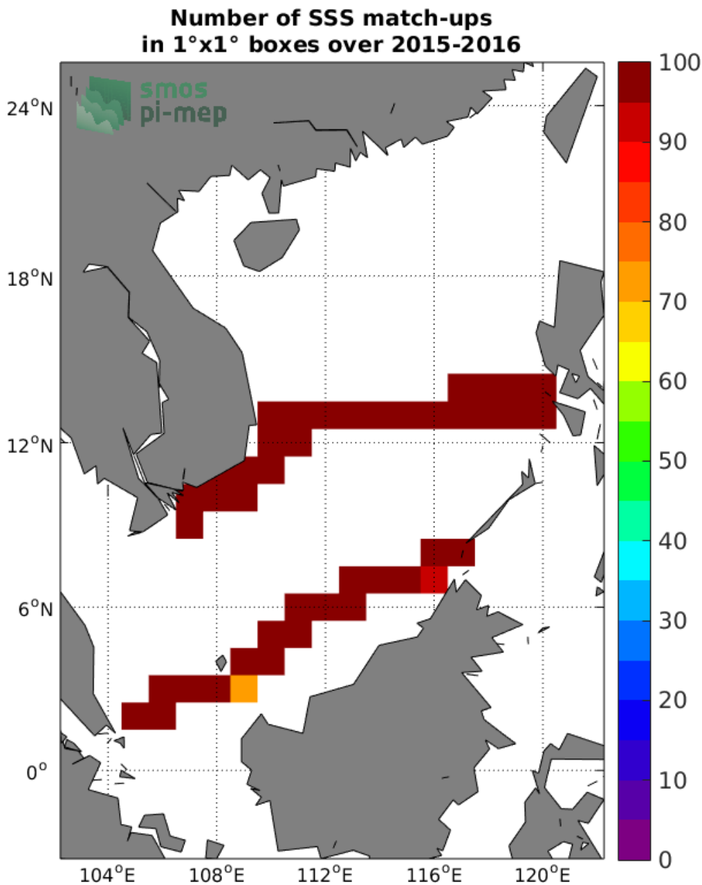
Figure 4: Number of SSS match-ups between TSG (SAMOS) SSS and the SMOS SSS L3 v4 - 9 Days (CATDS-CECOS-LOCEAN) SSS product for the South China Sea Pi-MEP region over 1°x1° boxes and for the full satellite product period.
