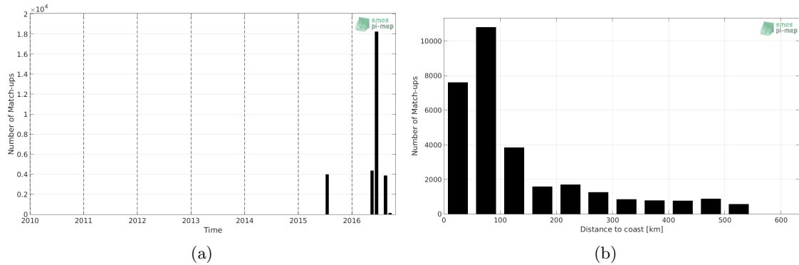
Figure 1: Number of match-ups between TSG (SAMOS) and SMOS SSS L3 v4 - 9 Days (CATDS-CECOS-LOCEAN) SSS as a function of time (a) and as function of the distance to coast (b) over the South China Sea Pi-MEP region and for the full satellite product period.
