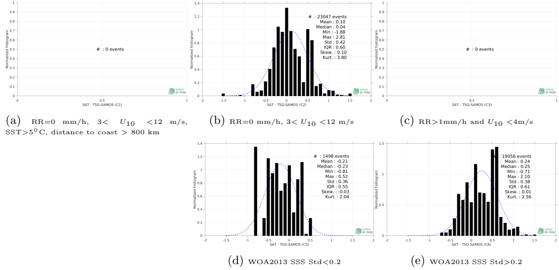
Figure 13: Normalized histogram of \Delta SSS (SMOS-L3-CATDS-CECOS-LOCEAN-V4-9DAYS-25KM - TSG-SAMOS) for 5 different subdatasets corresponding to: RR=0 mm/h, 3 < U_{10} < 12 m/s, SST > 5°C, distance to coast > 800 km (a), RR=0 mm/h, 3 < U_{10} < 12 m/s (b), RR > 1mm/h and U_{10} < 4 m/s (c), WOA2013 SSS Std < 0.2 (d), WOA2013 SSS Std > 0.2 (e).
