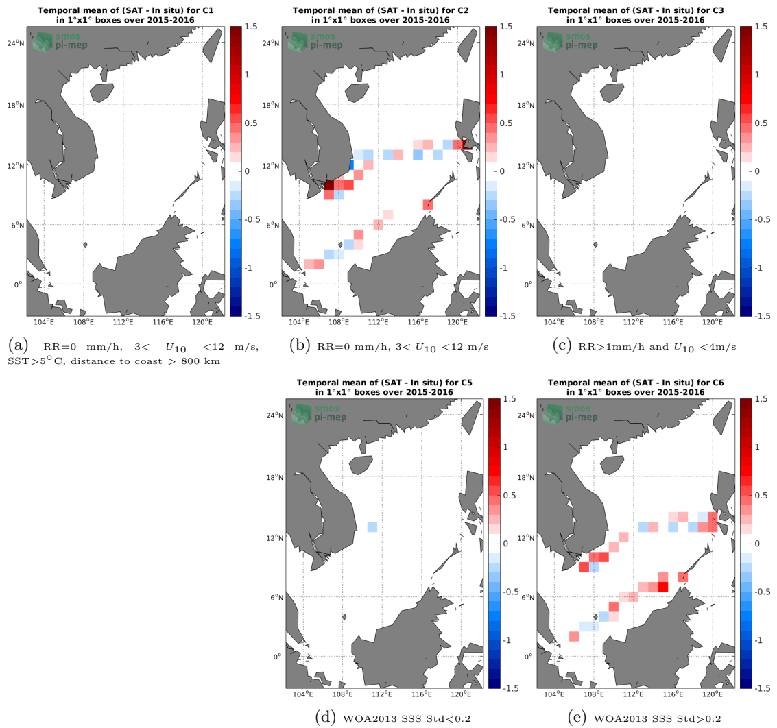
Figure 12: Temporal mean gridded over spatial boxes of size 1^\circ \times 1^\circ of \Delta SSS (SMOS-L3-CATDS-CECOS-LOCEAN-V4-9DAYS-25KM - TSG-SAMOS) for 5 different subdatasets corresponding to: RR=0 mm/h, 3 < U_{10} < 12 m/s, SST>5°C, distance to coast > 800 km (a), RR=0 mm/h, 3 < U_{10} < 12 m/s (b), RR>1mm/h and U_{10} < 4 m/s (c), WOA2013 SSS Std<0.2 (d), WOA2013 SSS Std>0.2 (e).
