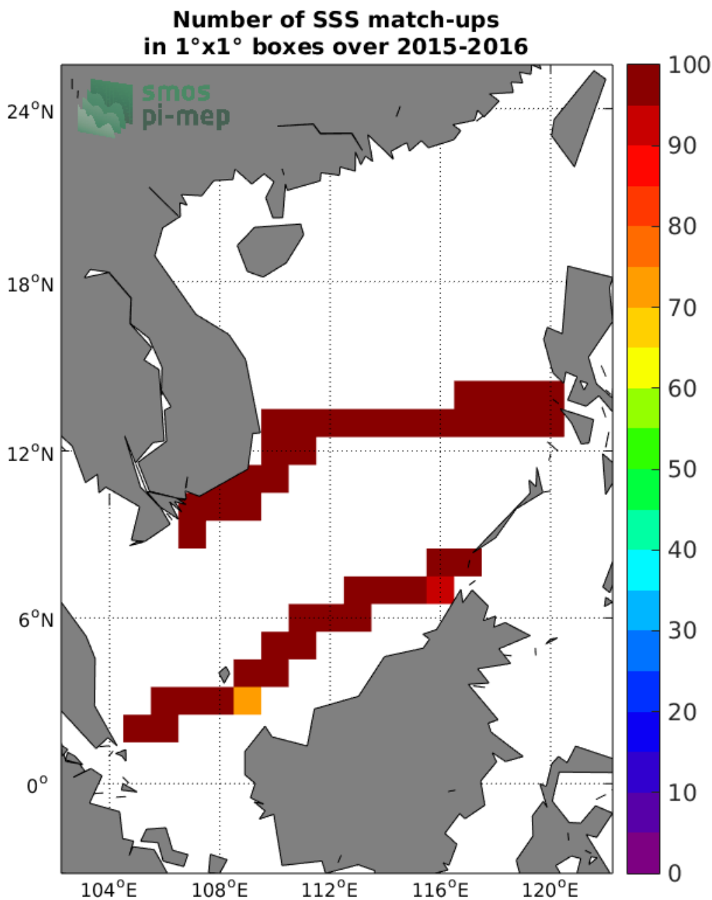
Figure 4: Number of SSS match-ups between TSG-SAMOS SSS and the SMOS-L3-CATDS-CECOS-LOCEAN-V4-9DAYS-25KM SSS product for the South China Sea Pi-MEP region over 1°x1° boxes and for the full satellite product period.
