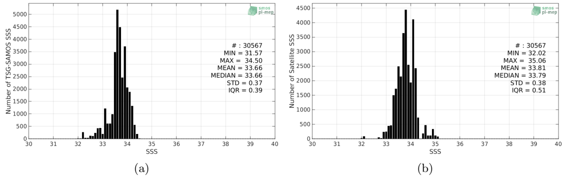
Figure 2: Histograms of SSS from TSG-SAMOS (a) and SMOS-L3-CATDS-CECOS-LOCEAN-V4-9DAYS-25KM (b) considering all match-up pairs per bins of 0.1 over the South China Sea Pi-MEP region and for the full satellite product period.
