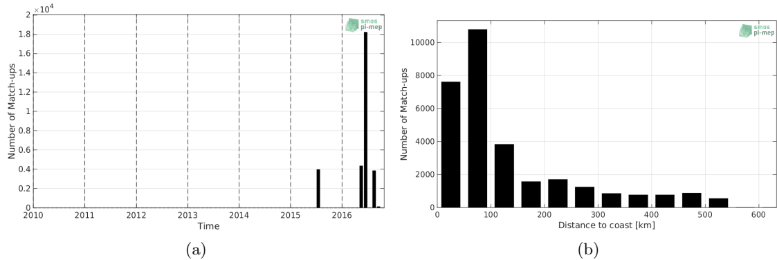
Figure 1: Number of match-ups between TSG-SAMOS and SMOS-L3-CATDS-CECOS-LOCEAN-V4-9DAYS-25KM SSS as a function of time (a) and as function of the distance to coast (b) over the South China Sea Pi-MEP region and for the full satellite product period.
