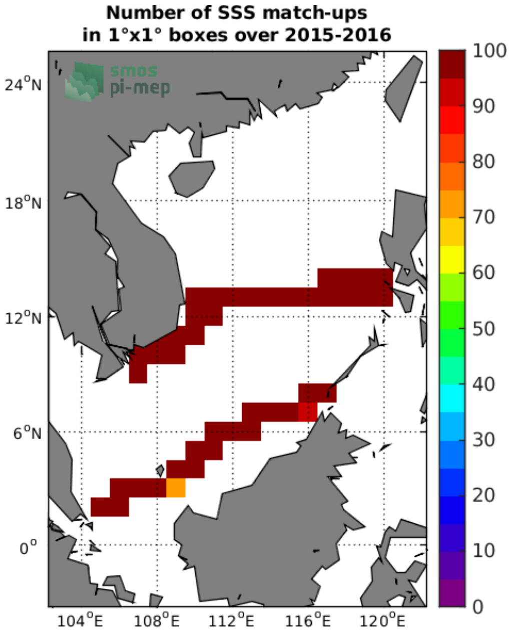
Figure 4: Number of SSS match-ups between TSG-SAMOS SSS and the SMOS-L3-CATDS-CECOS-LOCEAN-V4-9DAYS-25KM SSS product for the South China Sea Pi-MEP region over 1°x1° boxes and for the full satellite product period.
