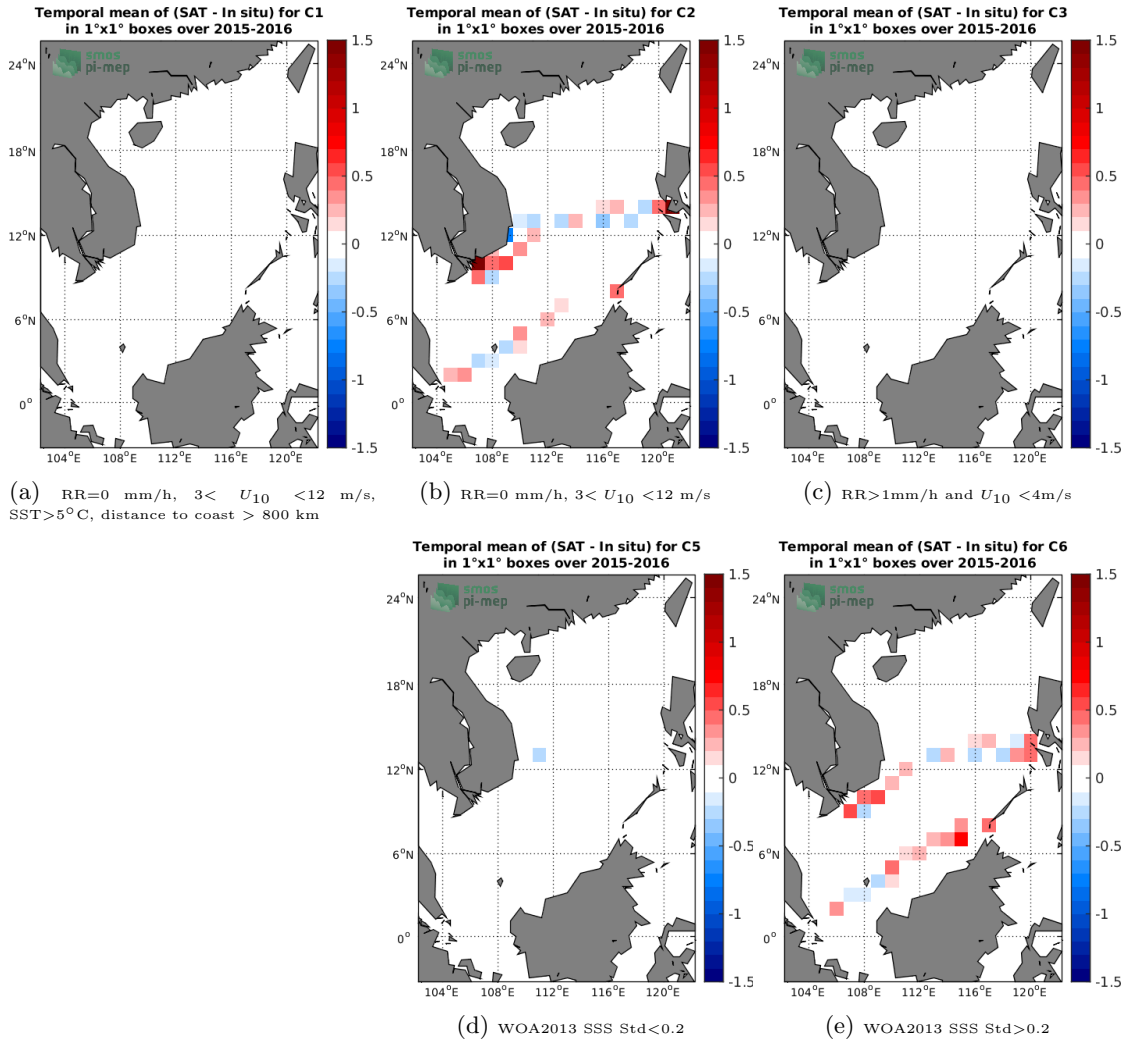
Figure 12: Temporal mean gridded over spatial boxes of size 1°x1° of \Delta SSS (SMOS-L3-CATDS-CECOS-LOCEAN-V4-9DAYS-25KM - TSG-SAMOS) for 5 different subdatasets corresponding to:RR=0 mm/h, 3 < U_{10} < 12 m/s, SST>5°C, distance to coast > 800 km (a), RR=0 mm/h, 3 < U_{10} < 12 m/s (b), RR>1mm/h and U_{10} < 4 m/s (c), WOA2013 SSS Std<0.2 (d), WOA2013 SSS Std>0.2 (e).
