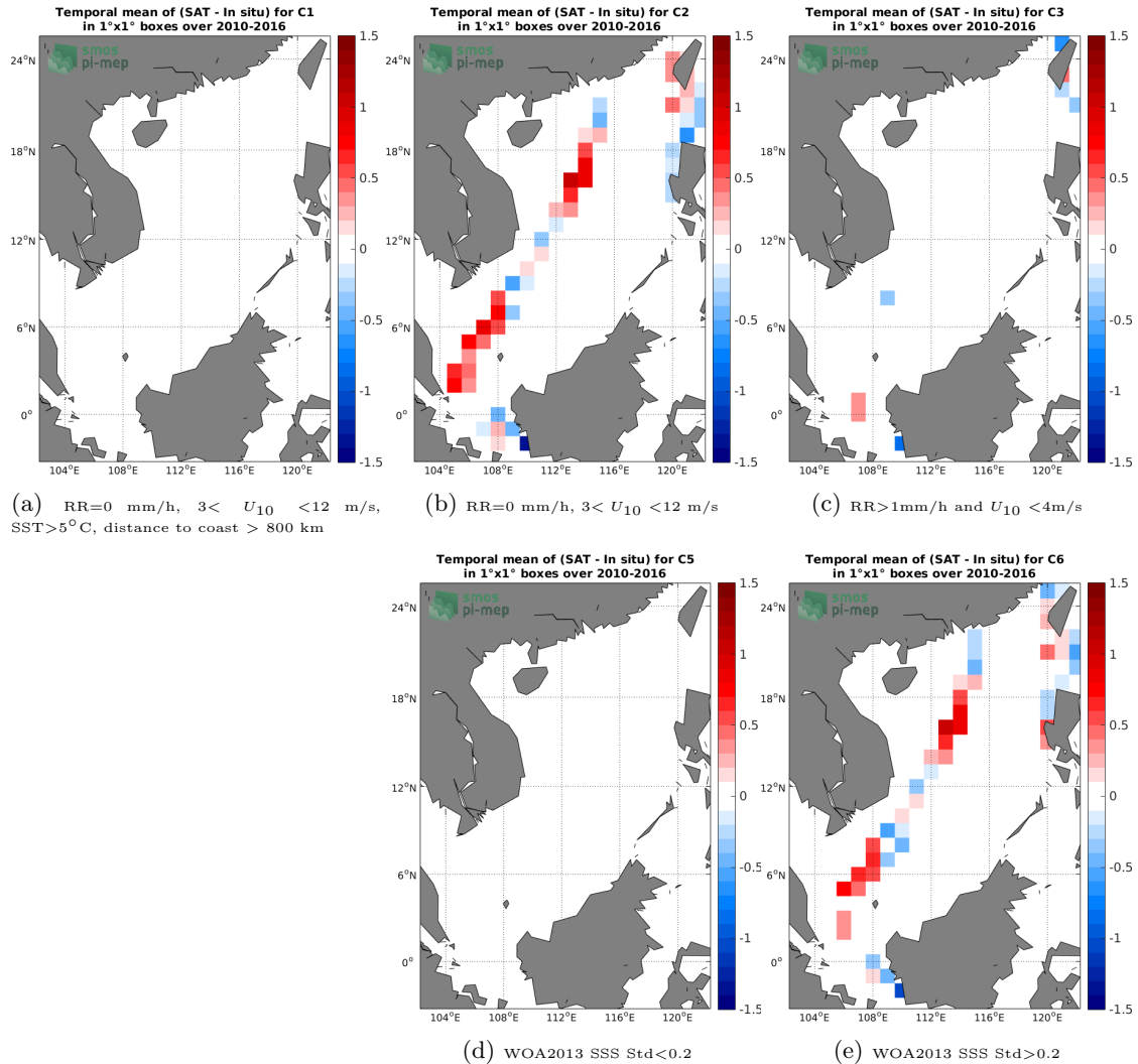
Figure 12: Temporal mean gridded over spatial boxes of size 1^\circ \times 1^\circ of \Delta\text{SSS} (SMOS SSS L3 v4 - 9 Days (CATDS-CECOS-LOCEAN) - TSG (LEGOS-DM)) for 5 different subdatasets corresponding to: RR=0 mm/h, 3 < U_{10} < 12 m/s, SST > 5^\circ\text{C} , distance to coast > 800 km (a), RR=0 mm/h, 3 < U_{10} < 12 m/s (b), RR > 1 mm/h and U_{10} < 4 m/s (c), WOA2013 SSS Std < 0.2 (d), WOA2013 SSS Std > 0.2 (e).
