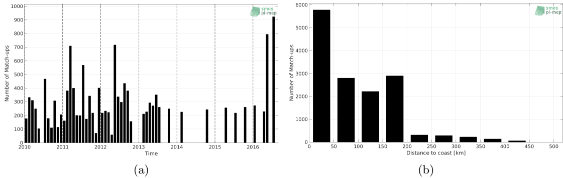
Figure 1: Number of match-ups between TSG (LEGOS-DM) and SMOS SSS L3 v4 - 9 Days (CATDS-CECOS-LOCEAN) SSS as a function of time (a) and as function of the distance to coast (b) over the South China Sea Pi-MEP region and for the full satellite product period.
