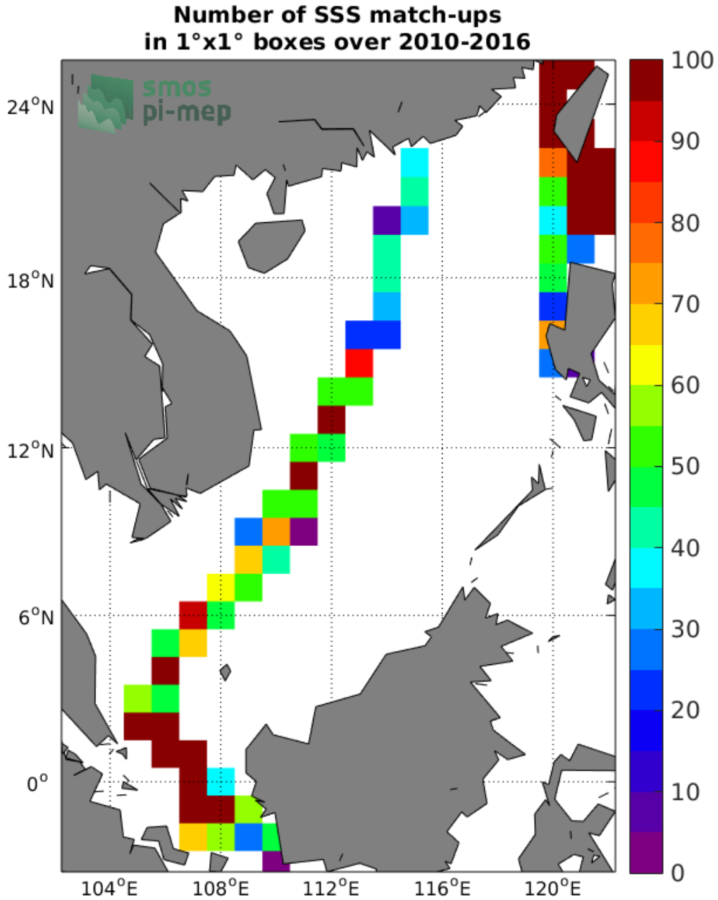
Figure 4: Number of SSS match-ups between TSG (LEGOS-DM) SSS and the SMOS SSS L3 v4 - 9 Days (CATDS-CECOS-LOCEAN) SSS product for the South China Sea Pi-MEP region over 1°x1° boxes and for the full satellite product period.
