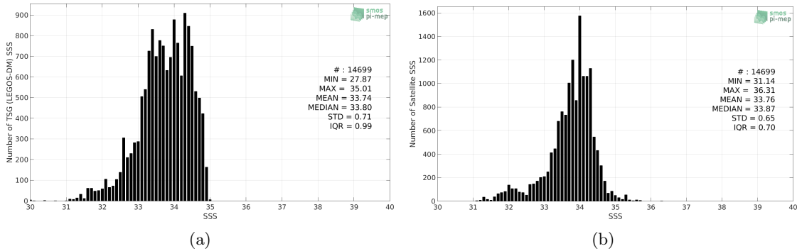
Figure 2: Histograms of SSS from TSG (LEGOS-DM) (a) and SMOS SSS L3 v4 - 9 Days (CATDS-CECOS-LOCEAN) (b) considering all match-up pairs per bins of 0.1 over the South China Sea Pi-MEP region and for the full satellite product period.
