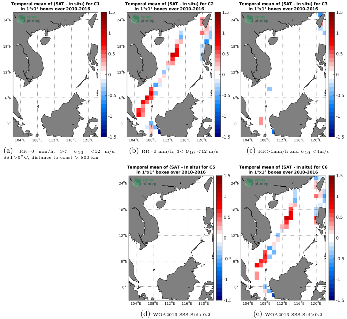
Figure 12: Temporal mean gridded over spatial boxes of size 1°x1° of \Delta SSS (SMOS-L3-CATDS-CECOS-LOCEAN-V4-9DAYS-25KM - TSG-LEGOS-DM) for 5 different subdatasets corresponding to:RR=0 mm/h, 3 < U_{10} < 12 m/s, SST>5°C, distance to coast > 800 km (a), RR=0 mm/h, 3 < U_{10} < 12 m/s (b), RR>1mm/h and U_{10} < 4 m/s (c), WOA2013 SSS Std<0.2 (d), WOA2013 SSS Std>0.2 (e).
