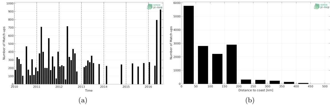
Figure 1: Number of match-ups between TSG-LEGOS-DM and SMOS-L3-CATDS-CECOS-LOCEAN-V4-18DAYS-25KM SSS as a function of time (a) and as function of the distance to coast (b) over the South China Sea Pi-MEP region and for the full satellite product period.
