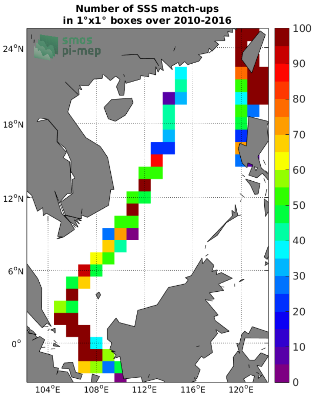
Figure 4: Number of SSS match-ups between TSG-LEGOS-DM SSS and the SMOS-L3-CATDS-CECOS-LOCEAN-V4-18DAYS-25KM SSS product for the South China Sea Pi-MEP region over 1°x1° boxes and for the full satellite product period.
