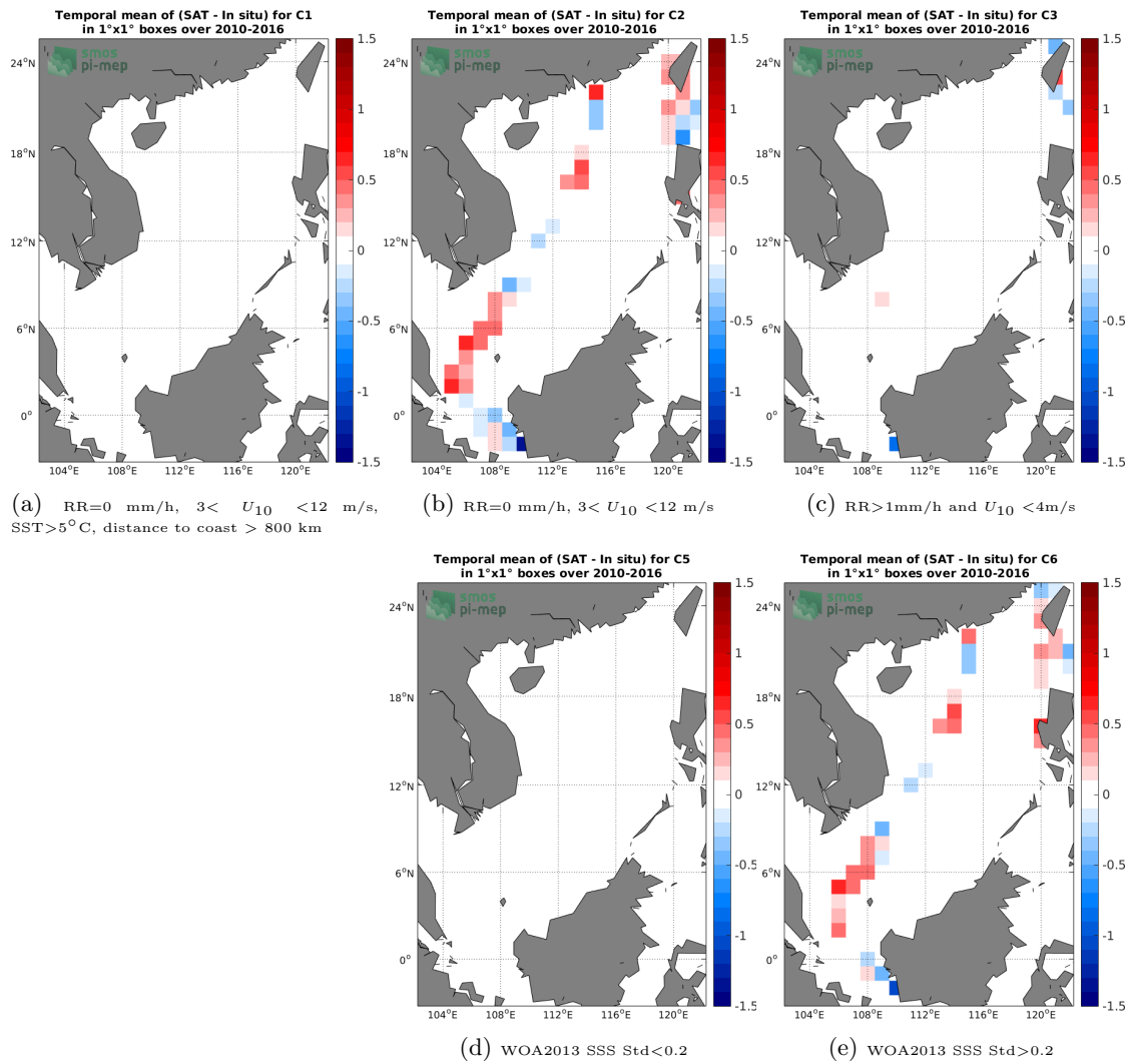
Figure 12: Temporal mean gridded over spatial boxes of size 1^\circ \times 1^\circ of \Delta\text{SSS} (SMOS-L3-CATDS-CECOS-LOCEAN-V4-18DAYS-25KM - TSG-LEGOS-DM) for 5 different subdatasets corresponding to: RR=0 mm/h, 3 < U_{10} < 12 m/s, SST > 5^\circ\text{C} , distance to coast > 800 km (a), RR=0 mm/h, 3 < U_{10} < 12 m/s (b), RR > 1 mm/h and U_{10} < 4 m/s (c), WOA2013 SSS Std < 0.2 (d), WOA2013 SSS Std > 0.2 (e).
