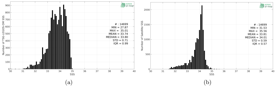
Figure 2: Histograms of SSS from TSG-LEGOS-DM (a) and SMOS-L3-CATDS-CECOS-LOCEAN-V4-18DAYS-25KM (b) considering all match-up pairs per bins of 0.1 over the South China Sea Pi-MEP region and for the full satellite product period.
