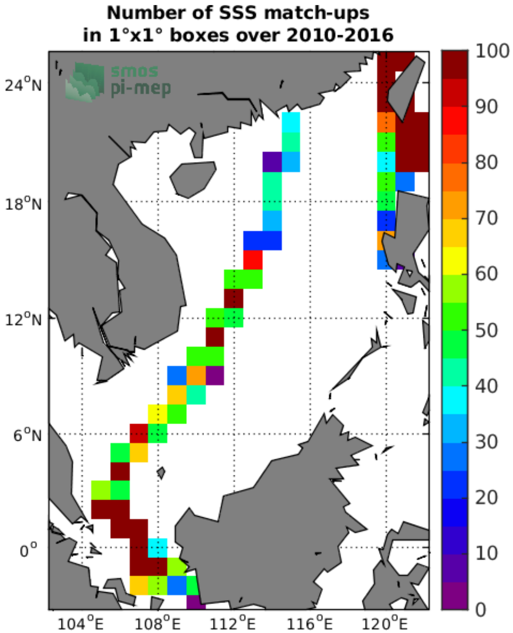
Figure 4: Number of SSS match-ups between TSG-LEGOS-DM SSS and the SMOS-L3-CATDS-CECOS-LOCEAN-V4-18DAYS-25KM SSS product for the South China Sea Pi-MEP region over 1°x1° boxes and for the full satellite product period.
