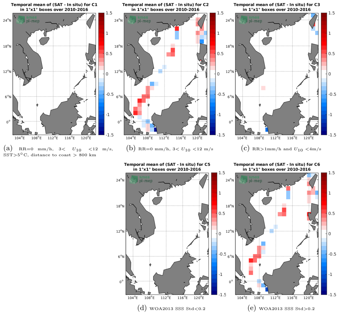
Figure 12: Temporal mean gridded over spatial boxes of size 1°x1° of \Delta SSS (SMOS-L3-CATDS-CECOS-LOCEAN-V4-18DAYS-25KM - TSG-LEGOS-DM) for 5 different subdatasets corresponding to:RR=0 mm/h, 3 < U_{10} < 12 m/s, SST>5°C, distance to coast > 800 km (a), RR=0 mm/h, 3 < U_{10} < 12 m/s (b), RR>1mm/h and U_{10} < 4 m/s (c), WOA2013 SSS Std<0.2 (d), WOA2013 SSS Std>0.2 (e).
