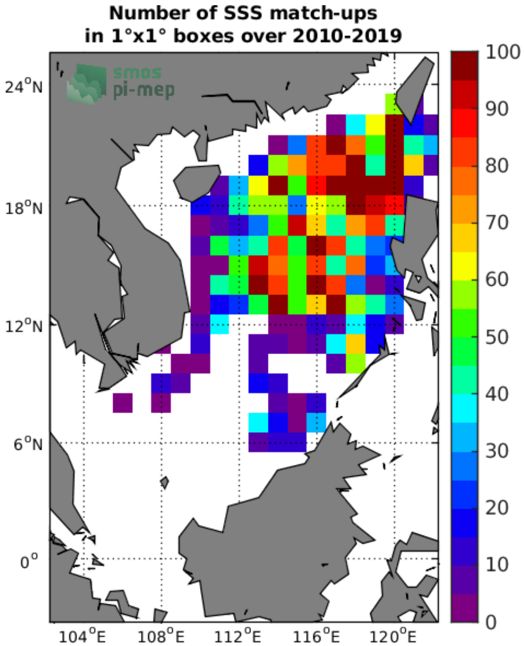
Figure 4: Number of SSS match-ups between Argo SSS and the SMOS-L3-CATDS-CECOS-LOCEAN-V4-18DAYS-25KM SSS product for the South China Sea Pi-MEP region over 1°x1° boxes and for the full satellite product period.
