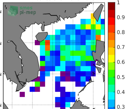
Temporal STD of (Sat - Argo) in 1°x1° boxes over 2010-2019
