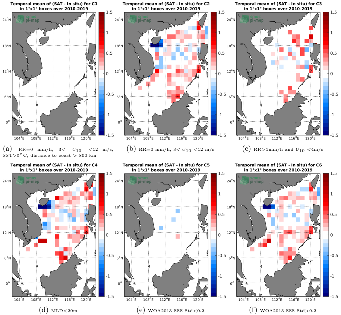
Figure 12: Temporal mean gridded over spatial boxes of size 1°x1° of \Delta SSS (SMOS-L3-CATDS-CECOS-LOCEAN-V4-18DAYS-25KM - Argo) for 6 different subdatasets corresponding to:RR=0 mm/h, 3 < U_{10} < 12 m/s, SST>5°C, distance to coast > 800 km (a), RR=0 mm/h, 3 < U_{10} < 12 m/s (b), RR>1mm/h and U_{10} < 4 m/s (c),MLD<20m (d),WOA2013 SSS Std<0.2 (e),WOA2013 SSS Std>0.2 (f).
