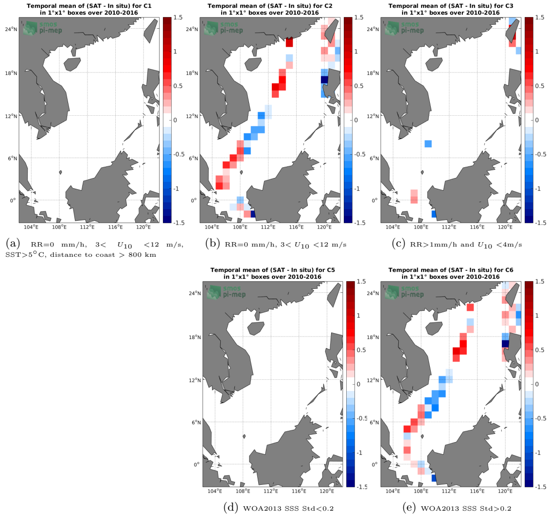
Figure 12: Temporal mean gridded over spatial boxes of size 1^\circ \times 1^\circ of \Delta SSS (SMOS-L3-CATDS-CECOS-LOCEAN-V3-9DAYS-25KM - TSG-LEGOS-DM) for 5 different subdatasets corresponding to:RR=0 mm/h, 3 < U_{10} < 12 m/s, SST>5°C, distance to coast > 800 km (a), RR=0 mm/h, 3 < U_{10} < 12 m/s (b), RR>1mm/h and U_{10} < 4 m/s (c), WOA2013 SSS Std<0.2 (d), WOA2013 SSS Std>0.2 (e).
