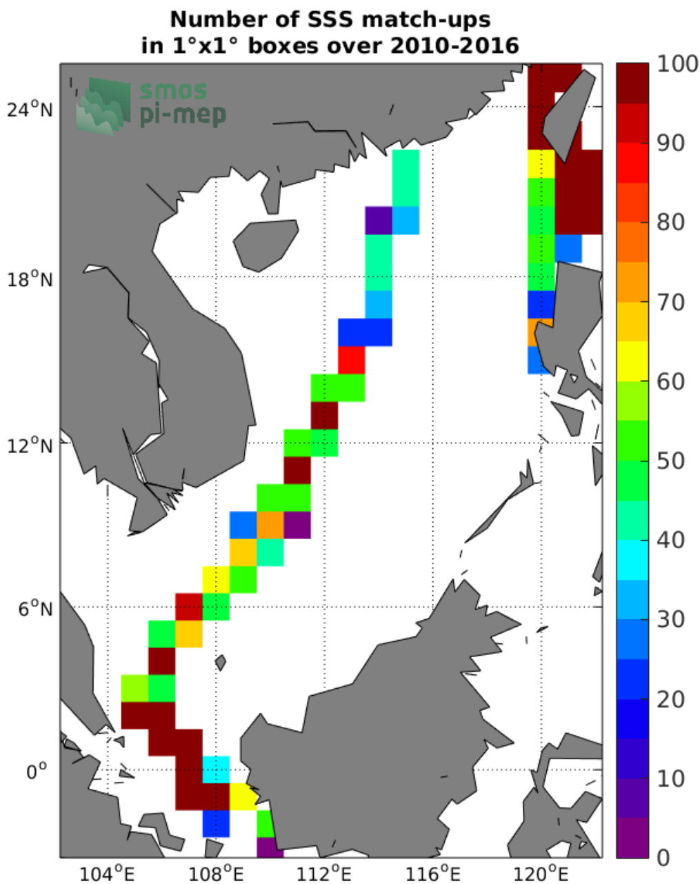
Figure 4: Number of SSS match-ups between TSG-LEGOS-DM SSS and the SMOS-L3-CATDS-CECOS-LOCEAN-V3-9DAYS-25KM SSS product for the South China Sea Pi-MEP region over 1°x1° boxes and for the full satellite product period.
