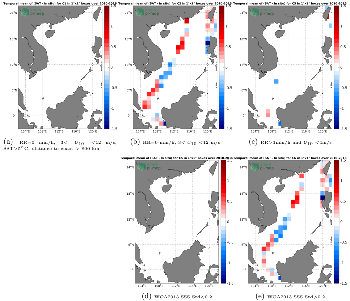
Figure 12: Temporal mean gridded over spatial boxes of size 1^\circ \times 1^\circ of \Delta SSS (SMOS-L3-CATDS-CECOS-LOCEAN-V3-9DAYS-25KM - TSG-LEGOS-DM) for 5 different subdatasets corresponding to:RR=0 mm/h, 3 < U_{10} < 12 m/s, SST >5^\circ C, distance to coast > 800 km (a), RR=0 mm/h, 3 < U_{10} < 12 m/s (b), RR >1 mm/h and U_{10} < 4 m/s (c), WOA2013 SSS Std <0.2 (d), WOA2013 SSS Std >0.2 (e).
