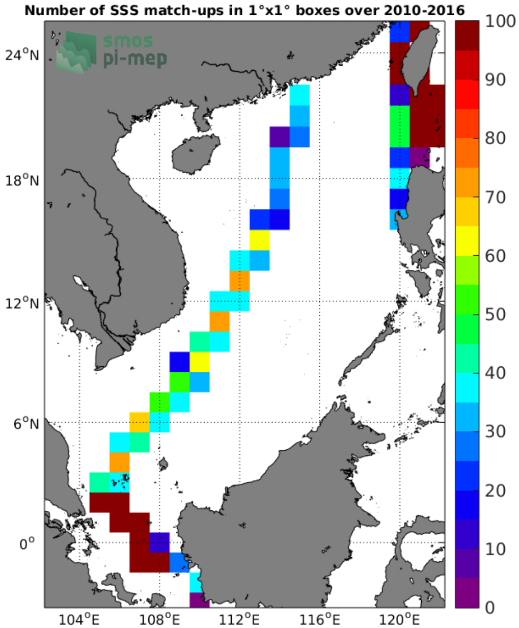
Figure 4: Number of SSS match-ups between TSG-LEGOS-DM SSS and the SMOS-L3-CATDS-CECOS-LOCEAN-V3-9DAYS-25KM SSS product for the South China Sea Pi-MEP region over 1°x1° boxes and for the full satellite product period.
