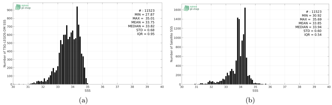
Figure 2: Histograms of SSS from TSG-LEGOS-DM (a) and SMOS-L3-CATDS-CECOS-LOCEAN-V3-9DAYS-25KM (b) considering all match-up pairs per bins of 0.1 over the South China Sea Pi-MEP region and for the full satellite product period.
