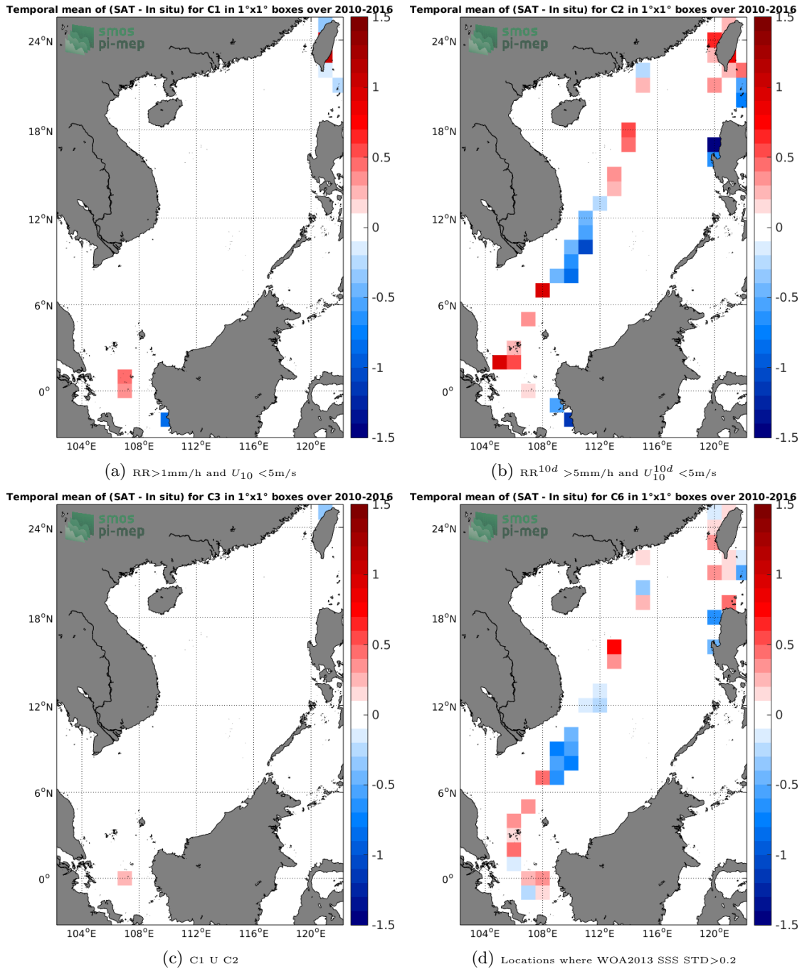
Figure 12: Temporal mean gridded over spatial boxes of size 1°x1° of \Delta SSS (SMOS-L3-CATDS-CECOS-LOCEAN-V3-9DAYS-25KM - TSG-LEGOS-DM) for 4 different subdatasets corresponding to: RR > 1\text{mm/h} and U_{10} < 5\text{m/s} (a), RR^{10d} > 5\text{mm/h} and U_{10}^{10d} < 5\text{m/s} (b), C1 U C2 (c), Locations where WOA2013 SSS STD > 0.2 (d).
