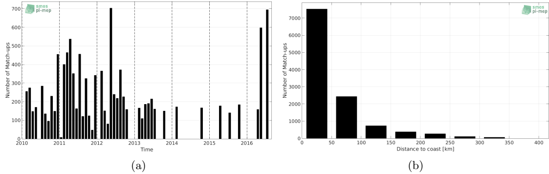
Figure 1: Number of match-ups between TSG-LEGOS-DM and SMOS-L3-CATDS-CECOS-LOCEAN-V3-9DAYS-25KM SSS as a function of time (a) and as function of the distance to coast (b) over the South China Sea Pi-MEP region and for the full satellite product period.
