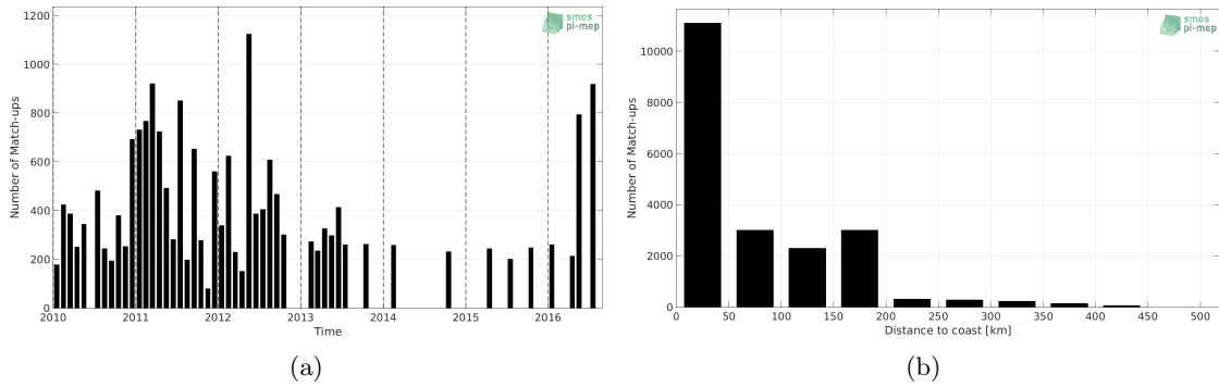
Figure 1: Number of match-ups between TSG-LEGOS-DM and SMOS-L3-CATDS-CECOS-LOCEAN-V3-18DAYS-25KM SSS as a function of time (a) and as function of the distance to coast (b) over the South China Sea Pi-MEP region and for the full satellite product period.
