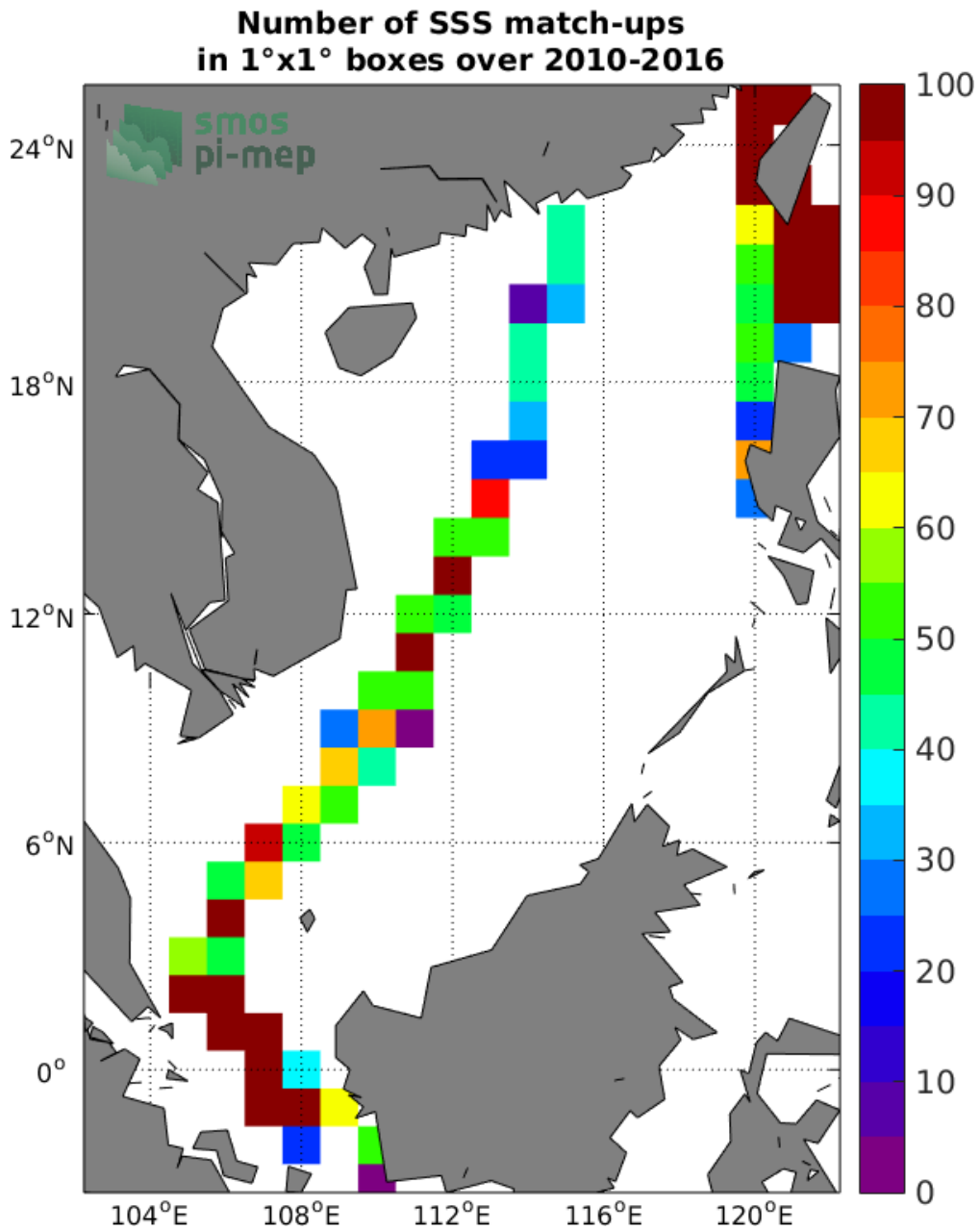
Figure 4: Number of SSS match-ups between TSG-LEGOS-DM SSS and the SMOS-L3-CATDS-CECOS-LOCEAN-V3-18DAYS-25KM SSS product for the South China Sea Pi-MEP region over 1°x1° boxes and for the full satellite product period.
