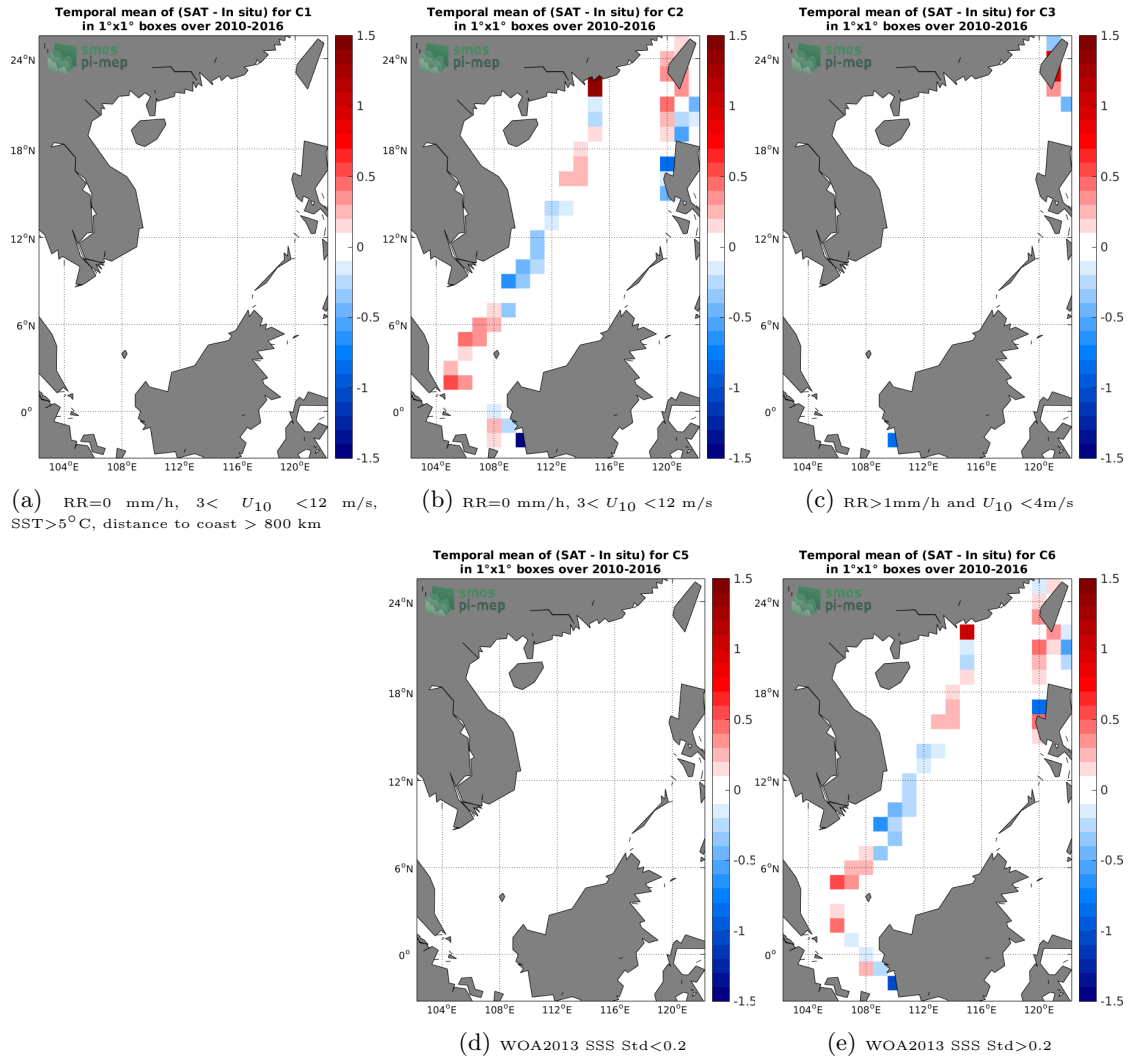
Figure 12: Temporal mean gridded over spatial boxes of size 1°x1° of \Delta SSS (SMOS-L3-CATDS-CECOS-LOCEAN-V3-18DAYS-25KM - TSG-LEGOS-DM) for 5 different subdatasets corresponding to:RR=0 mm/h, 3 < U_{10} < 12 m/s, SST>5°C, distance to coast > 800 km (a), RR=0 mm/h, 3 < U_{10} < 12 m/s (b), RR>1mm/h and U_{10} < 4 m/s (c), WOA2013 SSS Std<0.2 (d), WOA2013 SSS Std>0.2 (e).
