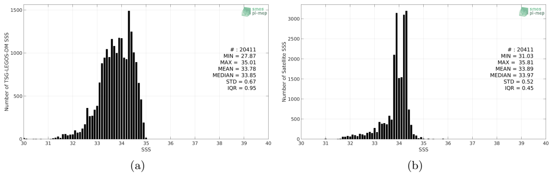
Figure 2: Histograms of SSS from TSG-LEGOS-DM (a) and SMOS-L3-CATDS-CECOS-LOCEAN-V3-18DAYS-25KM (b) considering all match-up pairs per bins of 0.1 over the South China Sea Pi-MEP region and for the full satellite product period.
