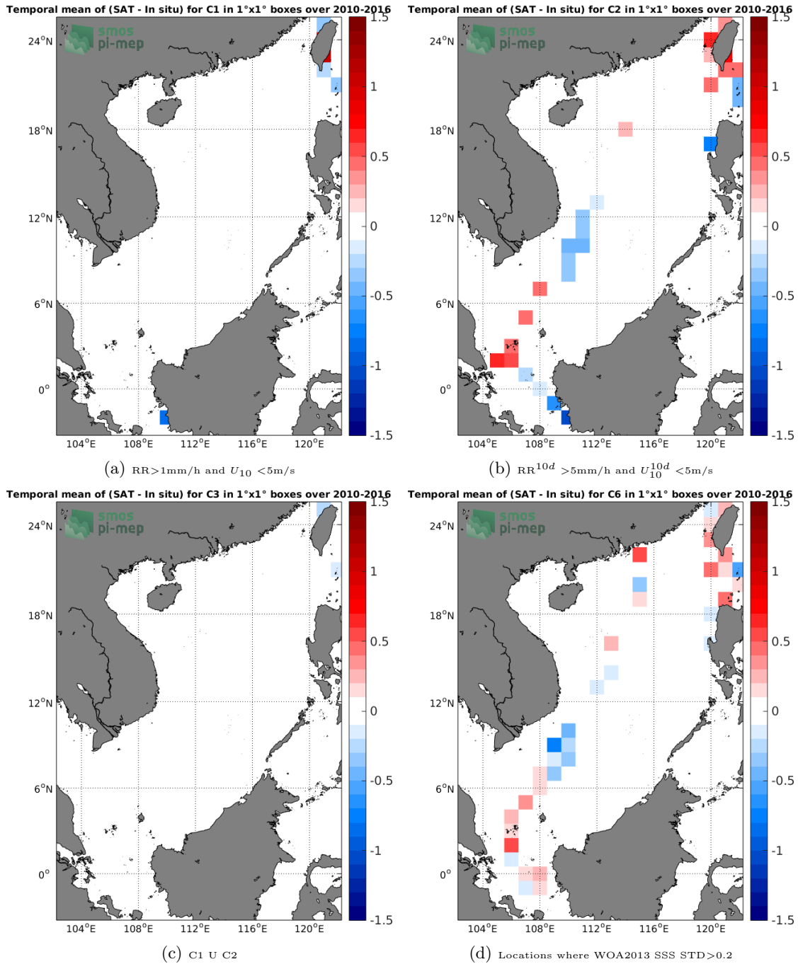
Figure 12: Temporal mean gridded over spatial boxes of size 1°x1° of \Delta\text{SSS} (SMOS-L3-CATDS-CECOS-LOCEAN-V3-18DAYS-25KM - TSG-LEGOS-DM) for 4 different subdatasets corresponding to: RR > 1\text{mm/h} and U_{10} < 5\text{m/s} (a), RR^{10d} > 5\text{mm/h} and U_{10}^{10d} < 5\text{m/s} (b), C1 U C2 (c), Locations where WOA2013 SSS STD > 0.2 (d).
