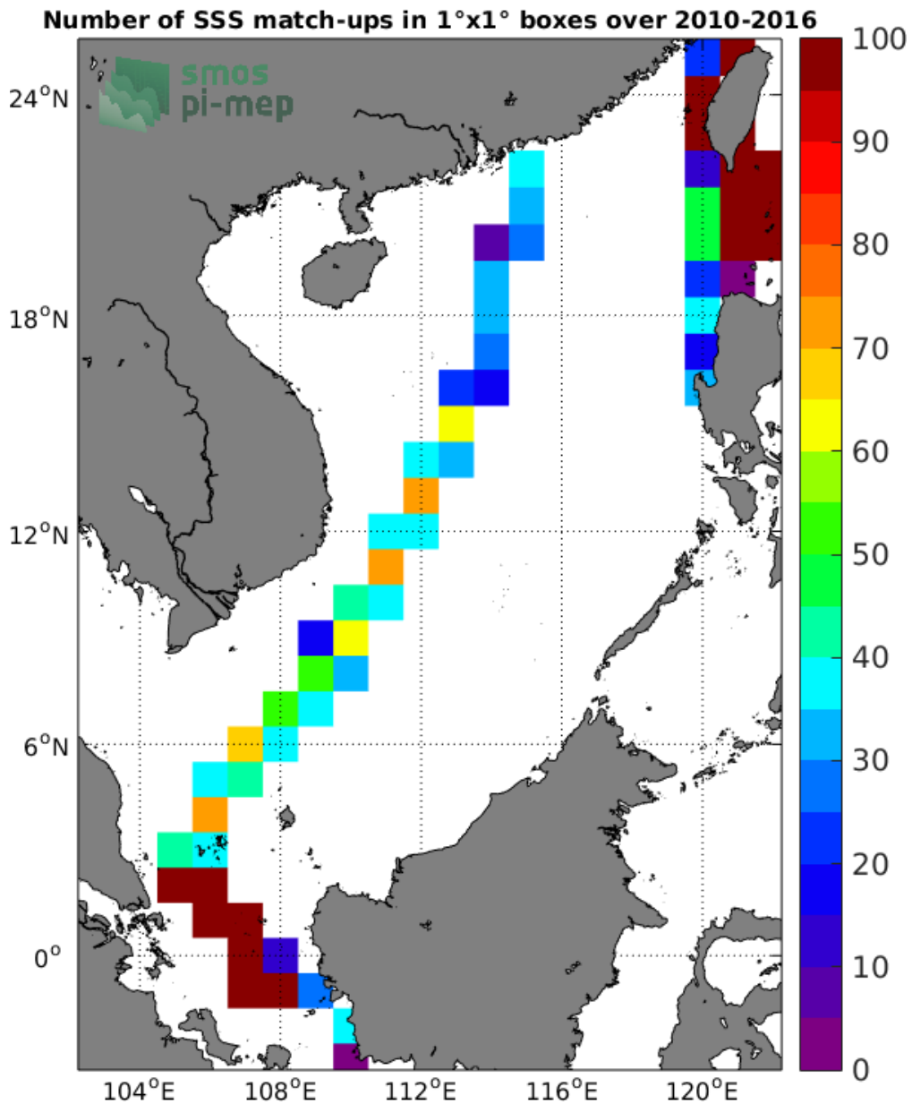
Figure 4: Number of SSS match-ups between TSG-LEGOS-DM SSS and the SMOS-L3-CATDS-CECOS-LOCEAN-V3-18DAYS-25KM SSS product for the South China Sea Pi-MEP region over 1°x1° boxes and for the full satellite product period.
