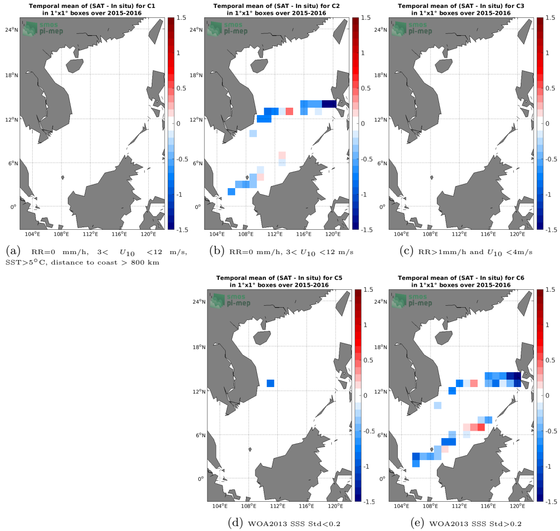
Figure 12: Temporal mean gridded over spatial boxes of size 1°x1° of \Delta SSS (SMOS SSS L3 v2 - Monthly - 0.25 Deg (CATDS-CECOS-IFREMER) - TSG (SAMOS)) for 5 different subdatasets corresponding to: RR=0 mm/h, 3 < U_{10} < 12 m/s, SST > 5°C, distance to coast > 800 km (a), RR=0 mm/h, 3 < U_{10} < 12 m/s (b), RR > 1mm/h and U_{10} < 4 m/s (c), WOA2013 SSS Std < 0.2 (d), WOA2013 SSS Std > 0.2 (e).
