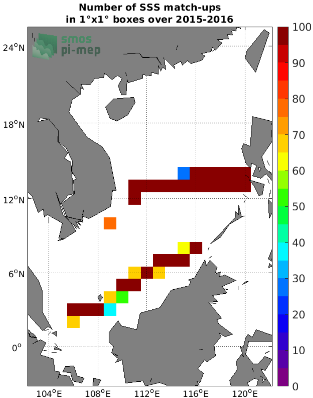
Figure 4: Number of SSS match-ups between TSG (SAMOS) SSS and the SMOS SSS L3 v2 - Monthly - 0.25 Deg (CATDS-CECOS-IFREMER) SSS product for the South China Sea Pi-MEP region over 1°x1° boxes and for the full satellite product period.
