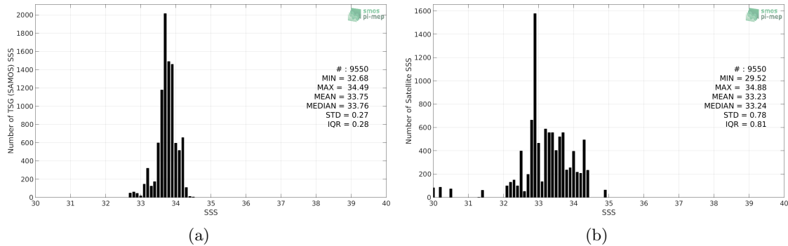
Figure 2: Histograms of SSS from TSG (SAMOS) (a) and SMOS SSS L3 v2 - Monthly - 0.25 Deg (CATDS-CECOS-IFREMER) (b) considering all match-up pairs per bins of 0.1 over the South China Sea Pi-MEP region and for the full satellite product period.
