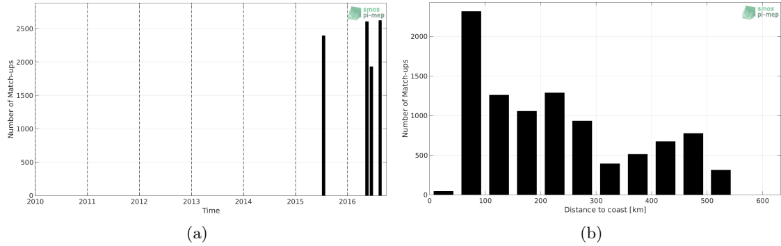
Figure 1: Number of match-ups between TSG (SAMOS) and SMOS SSS L3 v2 - Monthly - 0.25 Deg (CATDS-CECOS-IFREMER) SSS as a function of time (a) and as function of the distance to coast (b) over the South China Sea Pi-MEP region and for the full satellite product period.
