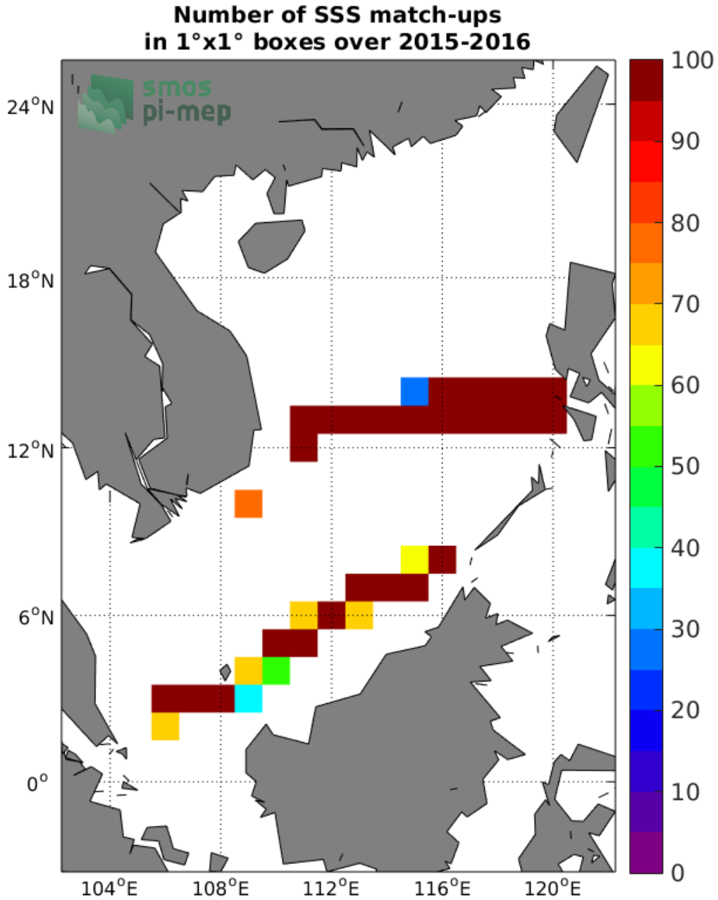
Figure 4: Number of SSS match-ups between TSG (SAMOS) SSS and the SMOS SSS L3 v2 - Monthly - 0.25 Deg (CATDS-CECOS-IFREMER) SSS product for the South China Sea Pi-MEP region over 1°x1° boxes and for the full satellite product period.
