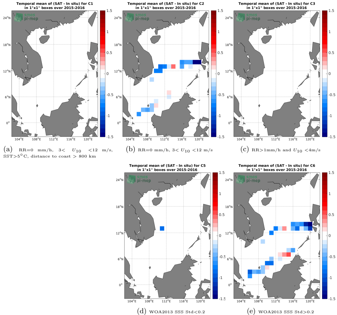
Figure 12: Temporal mean gridded over spatial boxes of size 1^\circ \times 1^\circ of \Delta SSS (SMOS SSS L3 v2 - Monthly - 0.25 Deg (CATDS-CECOS-IFREMER) - TSG (SAMOS)) for 5 different subdatasets corresponding to: RR=0 mm/h, 3 < U_{10} < 12 m/s, SST>5°C, distance to coast > 800 km (a), RR=0 mm/h, 3 < U_{10} < 12 m/s (b), RR>1mm/h and U_{10} < 4 m/s (c), WOA2013 SSS Std<0.2 (d), WOA2013 SSS Std>0.2 (e).
