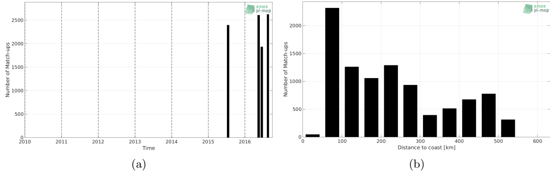
Figure 1: Number of match-ups between TSG-SAMOS and SMOS L3 v2 - Monthly - 0.25 Deg (CATDS-CECOS-IFREMER) SSS as a function of time (a) and as function of the distance to coast (b) over the South China Sea Pi-MEP region and for the full satellite product period.
