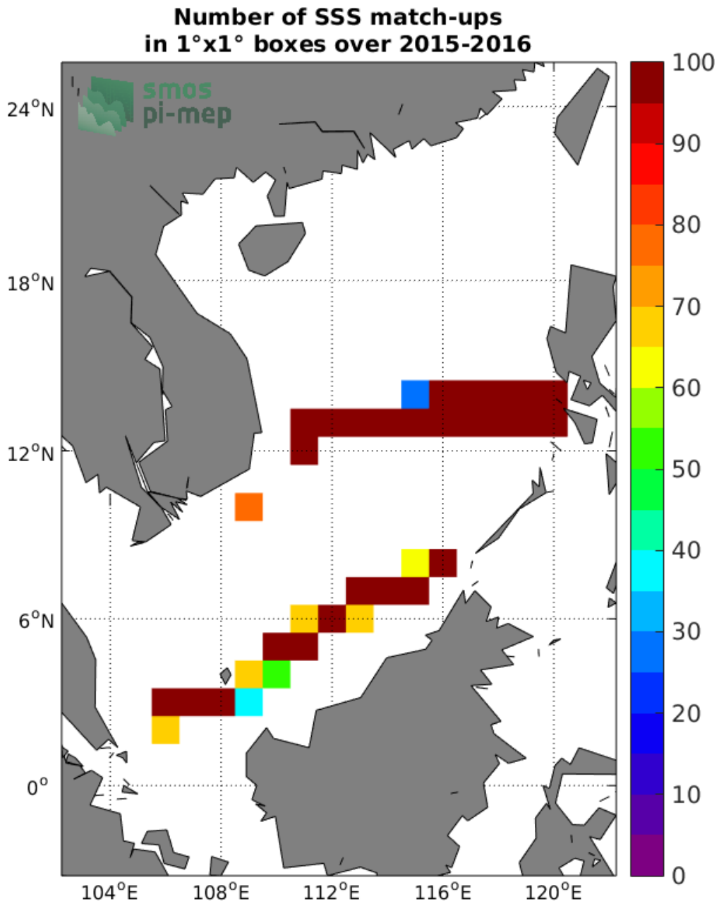
Figure 4: Number of SSS match-ups between TSG-SAMOS SSS and the SMOS L3 v2 - Monthly - 0.25 Deg (CATDS-CECOS-IFREMER) SSS product for the South China Sea Pi-MEP region over 1°x1° boxes and for the full satellite product period.
