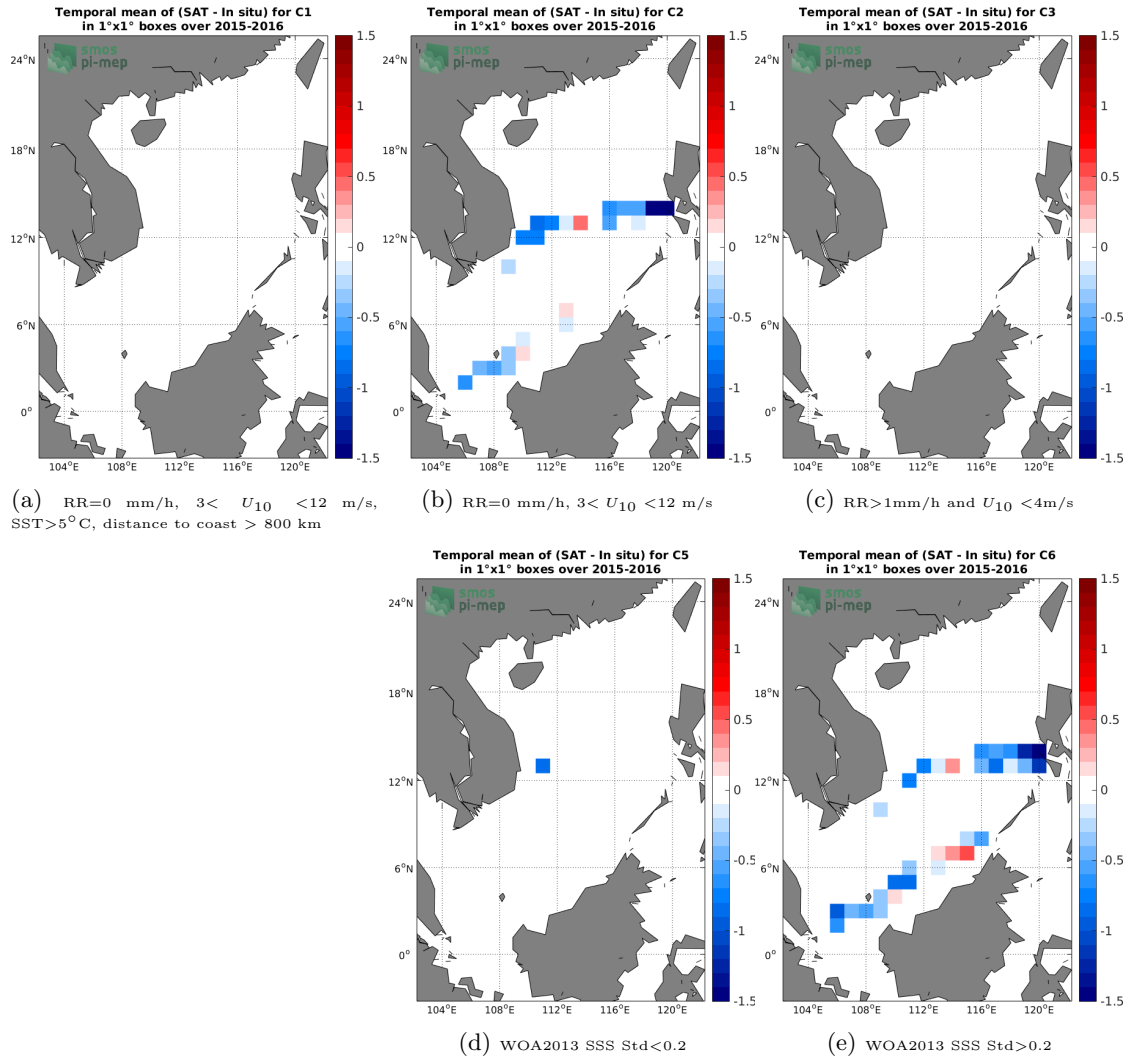
Figure 12: Temporal mean gridded over spatial boxes of size 1°x1° of \Delta SSS (SMOS L3 v2 - Monthly - 0.25 Deg (CATDS-CECOS-IFREMER) - TSG-SAMOS) for 5 different subdatasets corresponding to:RR=0 mm/h, 3 < U_{10} < 12 m/s, SST>5°C, distance to coast > 800 km (a), RR=0 mm/h, 3 < U_{10} < 12 m/s (b), RR>1mm/h and U_{10} < 4 m/s (c), WOA2013 SSS Std<0.2 (d), WOA2013 SSS Std>0.2 (e).
