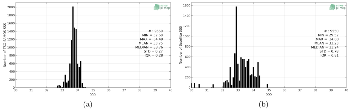
Figure 2: Histograms of SSS from TSG-SAMOS (a) and SMOS L3 v2 - Monthly - 0.25 Deg (CATDS-CECOS-IFREMER) (b) considering all match-up pairs per bins of 0.1 over the South China Sea Pi-MEP region and for the full satellite product period.
