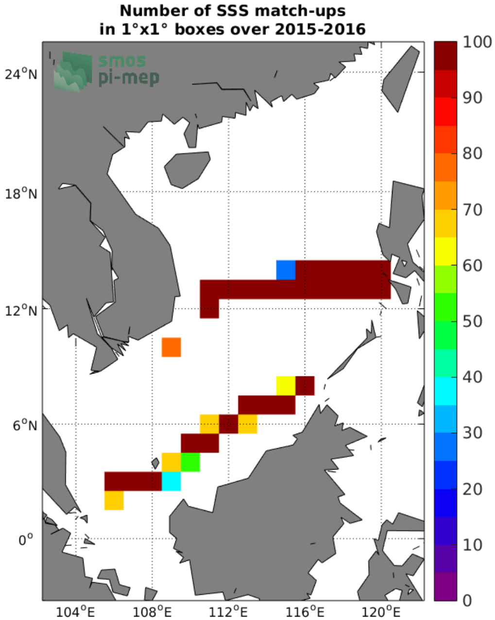
Figure 4: Number of SSS match-ups between TSG-SAMOS SSS and the SMOS-L3-CATDS-IFREMER-CECOS-V2-MONTHLY-0.25DEG SSS product for the South China Sea Pi-MEP region over 1°x1° boxes and for the full satellite product period.
