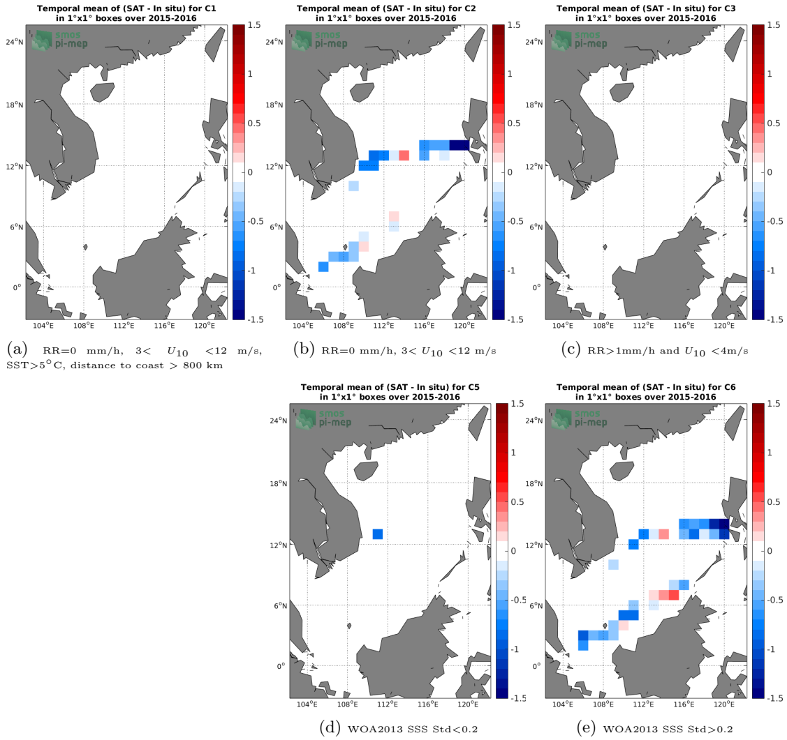
Figure 12: Temporal mean gridded over spatial boxes of size 1^\circ \times 1^\circ of \Delta SSS (SMOS-L3-CATDS-IFREMER-CECOS-V2-MONTHLY-0.25DEG - TSG-SAMOS) for 5 different subdatasets corresponding to:RR=0 mm/h, 3 < U_{10} < 12 m/s, SST>5°C, distance to coast > 800 km (a), RR=0 mm/h, 3 < U_{10} < 12 m/s (b), RR>1mm/h and U_{10} < 4 m/s (c), WOA2013 SSS Std<0.2 (d), WOA2013 SSS Std>0.2 (e).
