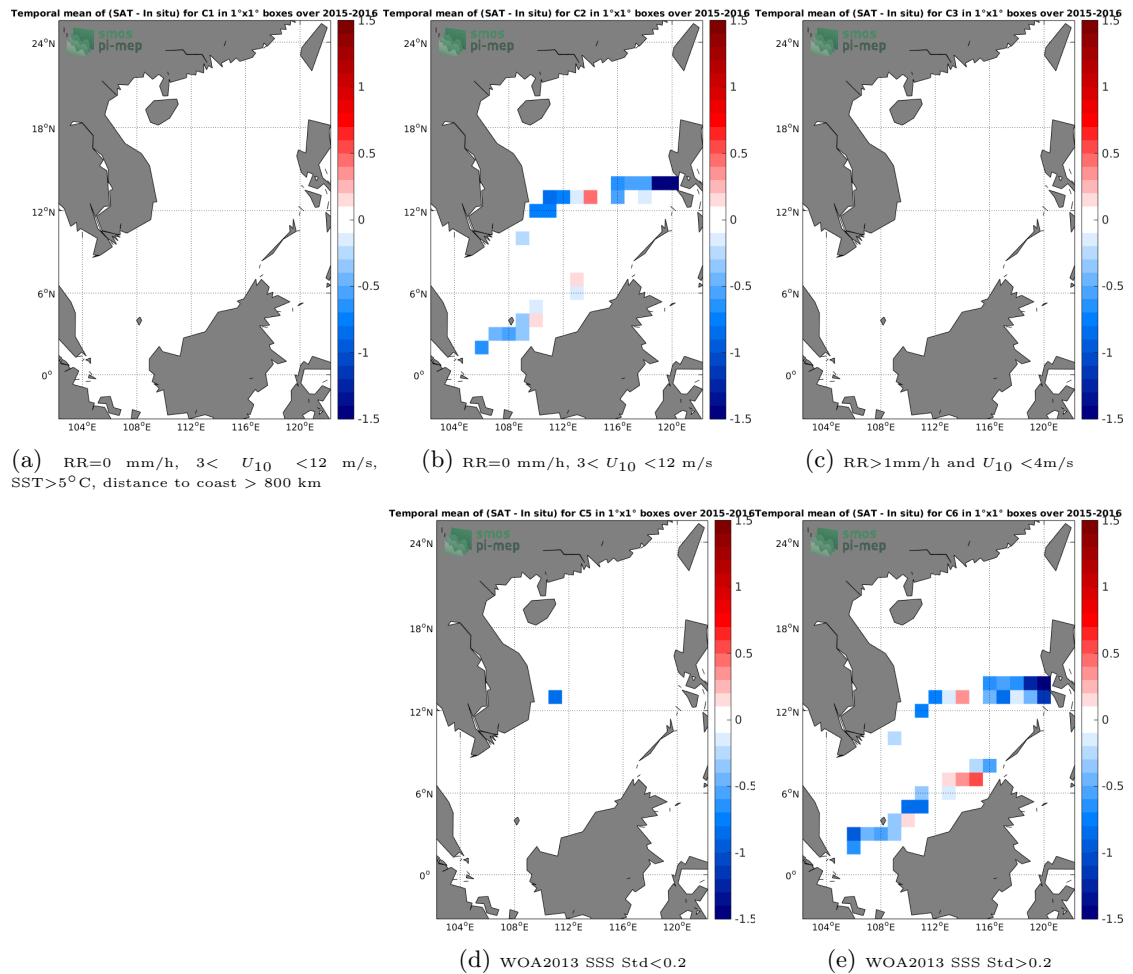
Figure 12: Temporal mean gridded over spatial boxes of size 1^\circ \times 1^\circ of \Delta SSS (SMOS-L3-CATDS-IFREMER-CECOS-V2-MONTHLY-0.25DEG - TSG-SAMOS) for 5 different subdatasets corresponding to:RR=0 mm/h, 3 < U_{10} < 12 m/s, SST > 5^\circ C, distance to coast > 800 km (a), RR=0 mm/h, 3 < U_{10} < 12 m/s (b), RR > 1 mm/h and U_{10} < 4 m/s (c), WOA2013 SSS Std < 0.2 (d), WOA2013 SSS Std > 0.2 (e).
