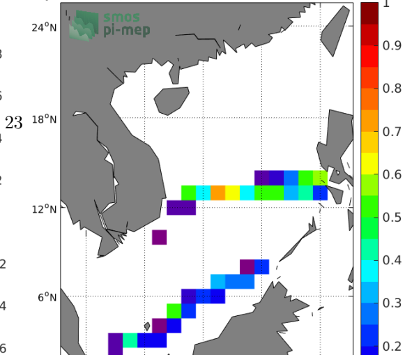
Temporal STD of (Sat-TSG-SAMOS) in 1°x1° boxes over 2015-2016
