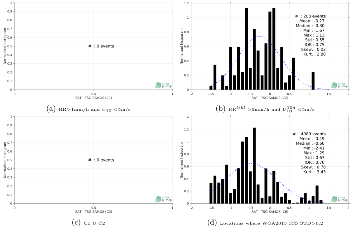
Figure 13: Normalized histogram of \Delta\text{SSS} (SMOS-L3-CATDS-IFREMER-CECOS-V2-MONTHLY-0.25DEG - TSG-SAMOS) for 6 different subdatasets corresponding to: RR > 1\text{mm/h} and U_{10} < 5\text{m/s} (a), RR^{10d} > 5\text{mm/h} and U_{10}^{10d} < 5\text{m/s} (b), C1 \cup C2 (c), Locations where WOA2013 SSS STD > 0.2 (d).
