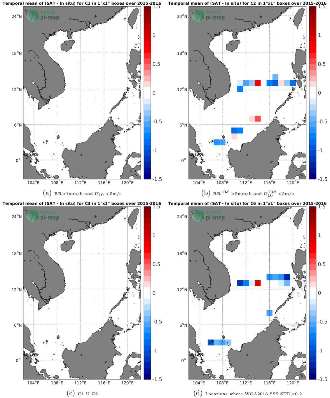
Figure 12: Temporal mean gridded over spatial boxes of size 1°x1° of \Delta\text{SSS} (SMOS-L3-CATDS-IFREMER-CECOS-V2-MONTHLY-0.25DEG - TSG-SAMOS) for 4 different subdatasets corresponding to: RR > 1\text{mm/h} and U_{10} < 5\text{m/s} (a), RR^{10d} > 5\text{mm/h} and U_{10}^{10d} < 5\text{m/s} (b), C1 U C2 (c), Locations where WOA2013 SSS STD > 0.2 (d).
