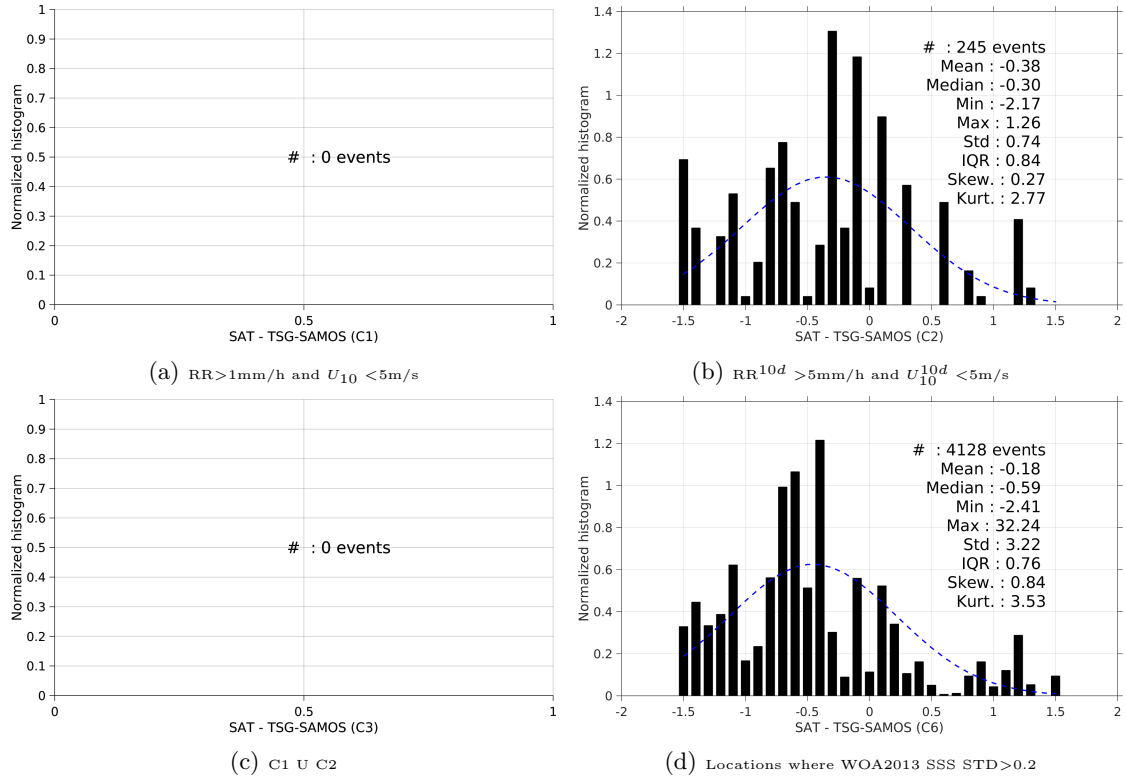
Figure 13: Normalized histogram of \Delta\text{SSS} (SMOS-L3-CATDS-IFREMER-CECOS-V2-MONTHLY-0.25DEG - TSG-SAMOS) for 6 different subdatasets corresponding to: RR > 1\text{mm/h} and U_{10} < 5\text{m/s} (a), RR^{10d} > 5\text{mm/h} and U_{10}^{10d} < 5\text{m/s} (b), C1 \cup C2 (c), Locations where WOA2013 SSS STD > 0.2 (d).
