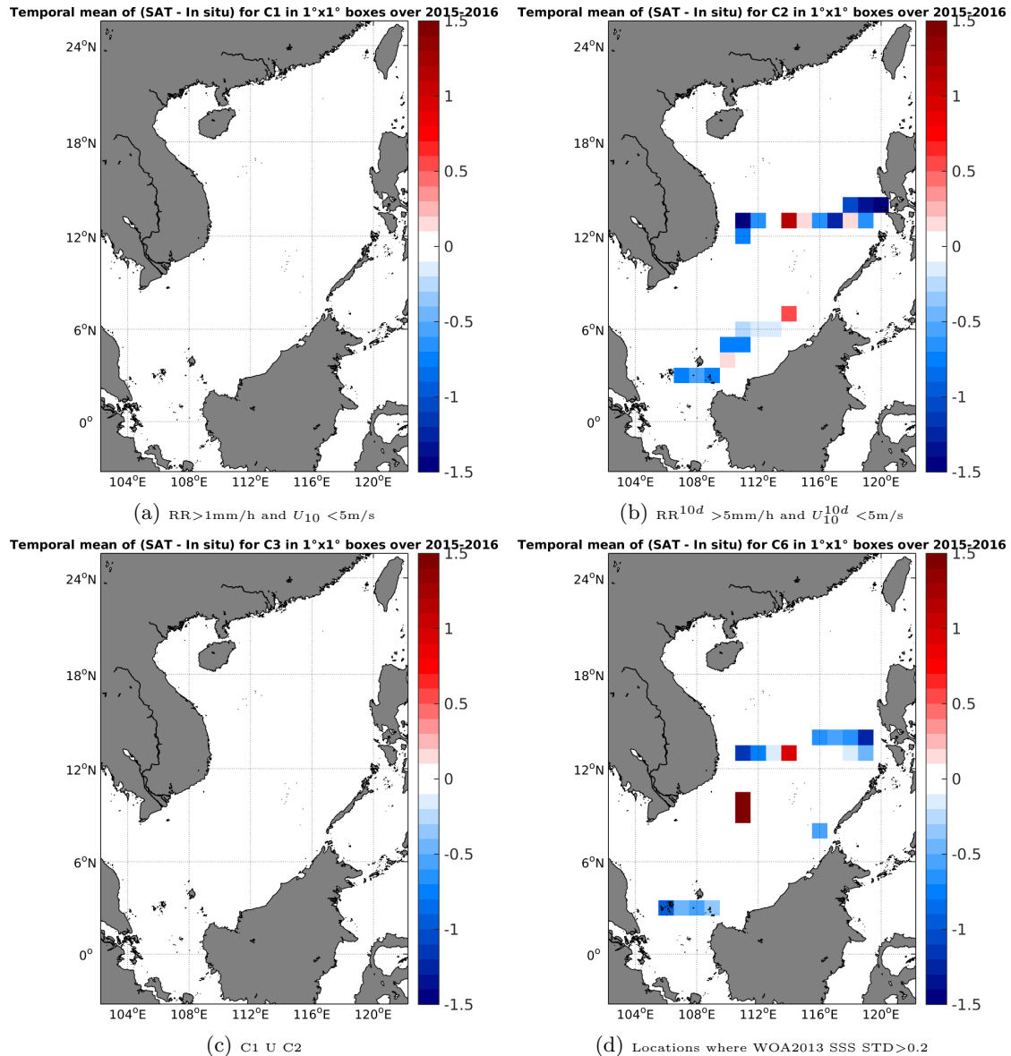
Figure 12: Temporal mean gridded over spatial boxes of size 1^\circ \times 1^\circ of \Delta SSS (SMOS-L3-CATDS-IFREMER-CECOS-V2-MONTHLY-0.25DEG - TSG-SAMOS) for 4 different subdatasets corresponding to: RR > 1\text{mm/h} and U_{10} < 5\text{m/s} (a), RR^{10d} > 5\text{mm/h} and U_{10}^{10d} < 5\text{m/s} (b), C1 U C2 (c), Locations where WOA2013 SSS STD > 0.2 (d).
