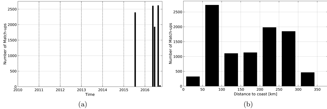
Figure 1: Number of match-ups between TSG-SAMOS and SMOS-L3-CATDS-IFREMER-CECOS-V2-MONTHLY-0.25DEG SSS as a function of time (a) and as function of the distance to coast (b) over the South China Sea Pi-MEP region and for the full satellite product period.
