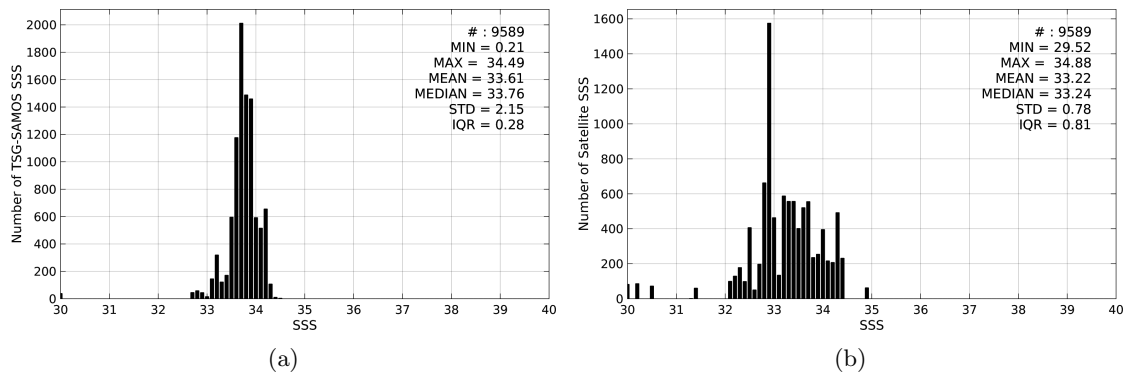
Figure 2: Histograms of SSS from TSG-SAMOS (a) and SMOS-L3-CATDS-IFREMER-CECOS-V2-MONTHLY-0.25DEG (b) considering all match-up pairs per bins of 0.1 over the South China Sea Pi-MEP region and for the full satellite product period.
