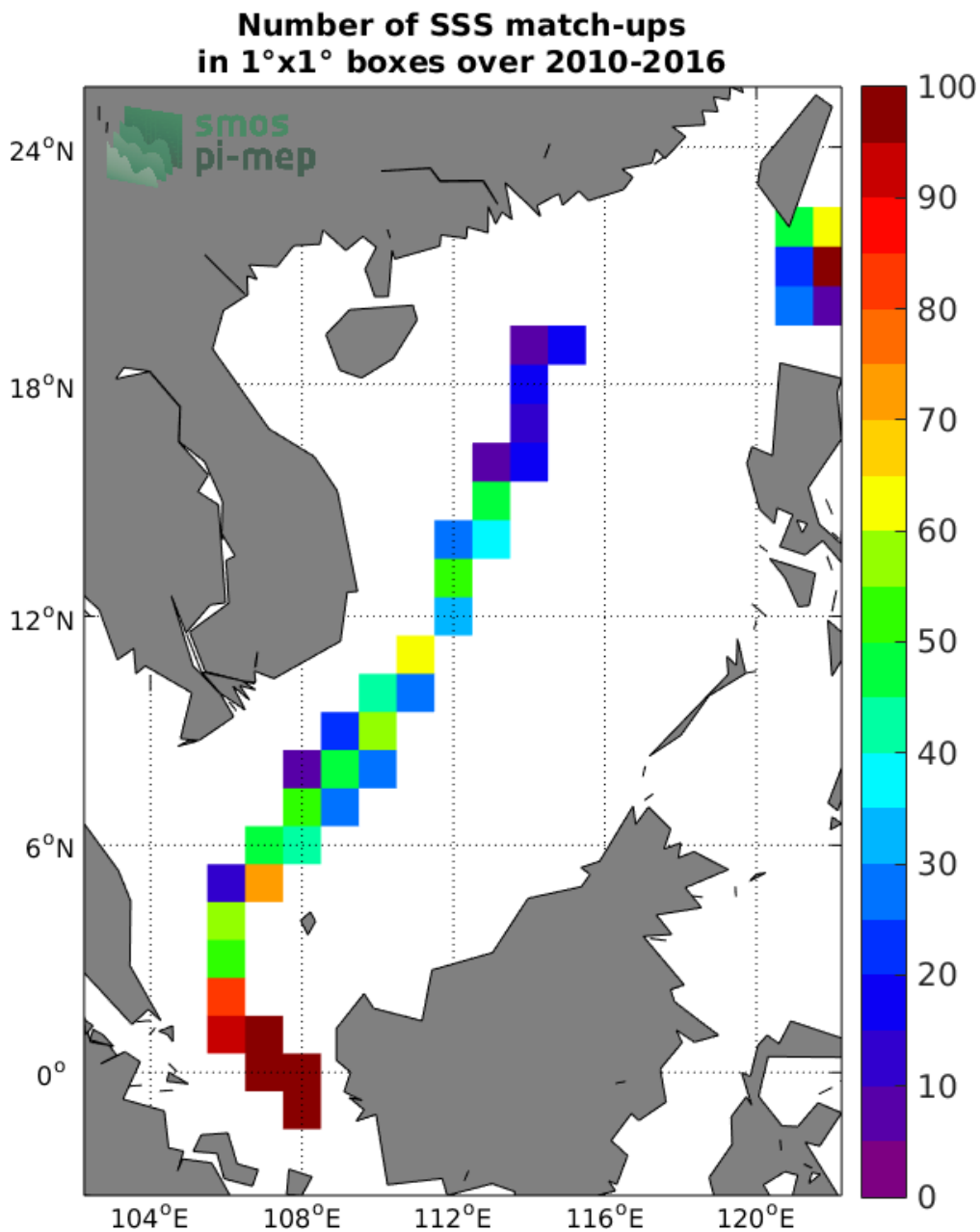
Figure 4: Number of SSS match-ups between TSG (LEGOS-DM) SSS and the SMOS SSS L3 v2 - Monthly - 0.25 Deg (CATDS-CECOS-IFREMER) SSS product for the South China Sea Pi-MEP region over 1°x1° boxes and for the full satellite product period.
