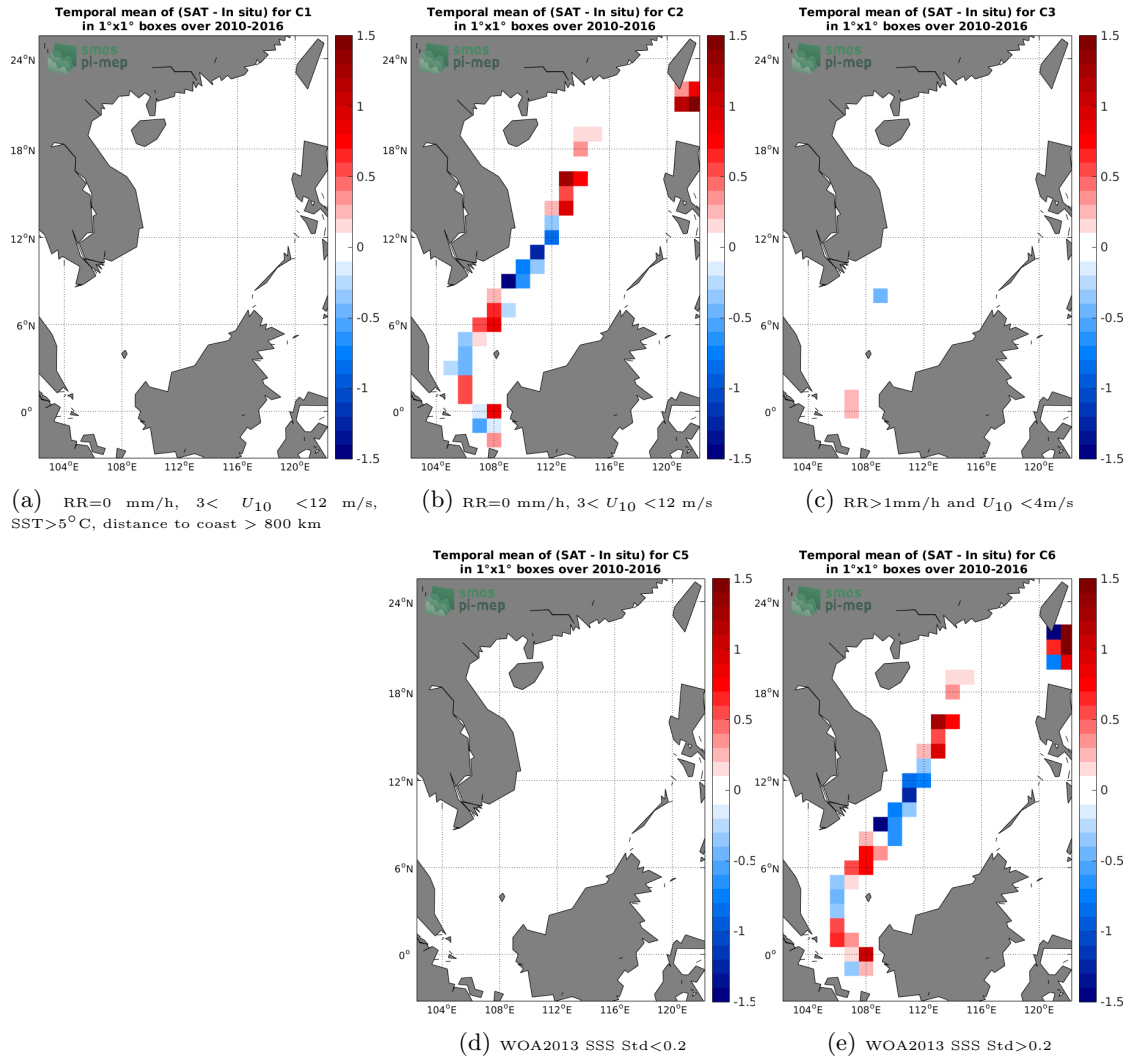
Figure 12: Temporal mean gridded over spatial boxes of size 1^\circ \times 1^\circ of \Delta\text{SSS} (SMOS SSS L3 v2 - Monthly - 0.25 Deg (CATDS-CECOS-IFREMER) - TSG (LEGOS-DM)) for 5 different subdatasets corresponding to: RR=0 mm/h, 3 < U_{10} < 12 m/s, SST > 5^\circ\text{C} , distance to coast > 800 km (a), RR=0 mm/h, 3 < U_{10} < 12 m/s (b), RR > 1\text{mm/h} and U_{10} < 4\text{m/s} (c), WOA2013 SSS Std < 0.2 (d), WOA2013 SSS Std > 0.2 (e).
