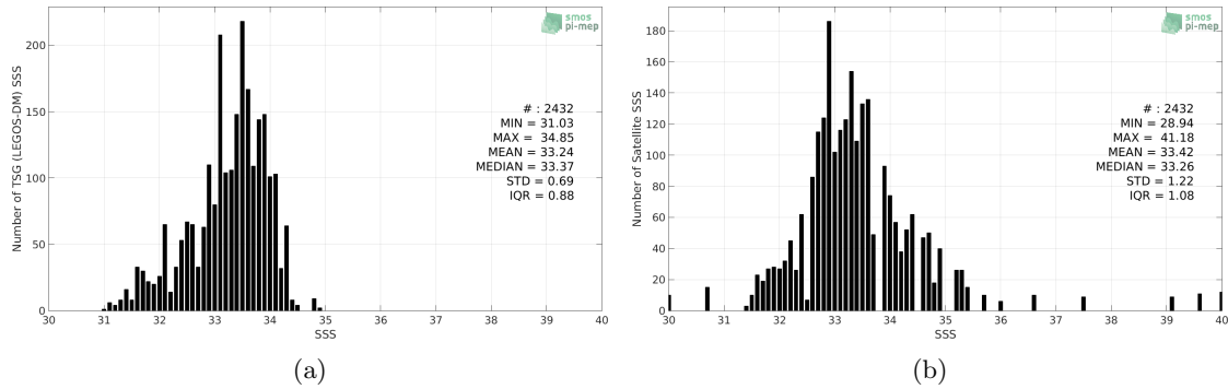
Figure 2: Histograms of SSS from TSG (LEGOS-DM) (a) and SMOS SSS L3 v2 - Monthly - 0.25 Deg (CATDS-CECOS-IFREMER) (b) considering all match-up pairs per bins of 0.1 over the South China Sea Pi-MEP region and for the full satellite product period.
