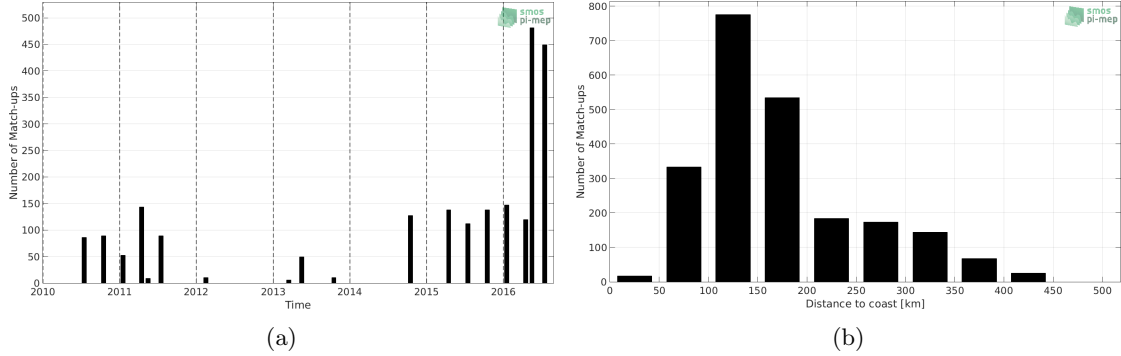
Figure 1: Number of match-ups between TSG-LEGOS-DM and SMOS-L3-CATDS-IFREMER-CECOS-V2-MONTHLY-0.25DEG SSS as a function of time (a) and as function of the distance to coast (b) over the South China Sea Pi-MEP region and for the full satellite product period.
