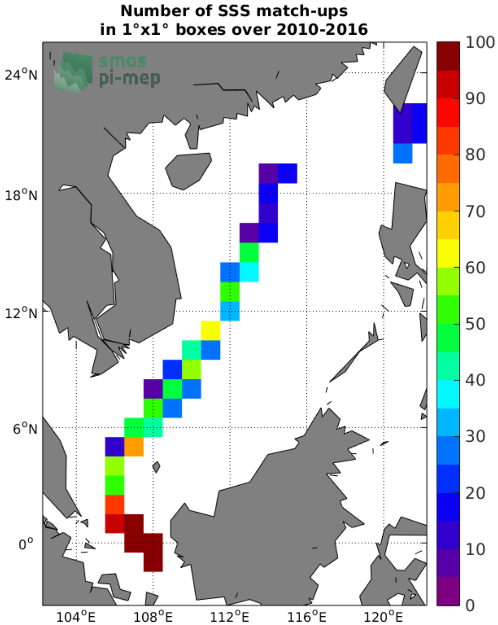
Figure 4: Number of SSS match-ups between TSG-LEGOS-DM SSS and the SMOS-L3-CATDS-IFREMER-CECOS-V2-MONTHLY-0.25DEG SSS product for the South China Sea Pi-MEP region over 1°x1° boxes and for the full satellite product period.
