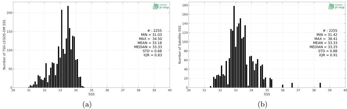
Figure 2: Histograms of SSS from TSG-LEGOS-DM (a) and SMOS-L3-CATDS-IFREMER-CECOS-V2-MONTHLY-0.25DEG (b) considering all match-up pairs per bins of 0.1 over the South China Sea Pi-MEP region and for the full satellite product period.
