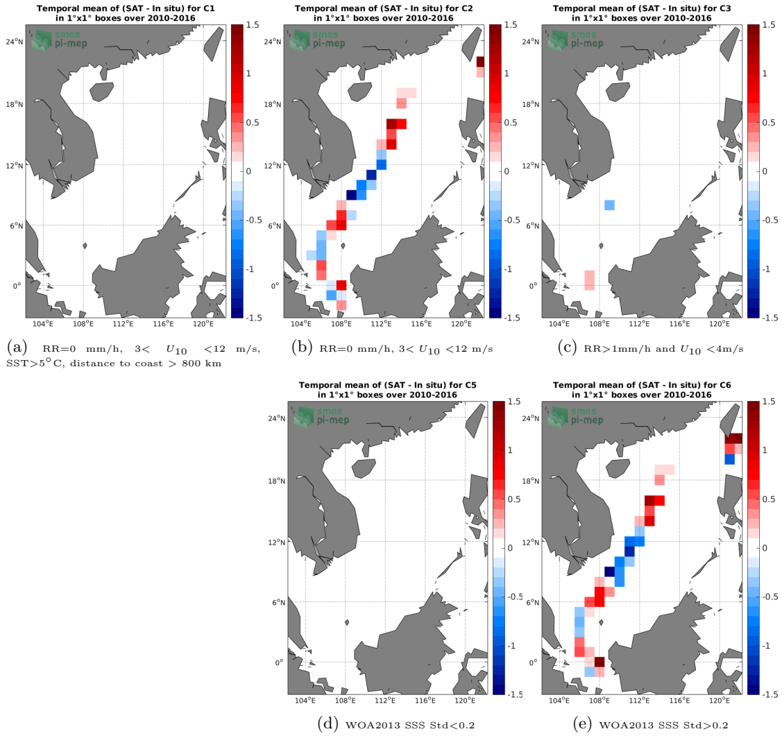
Figure 12: Temporal mean gridded over spatial boxes of size 1°x1° of \Delta SSS (SMOS-L3-CATDS-IFREMER-CECOS-V2-MONTHLY-0.25DEG - TSG-LEGOS-DM) for 5 different subdatasets corresponding to:RR=0 mm/h, 3 < U_{10} < 12 m/s, SST>5°C, distance to coast > 800 km (a), RR=0 mm/h, 3 < U_{10} < 12 m/s (b), RR>1mm/h and U_{10} < 4 m/s (c), WOA2013 SSS Std<0.2 (d), WOA2013 SSS Std>0.2 (e).
