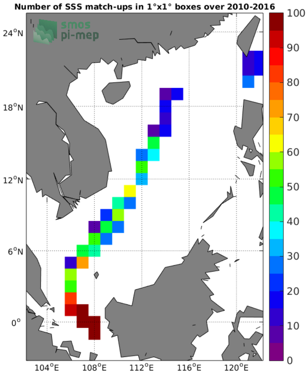
Figure 4: Number of SSS match-ups between TSG-LEGOS-DM SSS and the SMOS-L3-CATDS-IFREMER-CECOS-V2-MONTHLY-0.25DEG SSS product for the South China Sea Pi-MEP region over 1°x1° boxes and for the full satellite product period.
