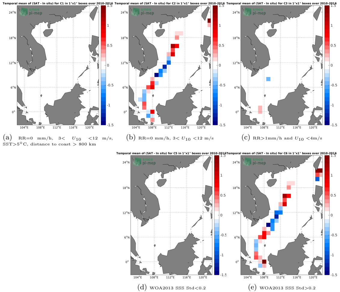
Figure 12: Temporal mean gridded over spatial boxes of size 1^\circ \times 1^\circ of \Delta SSS (SMOS-L3-CATDS-IFREMER-CECOS-V2-MONTHLY-0.25DEG - TSG-LEGOS-DM) for 5 different subdatasets corresponding to:RR=0 mm/h, 3 < U_{10} < 12 m/s, SST >5^\circ C, distance to coast > 800 km (a), RR=0 mm/h, 3 < U_{10} < 12 m/s (b), RR >1 mm/h and U_{10} < 4 m/s (c), WOA2013 SSS Std <0.2 (d), WOA2013 SSS Std >0.2 (e).
