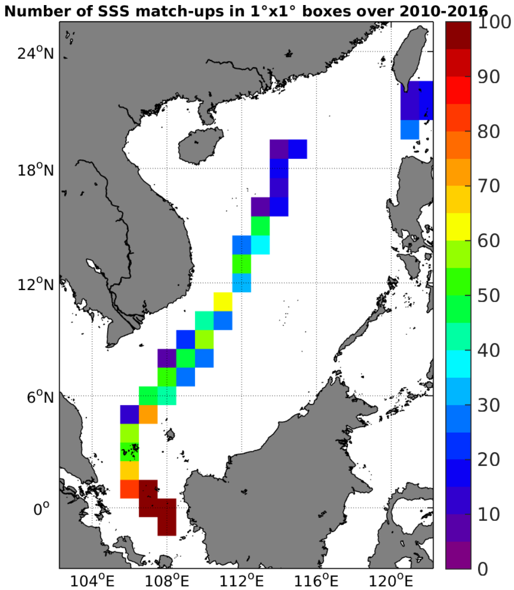
Figure 4: Number of SSS match-ups between TSG-LEGOS-DM SSS and the SMOS-L3-CATDS-IFREMER-CECOS-V2-MONTHLY-0.25DEG SSS product for the South China Sea Pi-MEP region over 1°x1° boxes and for the full satellite product period.
