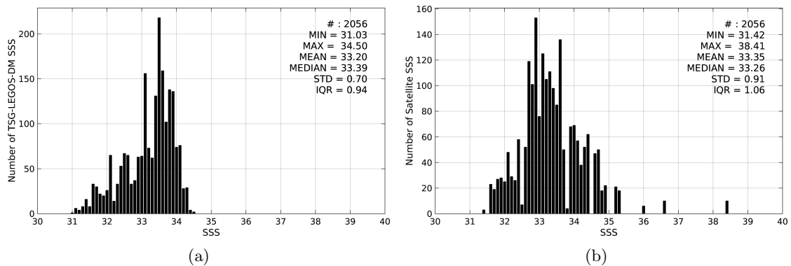
Figure 2: Histograms of SSS from TSG-LEGOS-DM (a) and SMOS-L3-CATDS-IFREMER-CECOS-V2-MONTHLY-0.25DEG (b) considering all match-up pairs per bins of 0.1 over the South China Sea Pi-MEP region and for the full satellite product period.
