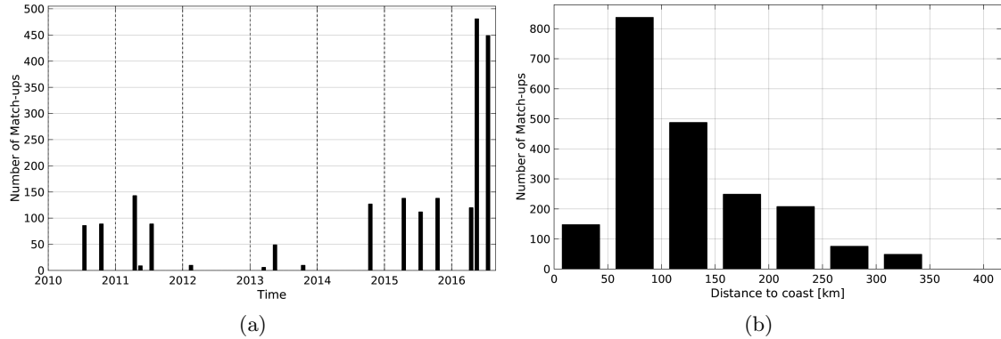
Figure 1: Number of match-ups between TSG-LEGOS-DM and SMOS-L3-CATDS-IFREMER-CECOS-V2-MONTHLY-0.25DEG SSS as a function of time (a) and as function of the distance to coast (b) over the South China Sea Pi-MEP region and for the full satellite product period.
