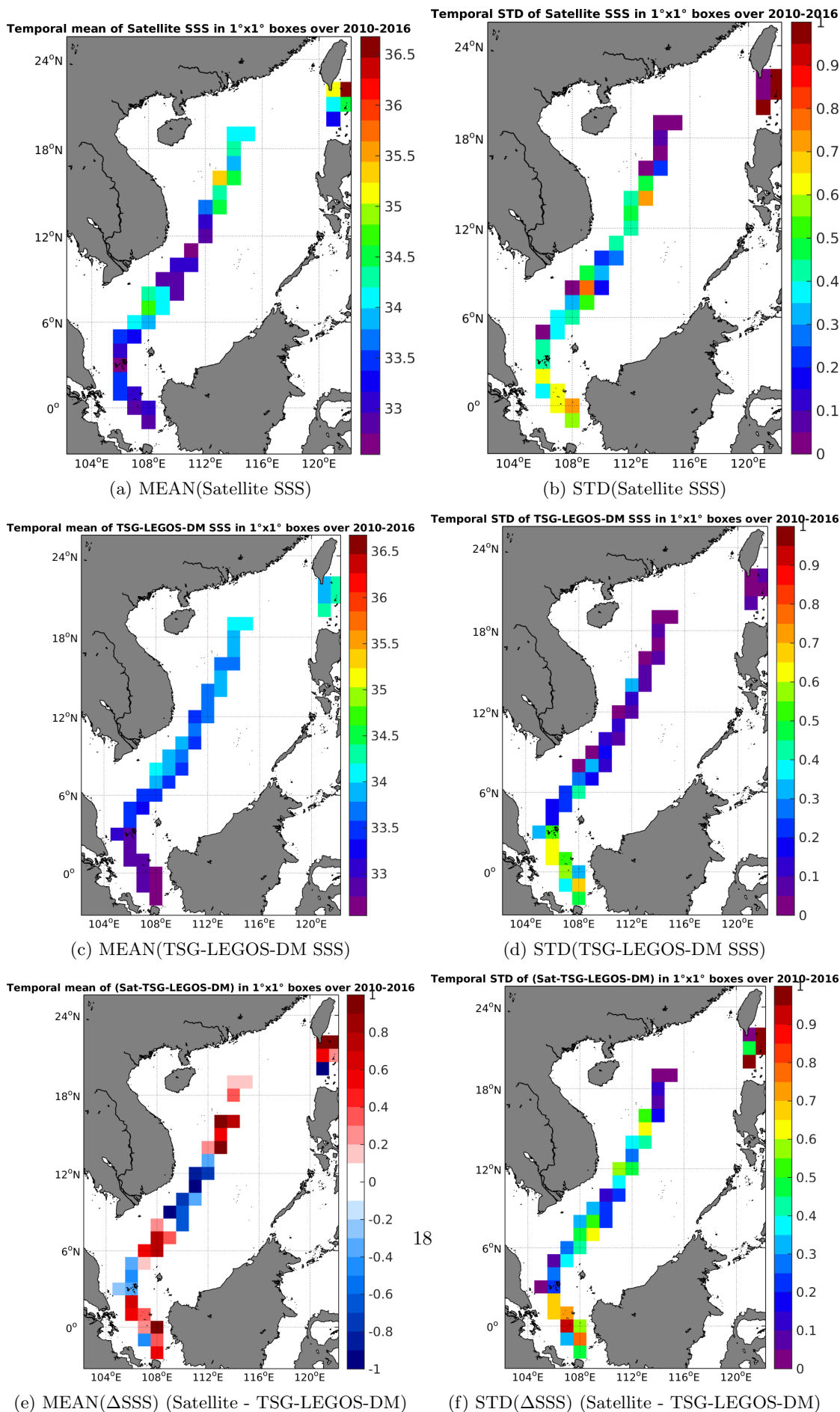
Figure 6: Temporal mean (left) and STD (right) of SSS from SMOS-L3-CATDS-IFREMER-CECOS-V2-MONTHLY-0.25DEG (top), TSG-LEGOS-DM (middle), and of \Delta SSS (Satellite - TSG-LEGOS-DM). Only match-up pairs are used to generate these maps.
