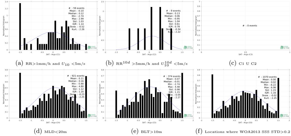
Figure 13: Normalized histogram of \Delta SSS (SMOS-L3-CATDS-IFREMER-CECOS-V2-MONTHLY-0.25DEG - Argo) for 6 different subdatasets corresponding to: RR > 1\text{mm/h} and U_{10} < 5\text{m/s} (a), RR^{10d} > 5\text{mm/h} and U_{10}^{10d} < 5\text{m/s} (b), C1 U C2 (c), MLD < 20\text{m} (d), BLT > 10\text{m} (e), Locations where WOA2013 SSS STD > 0.2 (f).
