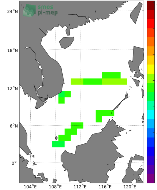
(c) MEAN(TSG-SAMOS SSS)
