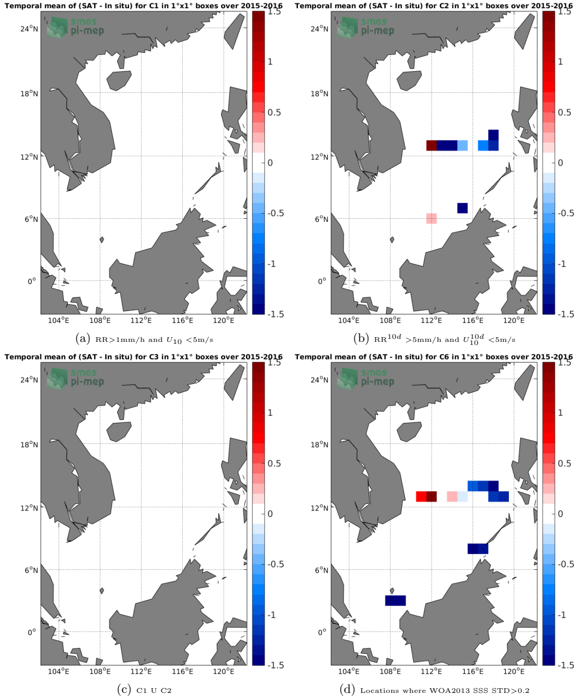
Figure 12: Temporal mean gridded over spatial boxes of size 1°x1° of \Delta\text{SSS} (SMOS-L3-CATDS-CECOS-IFREMER-V2-1DAY-0.5DEG - TSG-SAMOS) for 4 different subdatasets corresponding to: RR > 1\text{mm/h} and U_{10} < 5\text{m/s} (a), RR^{10d} > 5\text{mm/h} and U_{10}^{10d} < 5\text{m/s} (b), C1 U C2 (c), Locations where WOA2013 SSS STD > 0.2 (d).
