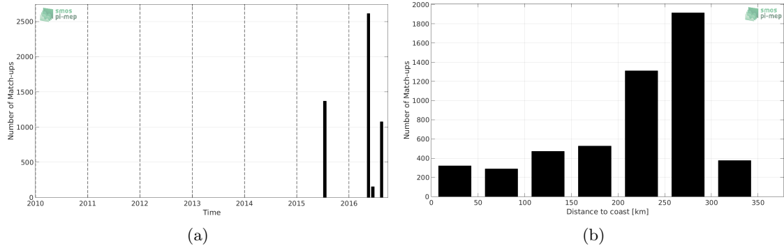
Figure 1: Number of match-ups between TSG-SAMOS and SMOS-L3-CATDS-CECOS-IFREMER-V2-1DAY-0.5DEG SSS as a function of time (a) and as function of the distance to coast (b) over the South China Sea Pi-MEP region and for the full satellite product period.
