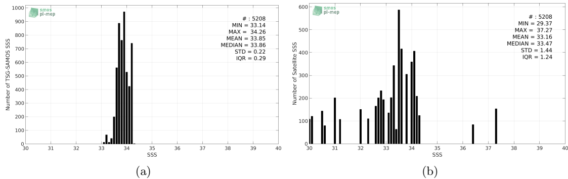
Figure 2: Histograms of SSS from TSG-SAMOS (a) and SMOS-L3-CATDS-CECOS-IFREMER-V2-1DAY-0.5DEG (b) considering all match-up pairs per bins of 0.1 over the South China Sea Pi-MEP region and for the full satellite product period.
