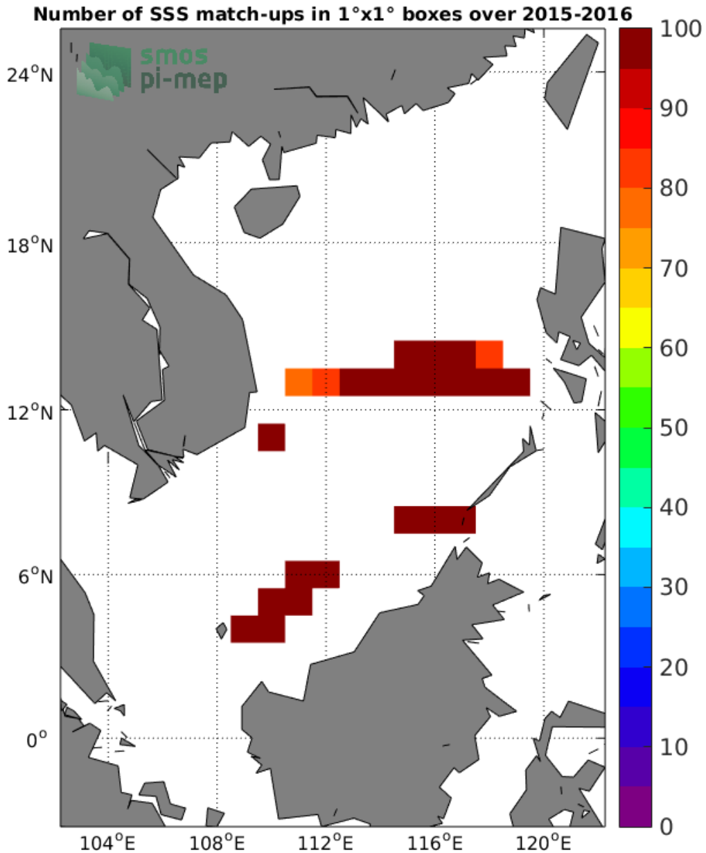
Figure 4: Number of SSS match-ups between TSG-SAMOS SSS and the SMOS-L3-CATDS-CECOS-IFREMER-V2-1DAY-0.5DEG SSS product for the South China Sea Pi-MEP region over 1°x1° boxes and for the full satellite product period.
