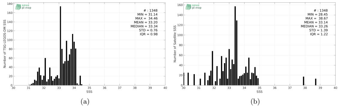
Figure 2: Histograms of SSS from TSG-LEGOS-DM (a) and SMOS-L3-CATDS-CECOS-IFREMER-V2-1DAY-0.5DEG (b) considering all match-up pairs per bins of 0.1 over the South China Sea Pi-MEP region and for the full satellite product period.
