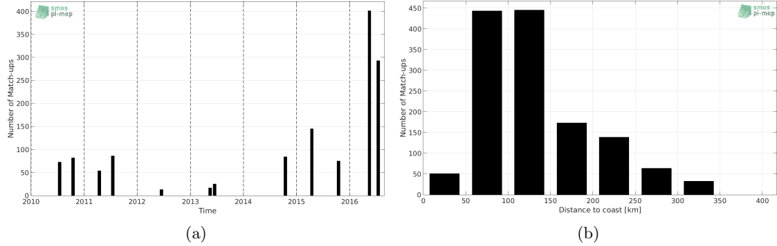
Figure 1: Number of match-ups between TSG-LEGOS-DM and SMOS-L3-CATDS-CECOS-IFREMER-V2-1DAY-0.5DEG SSS as a function of time (a) and as function of the distance to coast (b) over the South China Sea Pi-MEP region and for the full satellite product period.
