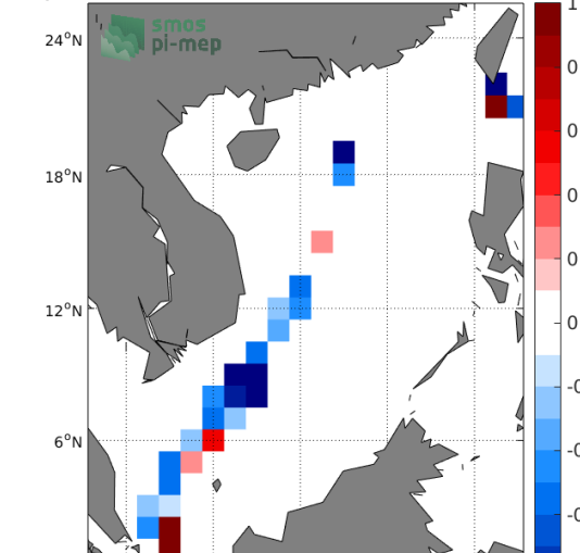
Temporal mean of (Sat-TSG-LEGOS-DM) in 1°x1° boxes over 2010-2016
