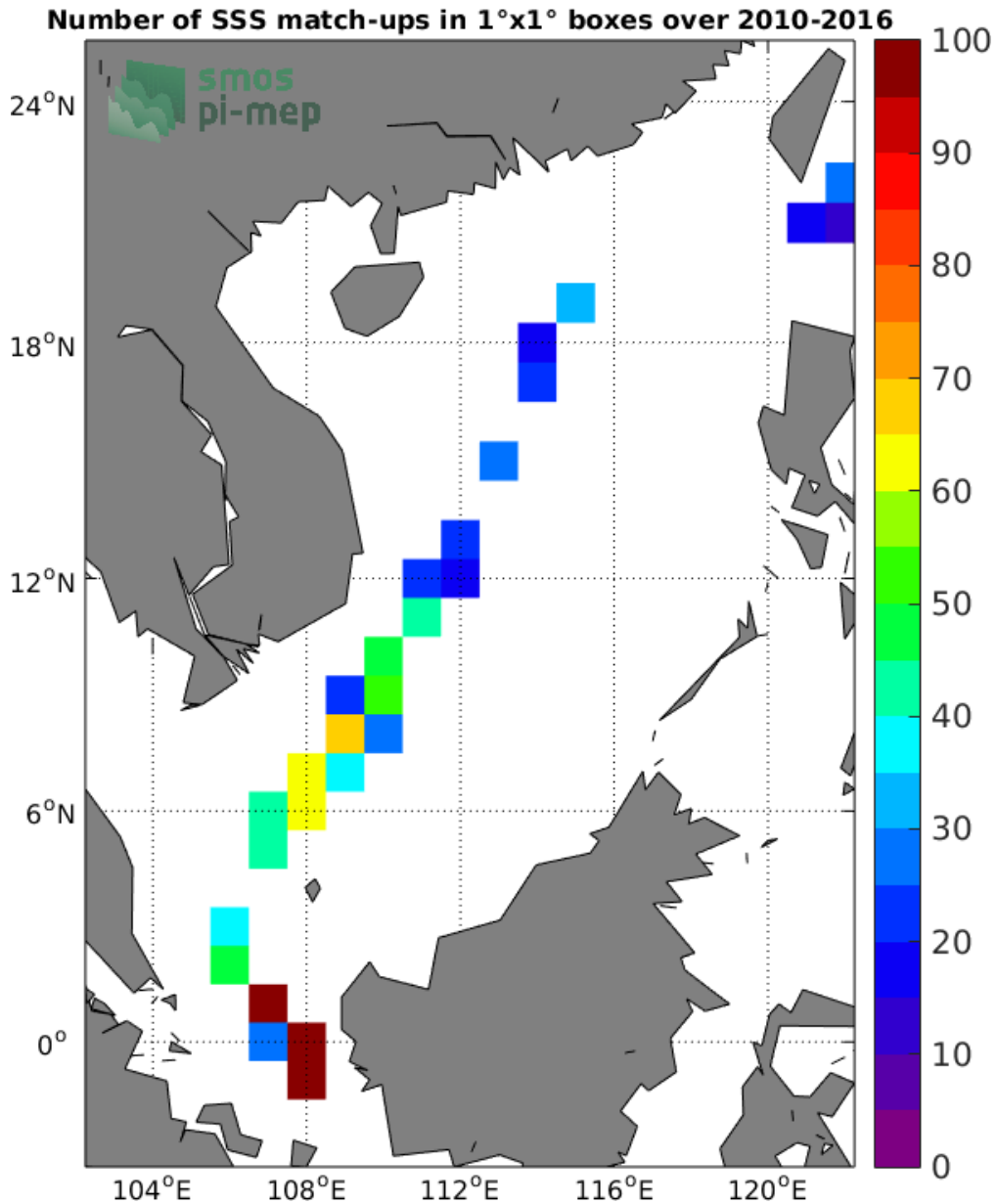
Figure 4: Number of SSS match-ups between TSG-LEGOS-DM SSS and the SMOS-L3-CATDS-CECOS-IFREMER-V2-1DAY-0.5DEG SSS product for the South China Sea Pi-MEP region over 1°x1° boxes and for the full satellite product period.
