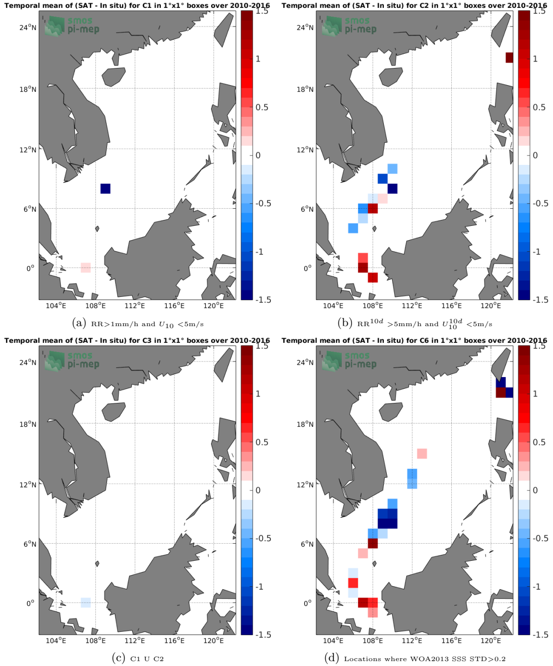
Figure 12: Temporal mean gridded over spatial boxes of size 1°x1° of \Delta\text{SSS} (SMOS-L3-CATDS-CECOS-IFREMER-V2-1DAY-0.5DEG - TSG-LEGOS-DM) for 4 different subdatasets corresponding to: RR > 1\text{mm/h} and U_{10} < 5\text{m/s} (a), RR^{10d} > 5\text{mm/h} and U_{10}^{10d} < 5\text{m/s} (b), C1 U C2 (c), Locations where WOA2013 SSS STD > 0.2 (d).
