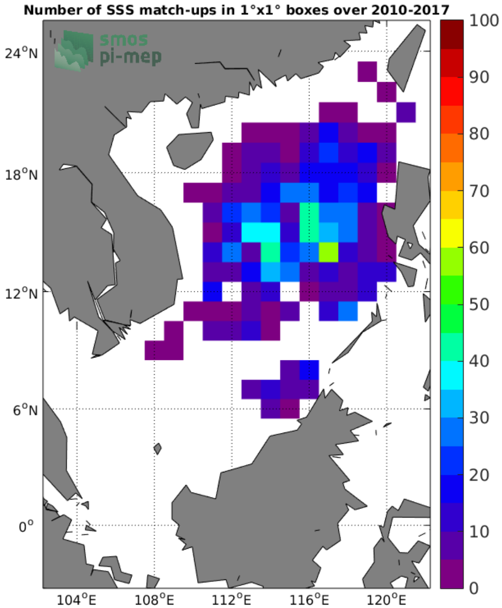
Figure 4: Number of SSS match-ups between Argo SSS and the SMOS-L3-CATDS-CECOS-IFREMER-V2-1DAY-0.5DEG SSS product for the South China Sea Pi-MEP region over 1°x1° boxes and for the full satellite product period.
