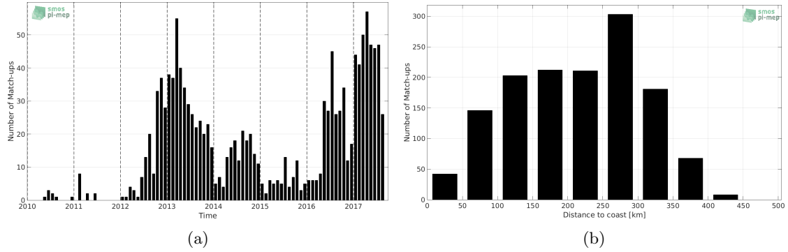
Figure 1: Number of match-ups between Argo and SMOS-L3-CATDS-CECOS-IFREMER-V2-1DAY-0.5DEG SSS as a function of time (a) and as function of the distance to coast (b) over the South China Sea Pi-MEP region and for the full satellite product period.
