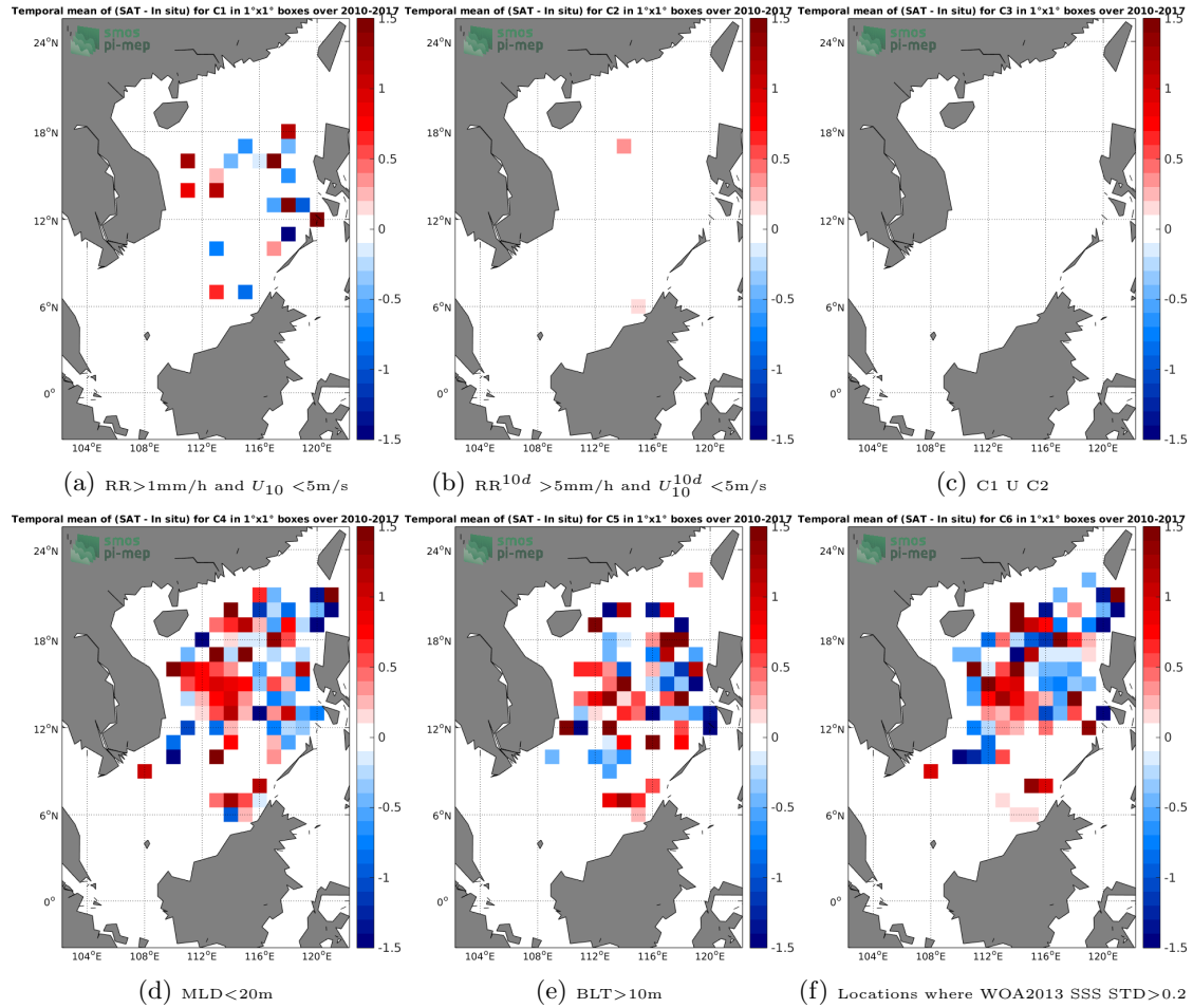
Figure 12: Temporal mean gridded over spatial boxes of size 1^\circ \times 1^\circ of \Delta\text{SSS} (SMOS-L3-CATDS-CECOS-IFREMER-V2-1DAY-0.5DEG - Argo) for 6 different subdatasets corresponding to: RR >1\text{mm/h} and U_{10} <5\text{m/s} (a), \text{RR}^{10d} >5\text{mm/h} and U_{10}^{10d} <5\text{m/s} (b), C1 U C2 (c), \text{MLD} <20\text{m} (d), \text{BLT} >10\text{m} (e), Locations where WOA2013 SSS STD >0.2 (f).
