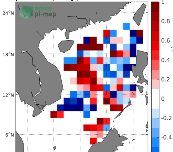
Temporal mean of (Sat-Argo) in 1°x1° boxes over 2010-2017
