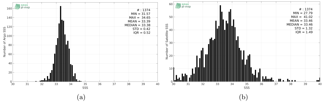
Figure 2: Histograms of SSS from Argo (a) and SMOS-L3-CATDS-CECOS-IFREMER-V2-1DAY-0.5DEG (b) considering all match-up pairs per bins of 0.1 over the South China Sea Pi-MEP region and for the full satellite product period.
