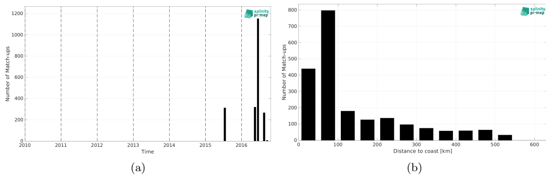
Figure 1: Number of match-ups between TSG (SAMOS) and SMOS SSS L3 v335 - Monthly - 25 km (CATDS-CPDC) SSS as a function of time (a) and as function of the distance to coast (b) over the South China Sea Pi-MEP region and for the full satellite product period.
