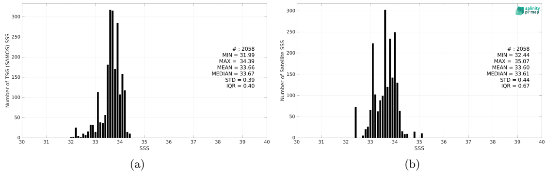
Figure 2: Histograms of SSS from TSG (SAMOS) (a) and SMOS SSS L3 v335 - Monthly - 25 km (CATDS-CPDC) (b) considering all match-up pairs per bins of 0.1 over the South China Sea Pi-MEP region and for the full satellite product period.
