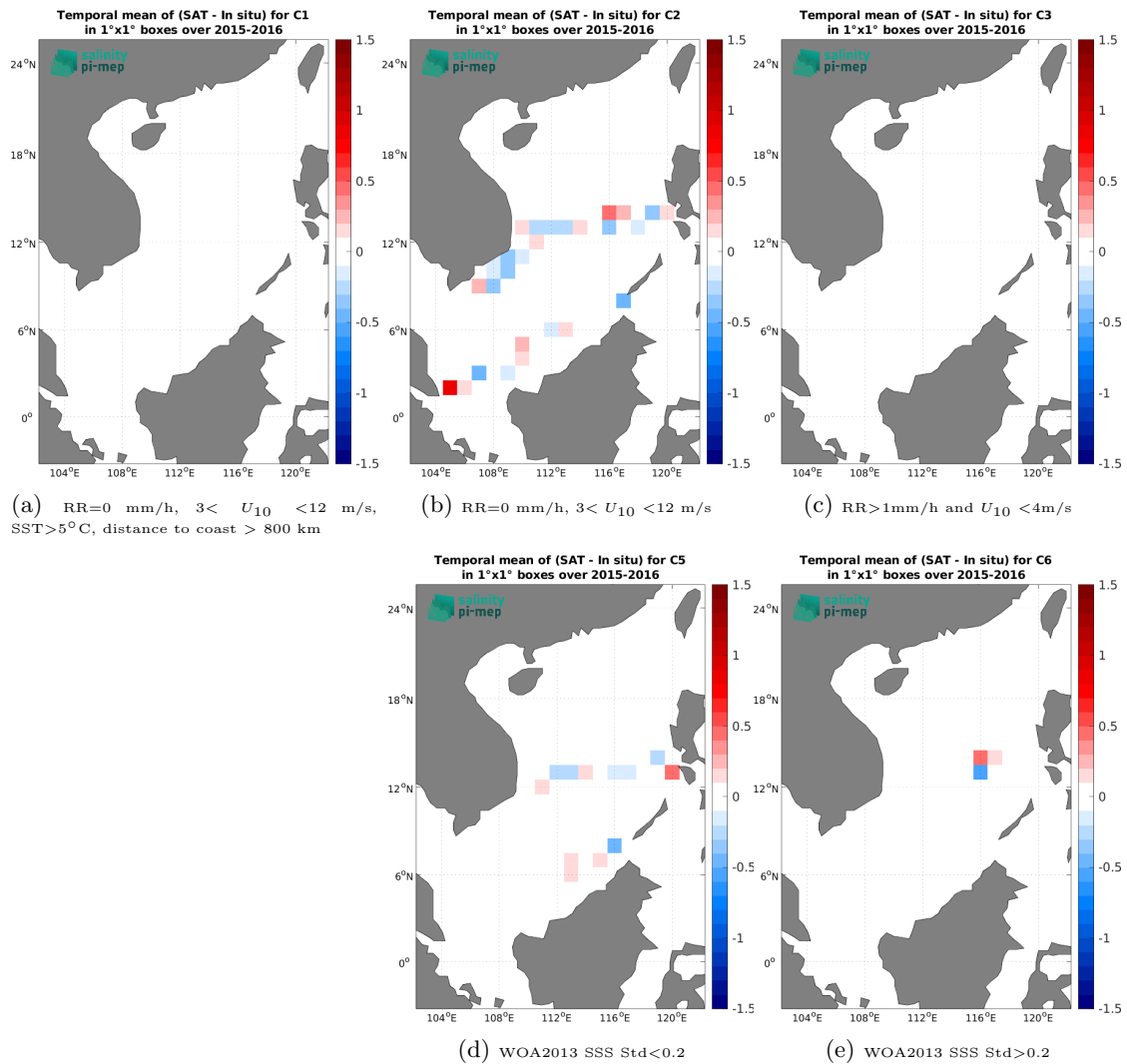
Figure 12: Temporal mean gridded over spatial boxes of size 1^\circ \times 1^\circ of \Delta SSS (SMOS SSS L3 v335 - Monthly - 25 km (CATDS-CPDC) - TSG (SAMOS)) for 5 different subdatasets corresponding to:RR=0 mm/h, 3 < U_{10} < 12 m/s, SST>5°C, distance to coast > 800 km (a), RR=0 mm/h, 3 < U_{10} < 12 m/s (b), RR>1mm/h and U_{10} < 4 m/s (c), WOA2013 SSS Std<0.2 (d), WOA2013 SSS Std>0.2 (e).
