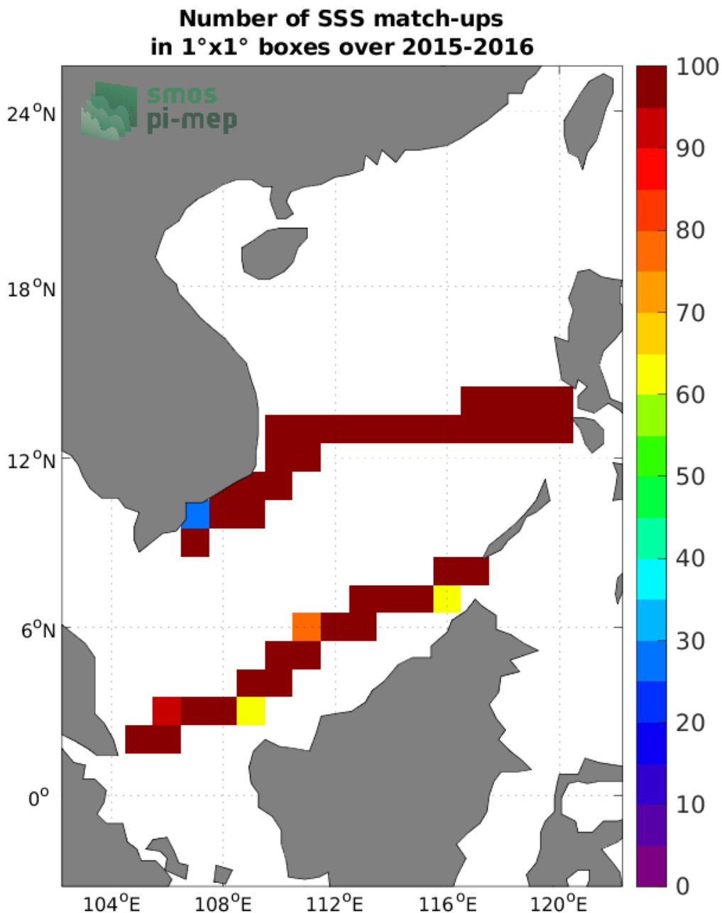
Figure 4: Number of SSS match-ups between TSG (SAMOS) SSS and the SMOS SSS L3 v335 - Monthly - 25 km (CATDS-CPDC) SSS product for the South China Sea Pi-MEP region over 1°x1° boxes and for the full satellite product period.
