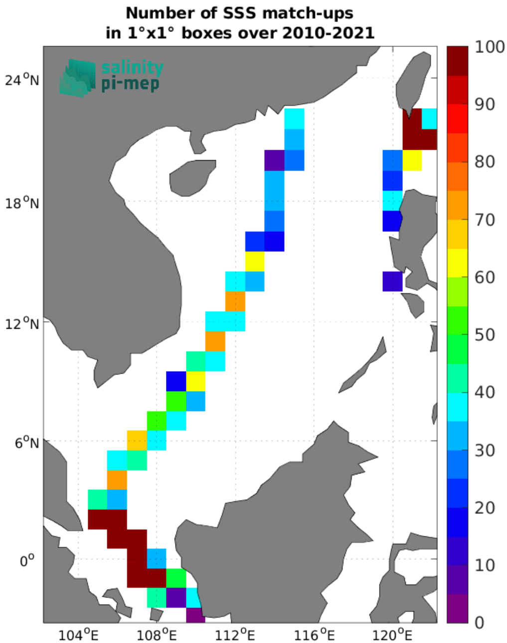
Figure 5: Number of SSS match-ups between TSG (LEGOS-DM) SSS and the SMOS SSS L3 v335 - Monthly - 25 km (CATDS-CPDC) SSS product for the South China Sea Pi-MEP region over 1^\circ \times 1^\circ boxes and for the full satellite product period.
