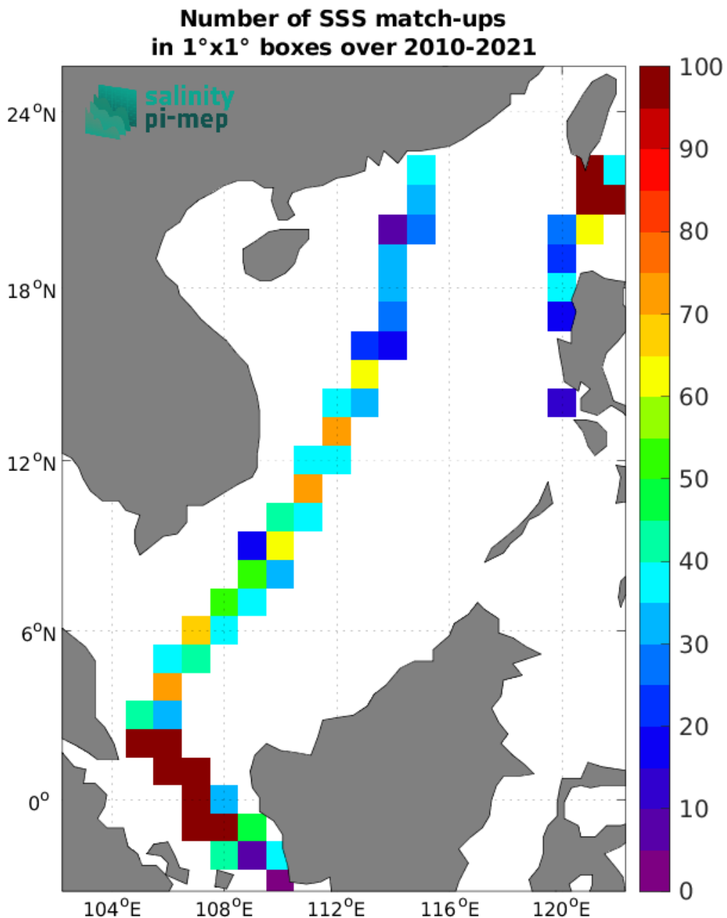
Figure 5: Number of SSS match-ups between TSG (LEGOS-DM) SSS and the SMOS SSS L3 v335 - Monthly - 25 km (CATDS-CPDC) SSS product for the South China Sea Pi-MEP region over 1°×1° boxes and for the full satellite product period.
