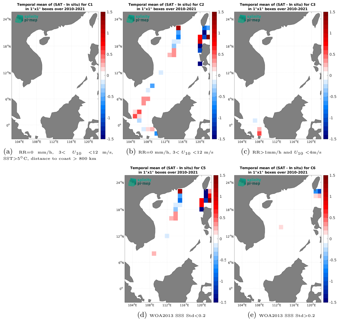
Figure 14: Temporal mean gridded over spatial boxes of size 1^\circ \times 1^\circ of \Delta SSS (SMOS SSS L3 v335 - Monthly - 25 km (CATDS-CPDC) - TSG (LEGOS-DM)) for 5 different subdatasets corresponding to:RR=0 mm/h, 3 < U_{10} < 12 m/s, SST>5°C, distance to coast > 800 km (a), RR=0 mm/h, 3 < U_{10} < 12 m/s (b), RR>1mm/h and U_{10} < 4 m/s (c), WOA2013 SSS Std<0.2 (d), WOA2013 SSS Std>0.2 (e).
