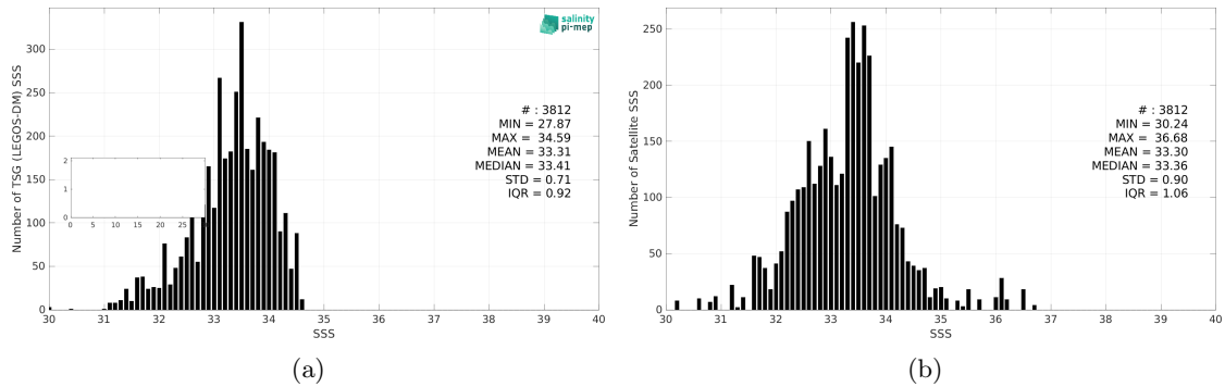
Figure 3: Histograms of SSS from TSG (LEGOS-DM) (a) and SMOS SSS L3 v335 - Monthly - 25 km (CATDS-CPDC) (b) considering all match-up pairs per bins of 0.1 over the South China Sea Pi-MEP region and for the full satellite product period.
