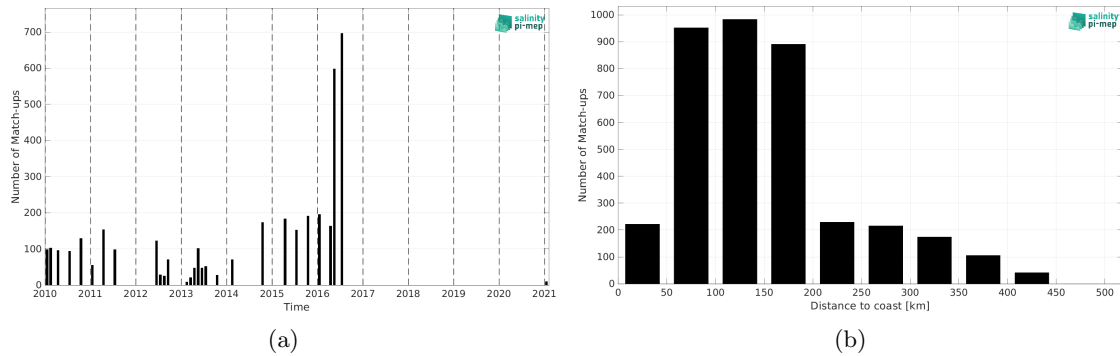
Figure 2: Number of match-ups between TSG (LEGOS-DM) and SMOS SSS L3 v335 - Monthly - 25 km (CATDS-CPDC) SSS as a function of time (a) and as function of the distance to coast (b) over the South China Sea Pi-MEP region and for the full satellite product period.
