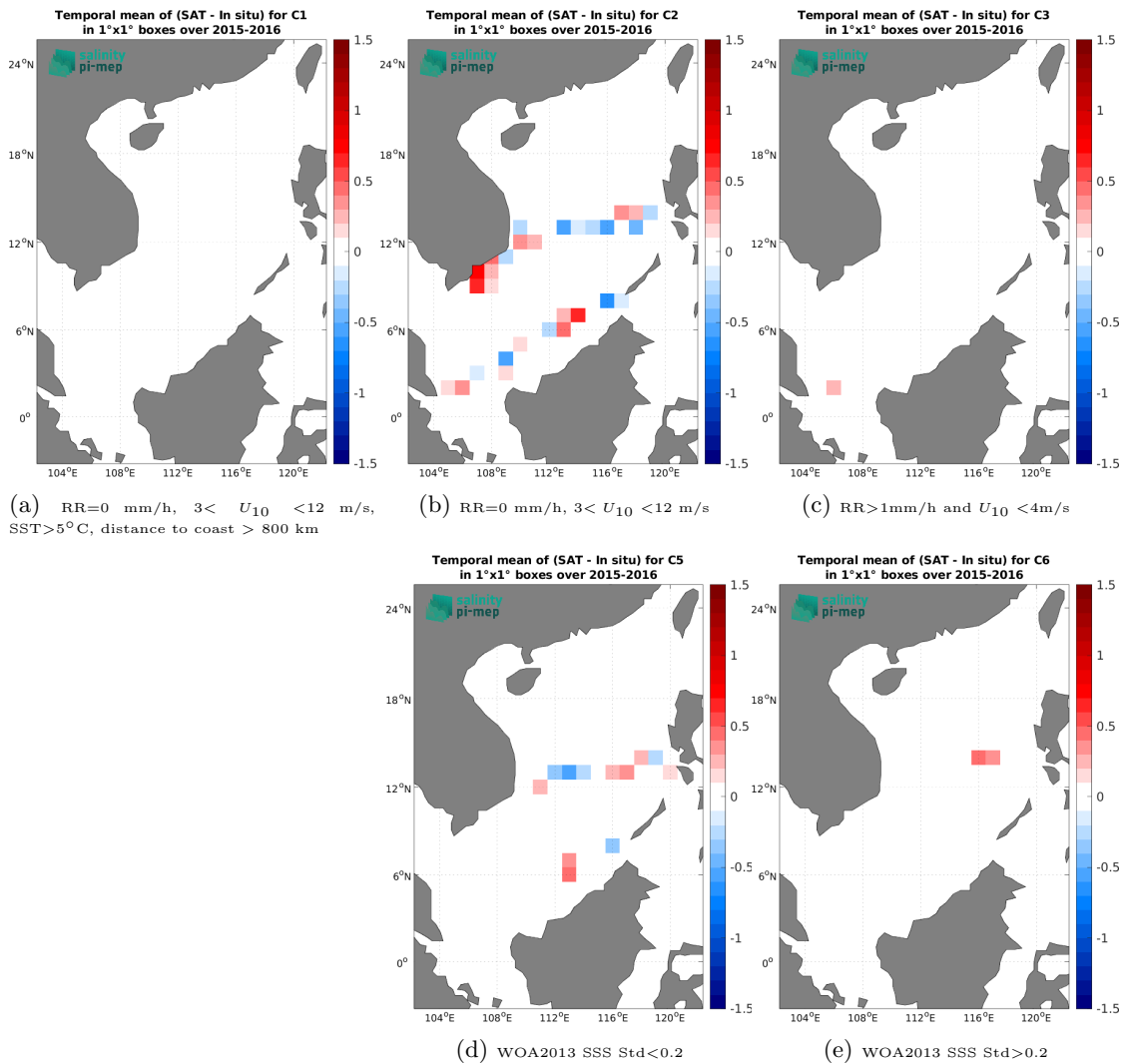
Figure 14: Temporal mean gridded over spatial boxes of size 1^\circ \times 1^\circ of \Delta SSS (SMOS SSS L3 v335 - 10 Days - 25 km (CATDS-CPDC) - TSG (SAMOS)) for 5 different subdatasets corresponding to:RR=0 mm/h, 3 < U_{10} < 12 m/s, SST>5°C, distance to coast > 800 km (a), RR=0 mm/h, 3 < U_{10} < 12 m/s (b), RR>1mm/h and U_{10} < 4 m/s (c), WOA2013 SSS Std<0.2 (d), WOA2013 SSS Std>0.2 (e).
