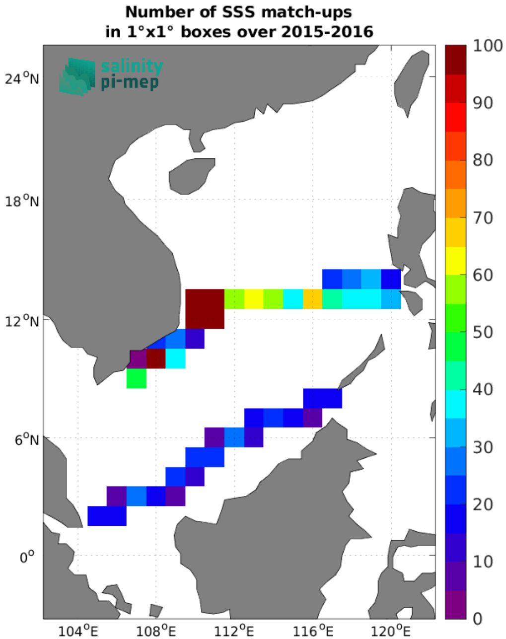
Figure 5: Number of SSS match-ups between TSG (SAMOS) SSS and the SMOS SSS L3 v335 - 10 Days - 25 km (CATDS-CPDC) SSS product for the South China Sea Pi-MEP region over 1°x1° boxes and for the full satellite product period.
