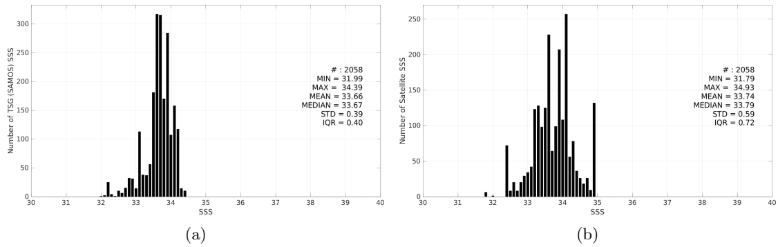
Figure 3: Histograms of SSS from TSG (SAMOS) (a) and SMOS SSS L3 v335 - 10 Days - 25 km (CATDS-CPDC) (b) considering all match-up pairs per bins of 0.1 over the South China Sea Pi-MEP region and for the full satellite product period.
