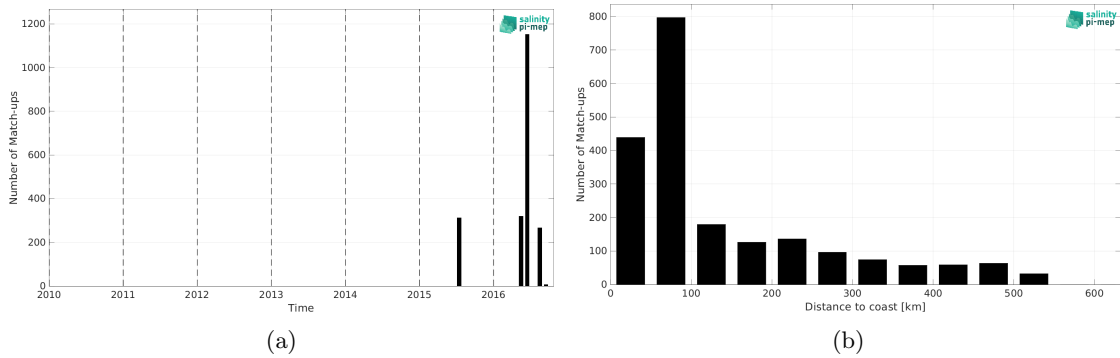
Figure 2: Number of match-ups between TSG (SAMOS) and SMOS SSS L3 v335 - 10 Days - 25 km (CATDS-CPDC) SSS as a function of time (a) and as function of the distance to coast (b) over the South China Sea Pi-MEP region and for the full satellite product period.
