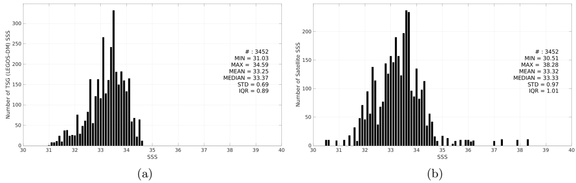
Figure 3: Histograms of SSS from TSG (LEGOS-DM) (a) and SMOS SSS L3 v335 - 10 Days - 25 km (CATDS-CPDC) (b) considering all match-up pairs per bins of 0.1 over the South China Sea Pi-MEP region and for the full satellite product period.
