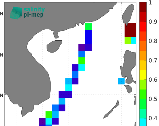
Temporal STD of (Sat - TSG (LEGOS-DM)) in 1°x1° boxes over 2010-2021
