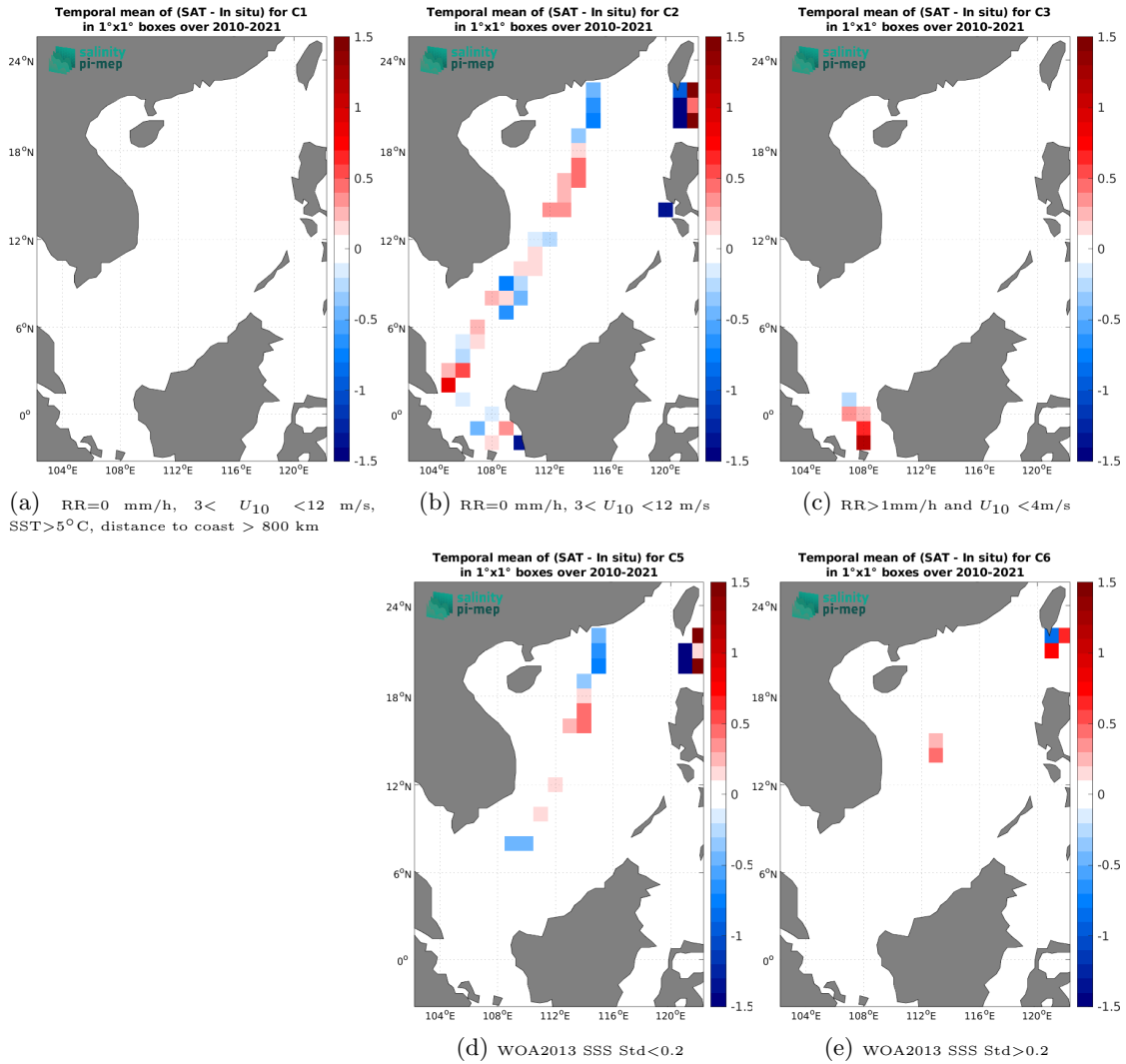
Figure 14: Temporal mean gridded over spatial boxes of size 1^\circ \times 1^\circ of \Delta SSS (SMOS SSS L3 v335 - 10 Days - 25 km (CATDS-CPDC) - TSG (LEGOS-DM)) for 5 different subdatasets corresponding to:RR=0 mm/h, 3 < U_{10} < 12 m/s, SST>5°C, distance to coast > 800 km (a), RR=0 mm/h, 3 < U_{10} < 12 m/s (b), RR>1mm/h and U_{10} < 4 m/s (c), WOA2013 SSS Std<0.2 (d), WOA2013 SSS Std>0.2 (e).
