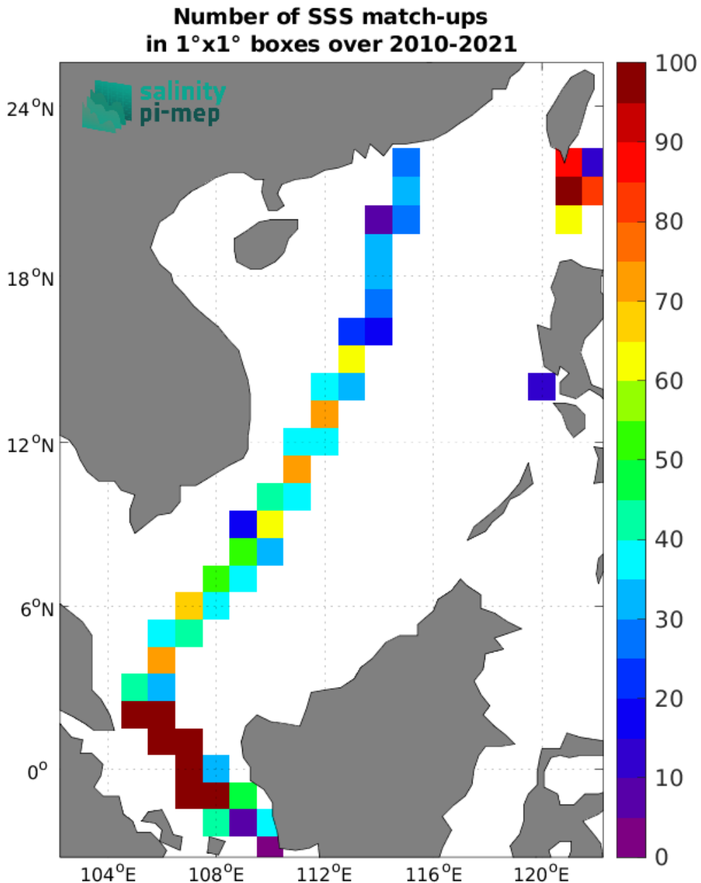
Figure 5: Number of SSS match-ups between TSG (LEGOS-DM) SSS and the SMOS SSS L3 v335 - 10 Days - 25 km (CATDS-CPDC) SSS product for the South China Sea Pi-MEP region over 1°×1° boxes and for the full satellite product period.
