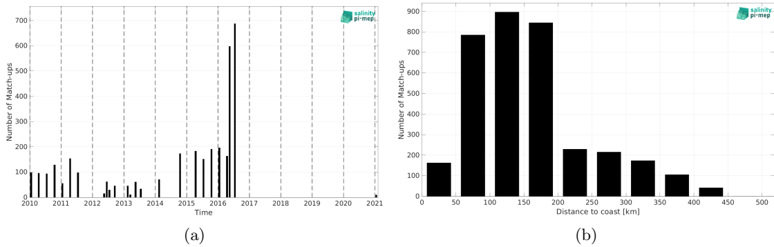
Figure 2: Number of match-ups between TSG (LEGOS-DM) and SMOS SSS L3 v335 - 10 Days - 25 km (CATDS-CPDC) SSS as a function of time (a) and as function of the distance to coast (b) over the South China Sea Pi-MEP region and for the full satellite product period.
