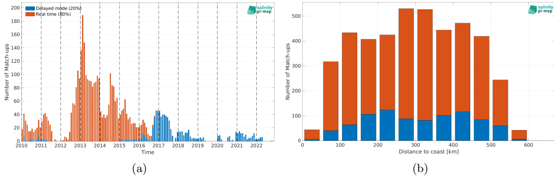
Figure 1: Number of match-ups between Argo and SMOS SSS L3 v335 - 10 Days - 25 km (CATDS-CPDC) SSS as a function of time (a) and as function of the distance to coast (b) over the South China Sea Pi-MEP region and for the full satellite product period.
