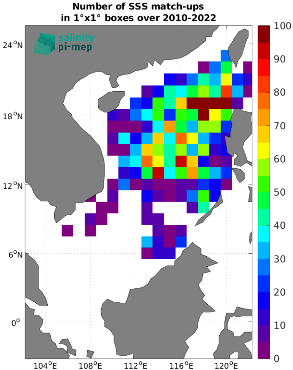
Figure 4: Number of SSS match-ups between Argo SSS and the SMOS SSS L3 v335 - 10 Days - 25 km (CATDS-CPDC) SSS product for the South China Sea Pi-MEP region over 1^\circ \times 1^\circ boxes and for the full satellite product period.
