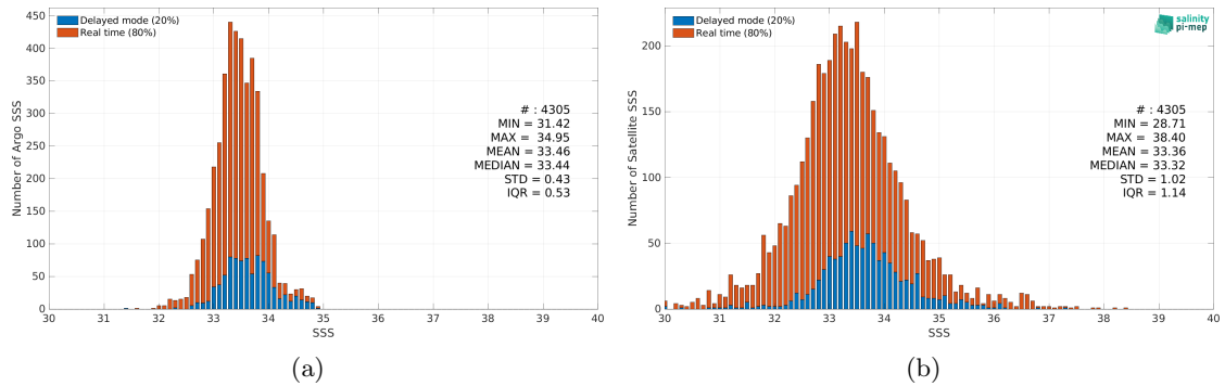
Figure 2: Histograms of SSS from Argo (a) and SMOS SSS L3 v335 - 10 Days - 25 km (CATDS-CPDC) (b) considering all match-up pairs per bins of 0.1 over the South China Sea Pi-MEP region and for the full satellite product period.
