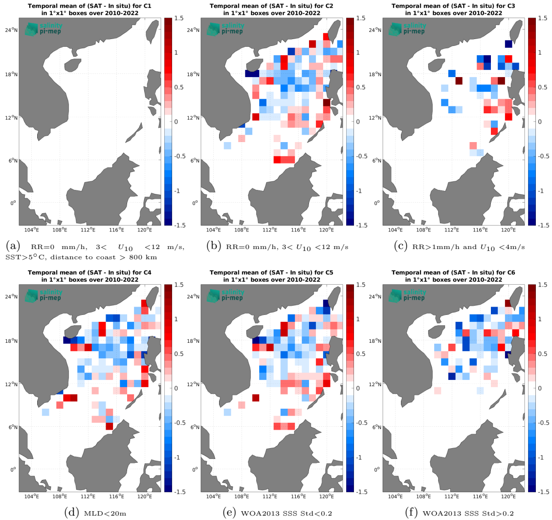
Figure 12: Temporal mean gridded over spatial boxes of size 1^\circ \times 1^\circ of \Delta SSS (SMOS SSS L3 v335 - 10 Days - 25 km (CATDS-CPDC) - Argo) for 6 different subdatasets corresponding to:RR=0 mm/h, 3 < U_{10} < 12 m/s, SST>5°C, distance to coast > 800 km (a), RR=0 mm/h, 3 < U_{10} < 12 m/s (b), RR>1mm/h and U_{10} < 4 m/s (c),MLD<20m (d),WOA2013 SSS Std<0.2 (e),WOA2013 SSS Std>0.2 (f).
