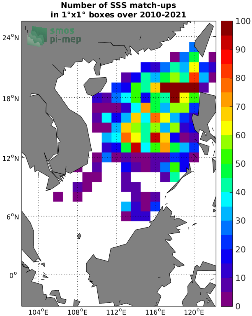
Figure 4: Number of SSS match-ups between Argo SSS and the SMOS SSS L3 v335 - 10 Days - 25 km (CATDS-CPDC) SSS product for the South China Sea Pi-MEP region over 1°x1° boxes and for the full satellite product period.
