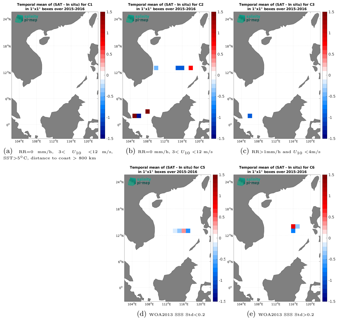
Figure 14: Temporal mean gridded over spatial boxes of size 1^\circ \times 1^\circ of \Delta SSS (SMOS SSS L2Q v333 - 0.25 Deg (CATDS-CPDC) - TSG (SAMOS)) for 5 different subdatasets corresponding to: RR=0 mm/h, 3 < U_{10} < 12 m/s, SST>5°C, distance to coast > 800 km (a), RR=0 mm/h, 3 < U_{10} < 12 m/s (b), RR>1mm/h and U_{10} < 4 m/s (c), WOA2013 SSS Std<0.2 (d), WOA2013 SSS Std>0.2 (e).
