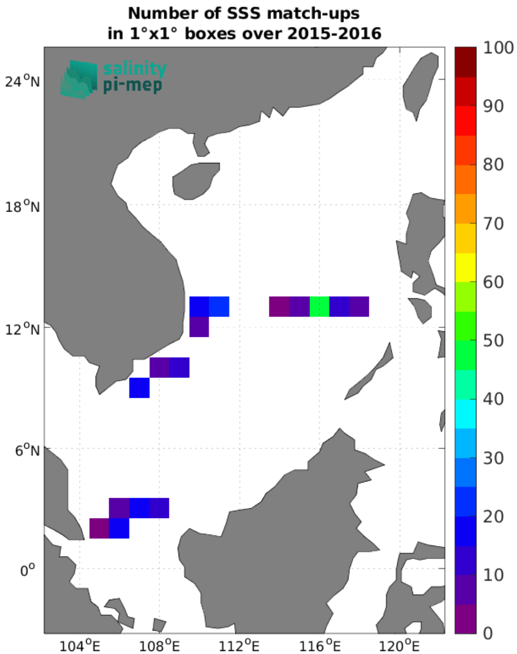
Figure 5: Number of SSS match-ups between TSG (SAMOS) SSS and the SMOS SSS L2Q v333 - 0.25 Deg (CATDS-CPDC) SSS product for the South China Sea Pi-MEP region over 1°x1° boxes and for the full satellite product period.
