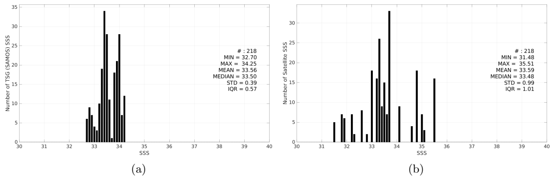
Figure 3: Histograms of SSS from TSG (SAMOS) (a) and SMOS SSS L2Q v333 - 0.25 Deg (CATDS-CPDC) (b) considering all match-up pairs per bins of 0.1 over the South China Sea Pi-MEP region and for the full satellite product period.
