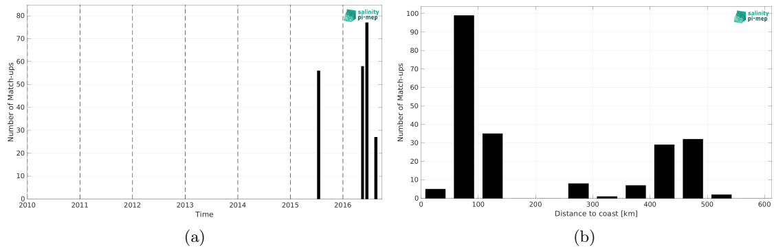
Figure 2: Number of match-ups between TSG (SAMOS) and SMOS SSS L2Q v333 - 0.25 Deg (CATDS-CPDC) SSS as a function of time (a) and as function of the distance to coast (b) over the South China Sea Pi-MEP region and for the full satellite product period.
