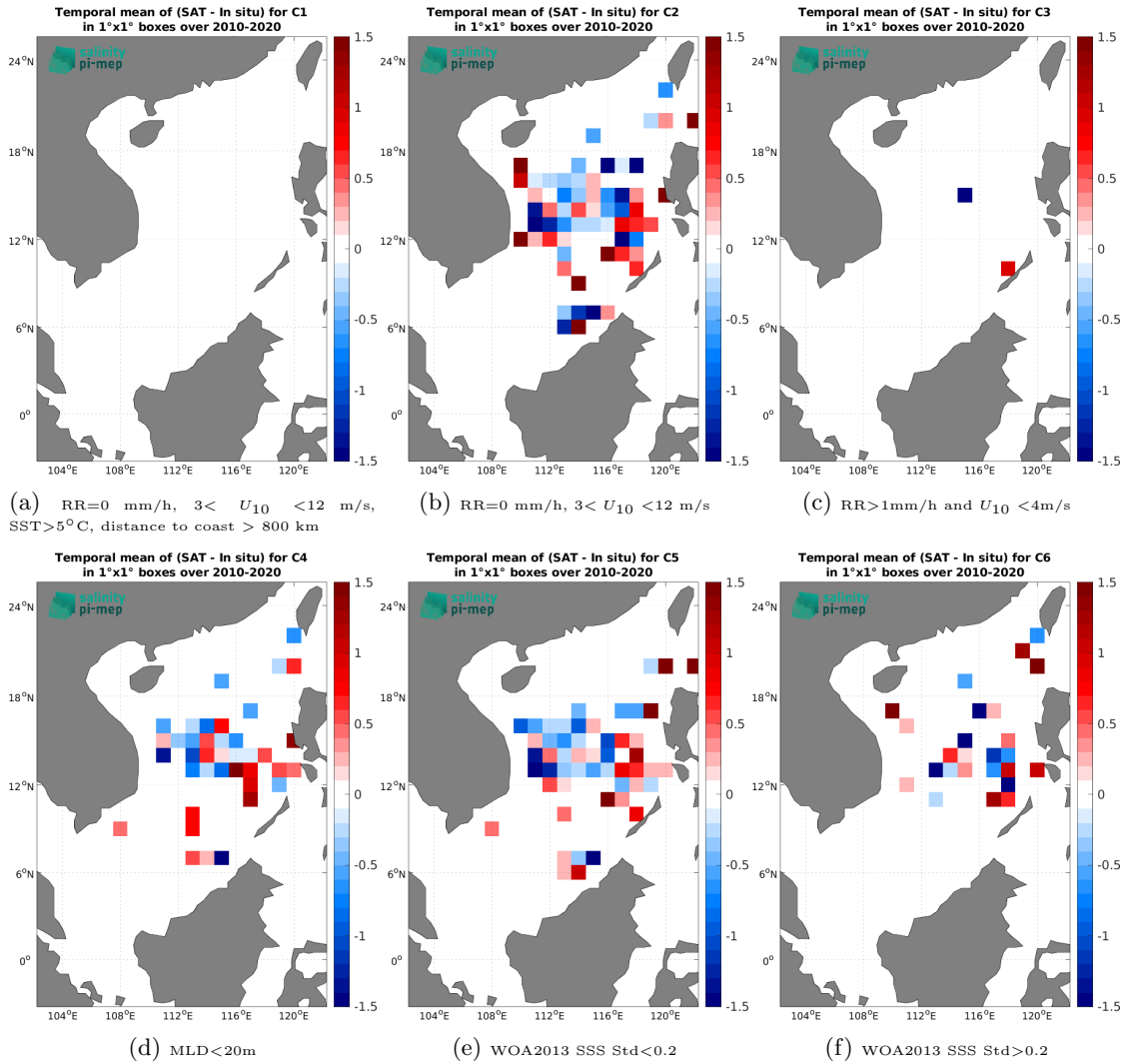
Figure 14: Temporal mean gridded over spatial boxes of size 1^\circ \times 1^\circ of \Delta SSS (SMOS SSS L2Q v333 - 0.25 Deg (CATDS-CPDC) - Argo) for 6 different subdatasets corresponding to: RR=0 mm/h, 3 < U_{10} < 12 m/s, SST>5°C, distance to coast > 800 km (a), RR=0 mm/h, 3 < U_{10} < 12 m/s (b), RR>1mm/h and U_{10} < 4 m/s (c),MLD<20m (d),WOA2013 SSS Std<0.2 (e),WOA2013 SSS Std>0.2 (f).
