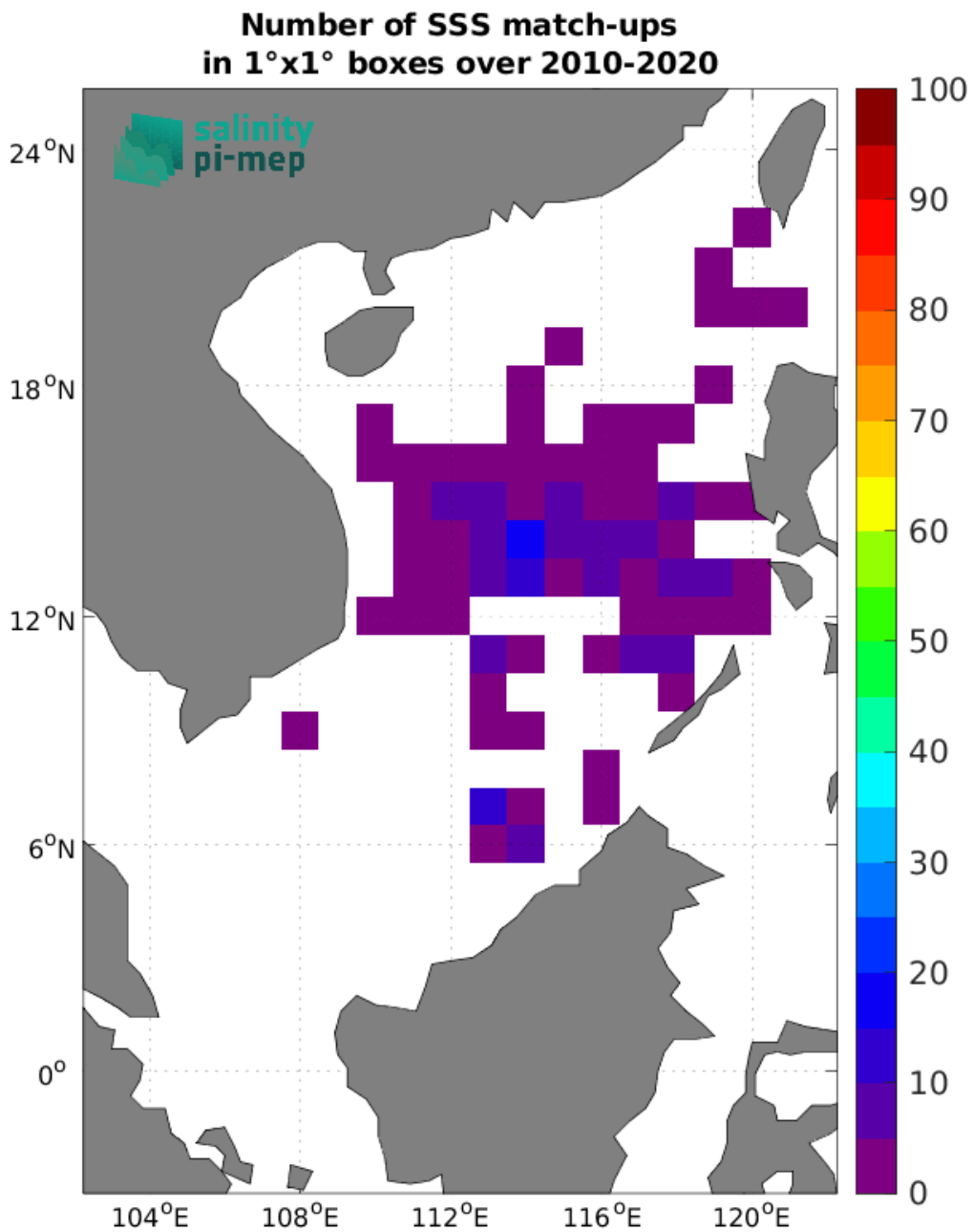
Figure 5: Number of SSS match-ups between Argo SSS and the SMOS SSS L2Q v333 - 0.25 Deg (CATDS-CPDC) SSS product for the South China Sea Pi-MEP region over 1^{\circ} \times 1^{\circ} boxes and for the full satellite product period.
