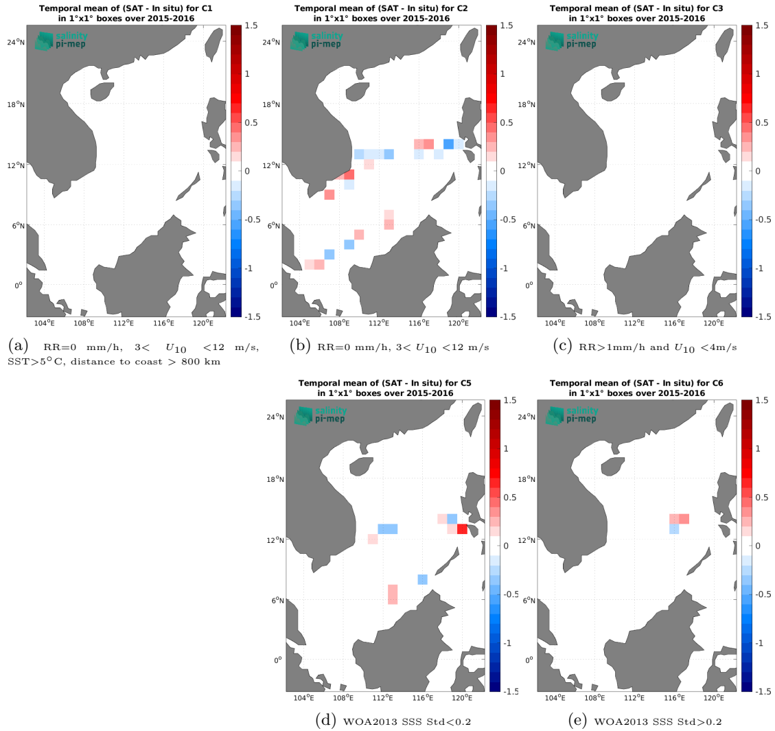
Figure 12: Temporal mean gridded over spatial boxes of size 1^\circ \times 1^\circ of \Delta\text{SSS} (SMOS SSS L3 v332 - 9 Days (CATDS-CPDC) - TSG (SAMOS)) for 5 different subdatasets corresponding to: RR=0 mm/h, 3 < U_{10} < 12 m/s, SST > 5^\circ\text{C} , distance to coast > 800 km (a), RR=0 mm/h, 3 < U_{10} < 12 m/s (b), RR > 1 mm/h and U_{10} < 4 m/s (c), WOA2013 SSS Std < 0.2 (d), WOA2013 SSS Std > 0.2 (e).
