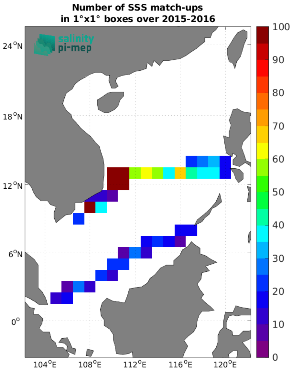
Figure 4: Number of SSS match-ups between TSG (SAMOS) SSS and the SMOS SSS L3 v332 - 9 Days (CATDS-CPDC) SSS product for the South China Sea Pi-MEP region over 1^\circ \times 1^\circ boxes and for the full satellite product period.
